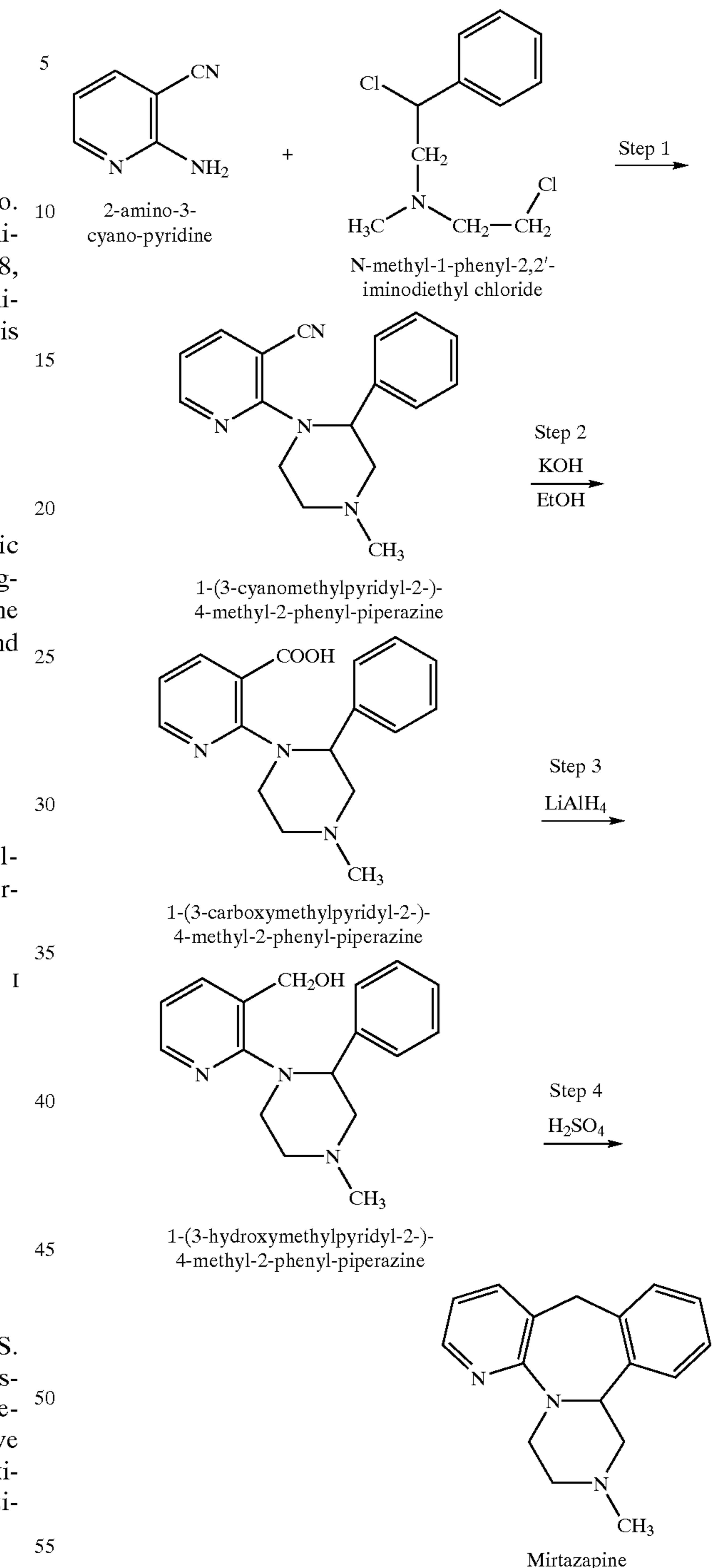
Scheme 1
