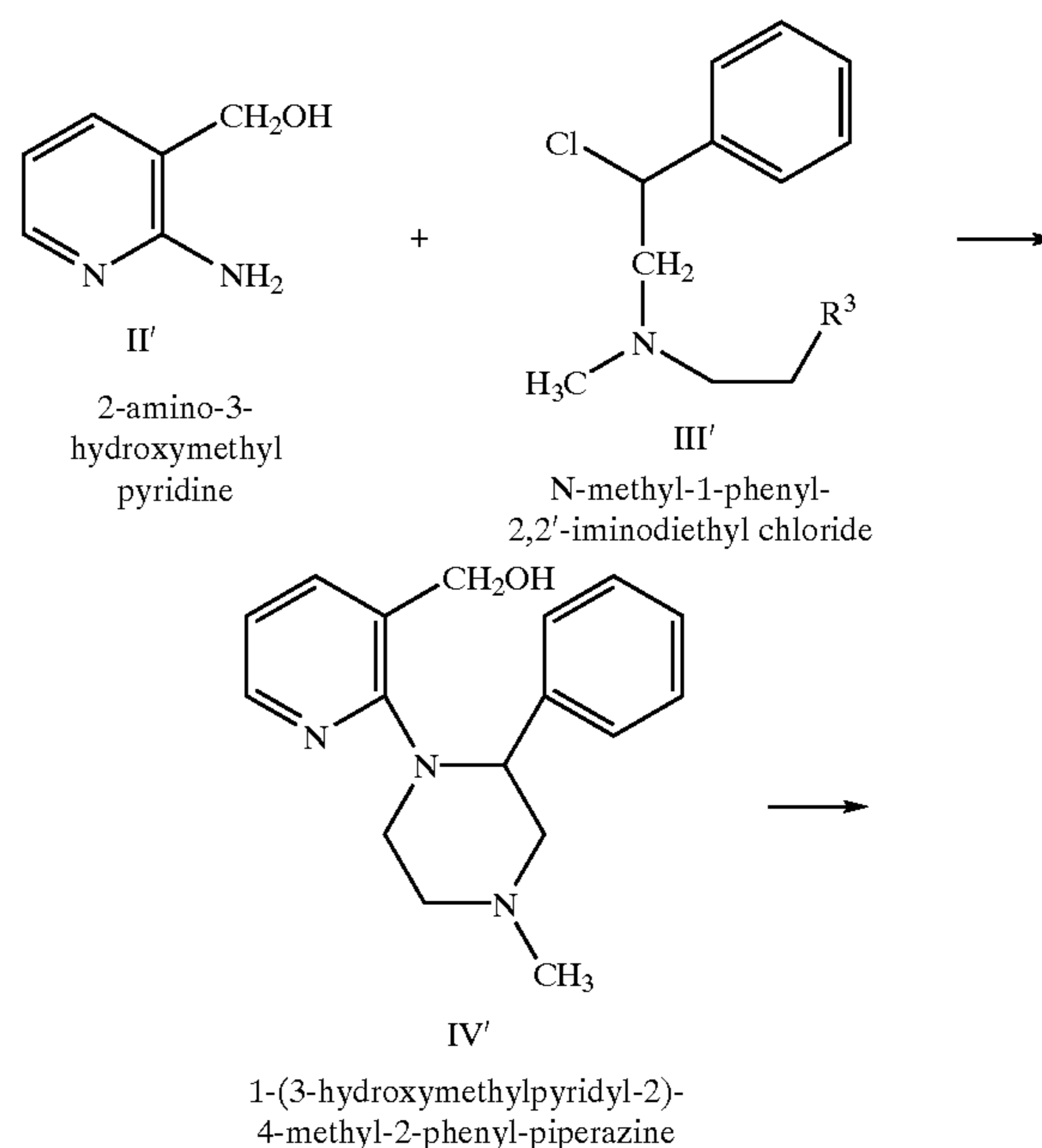
Scheme 3
