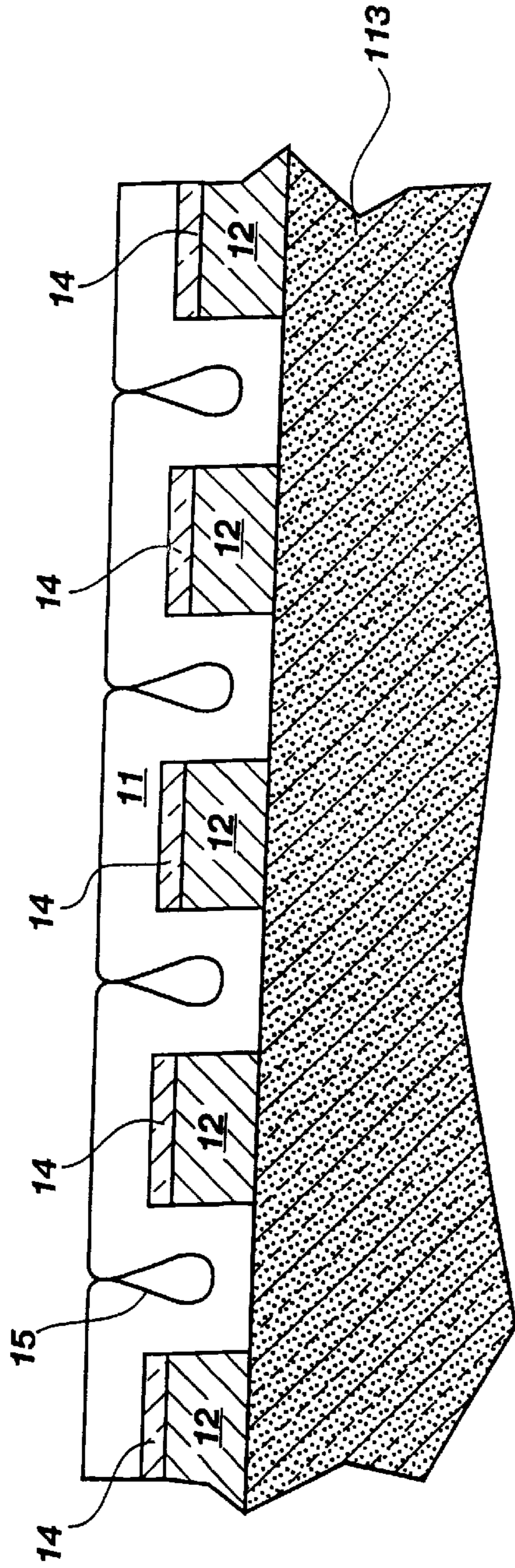
Fig. 1 (PRIOR ART)
