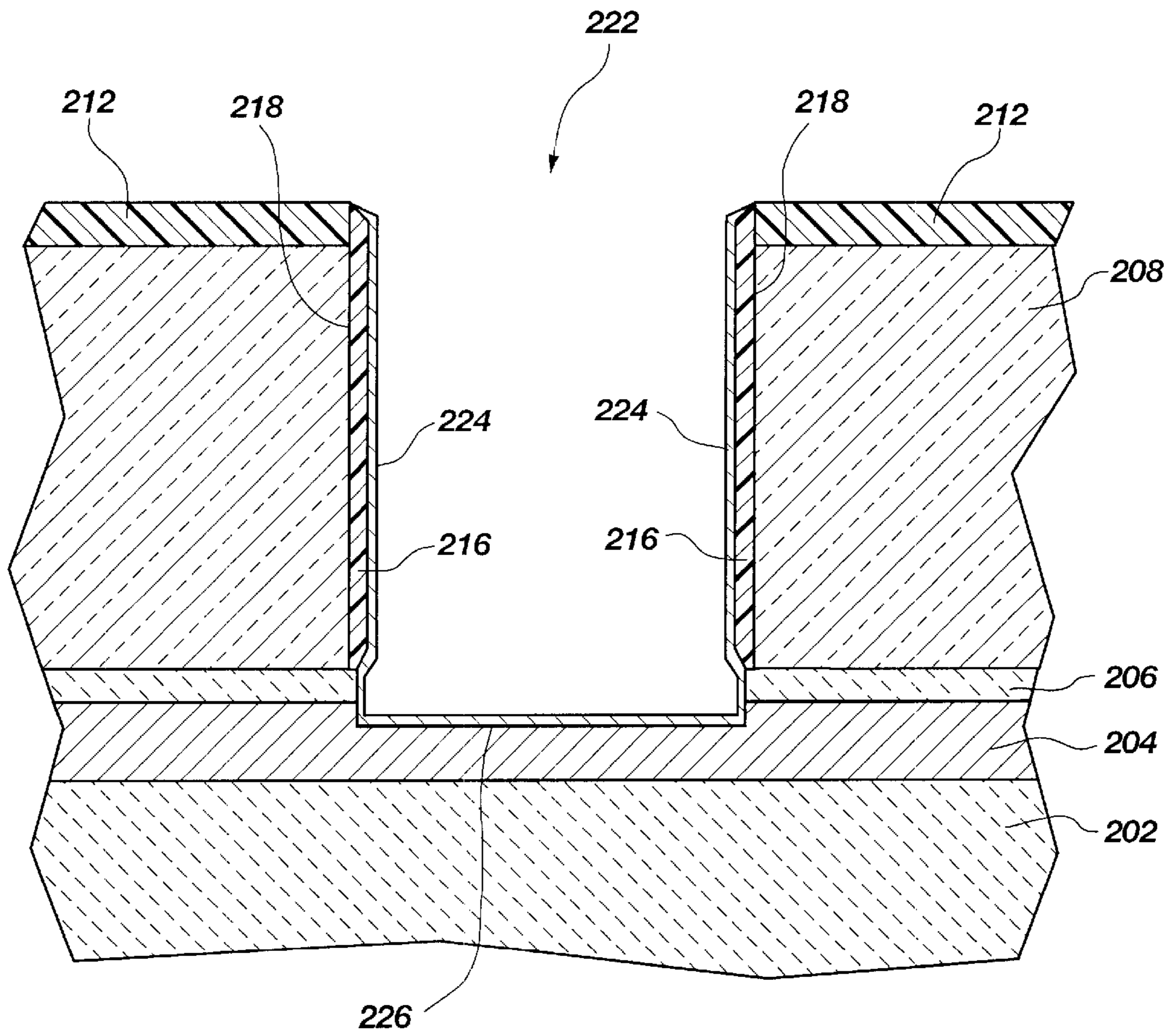
Fig. 14 (PRIOR ART)
