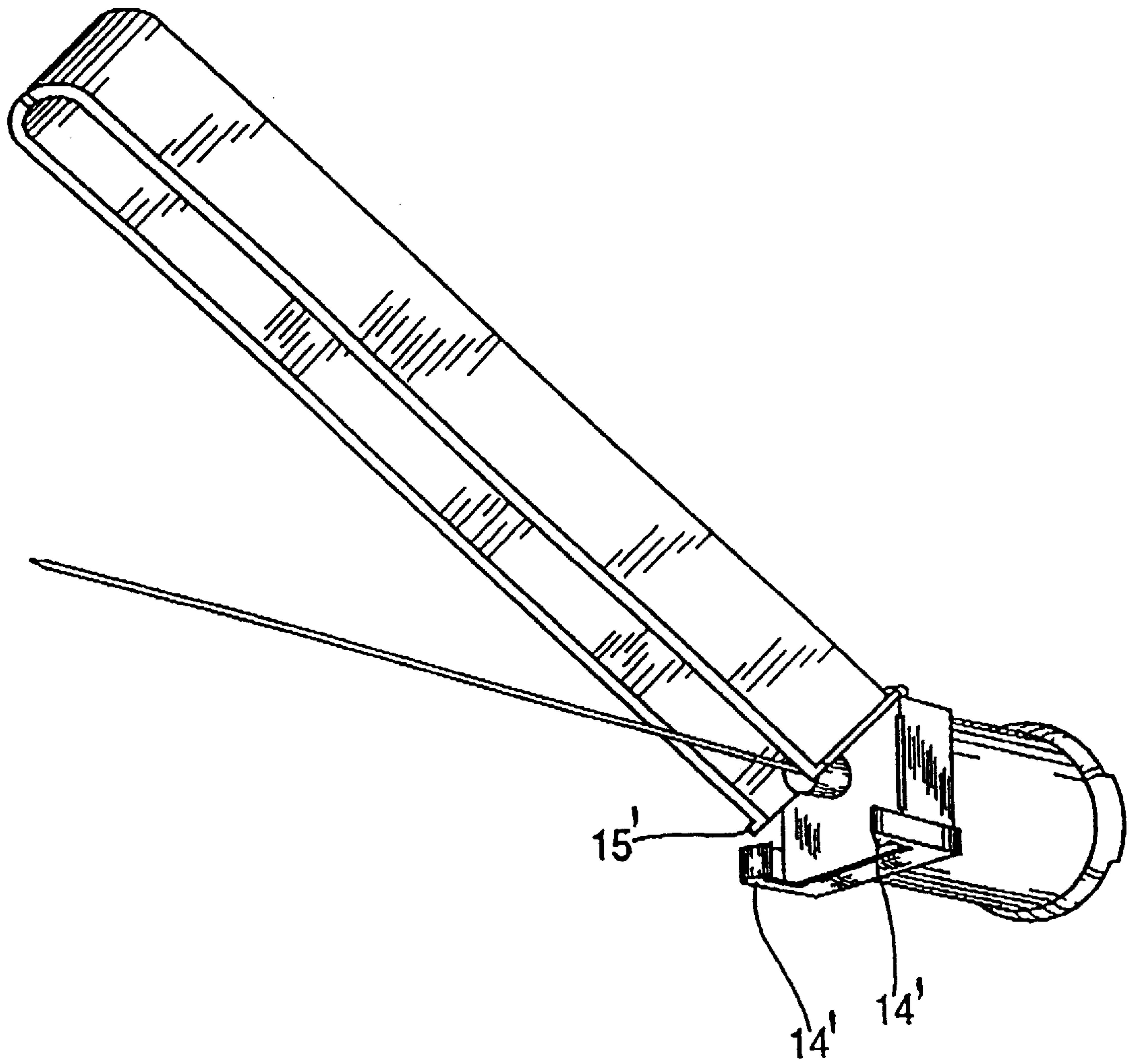
FIG. 4 PRIOR ART
