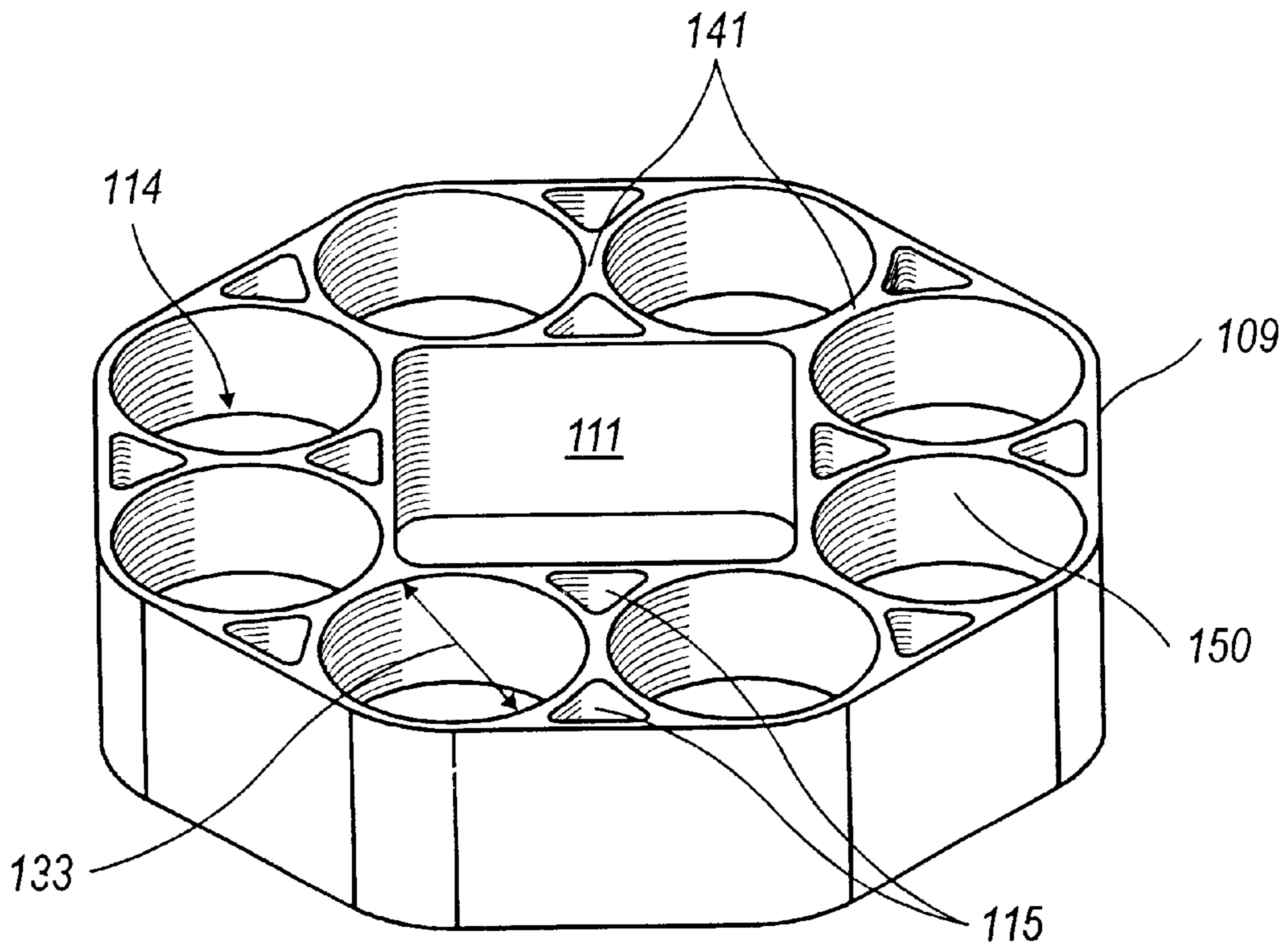
Bottom View FIG. 13a
