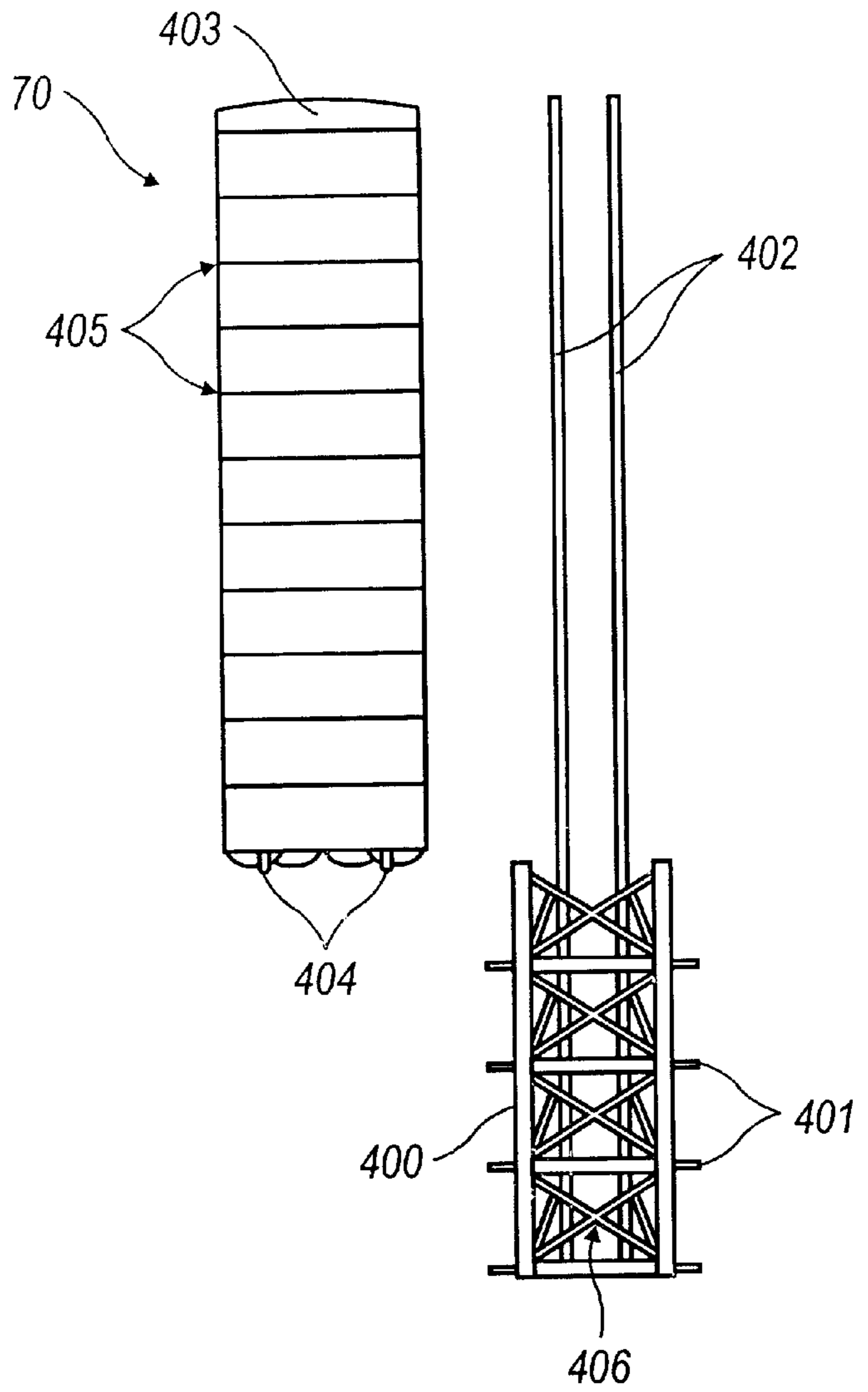
Truss Removed FIG. 4b
