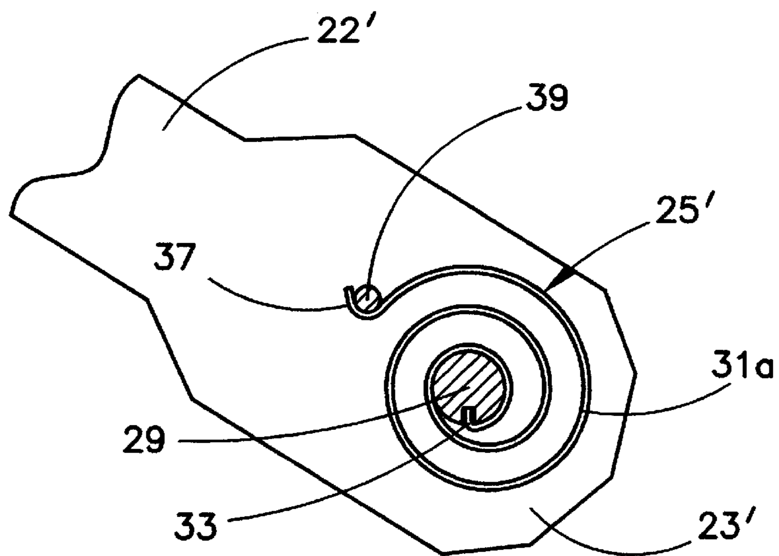
FIG. 3 (PRIOR ART)
