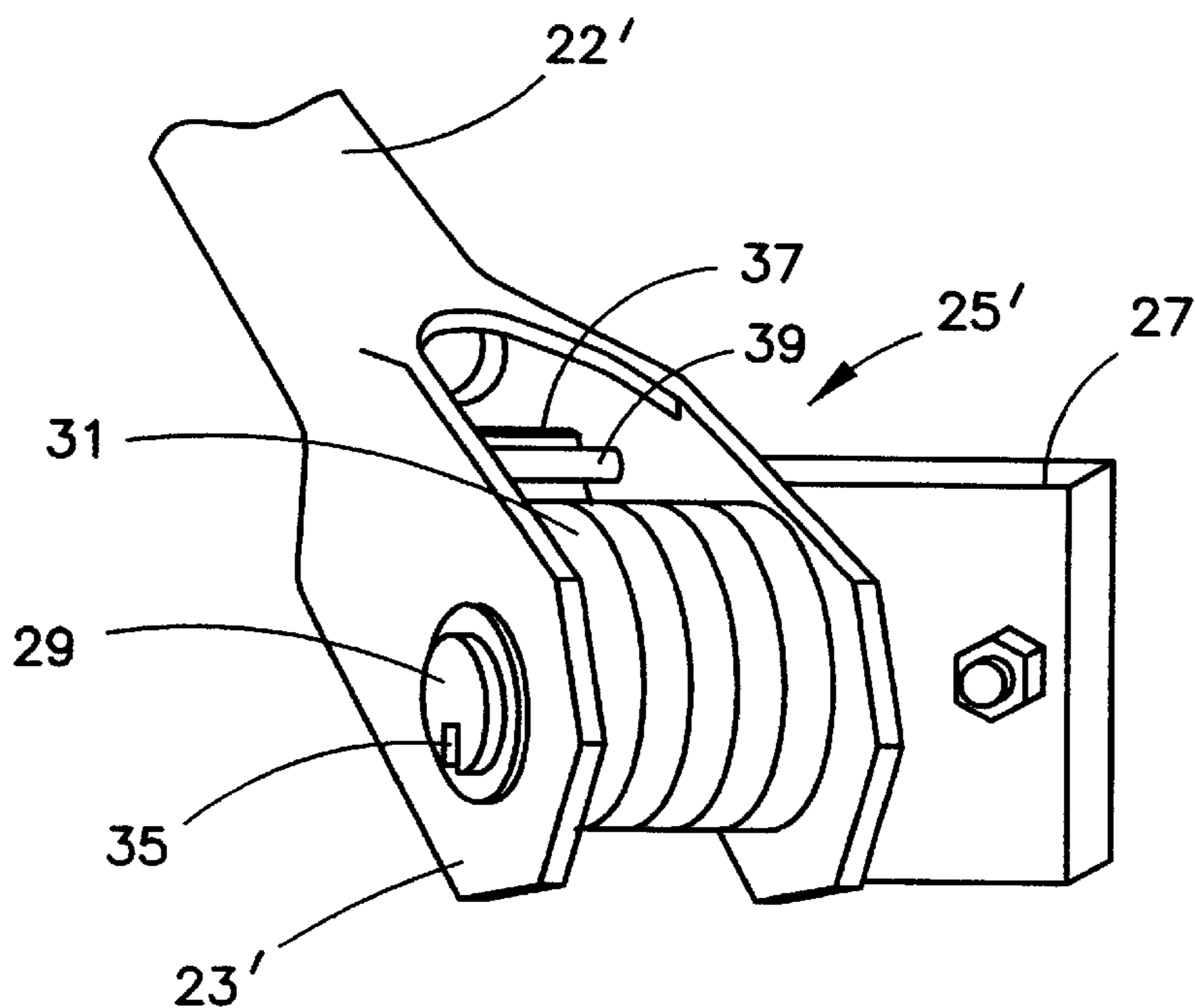
FIG. 2 (PRIOR ART)
