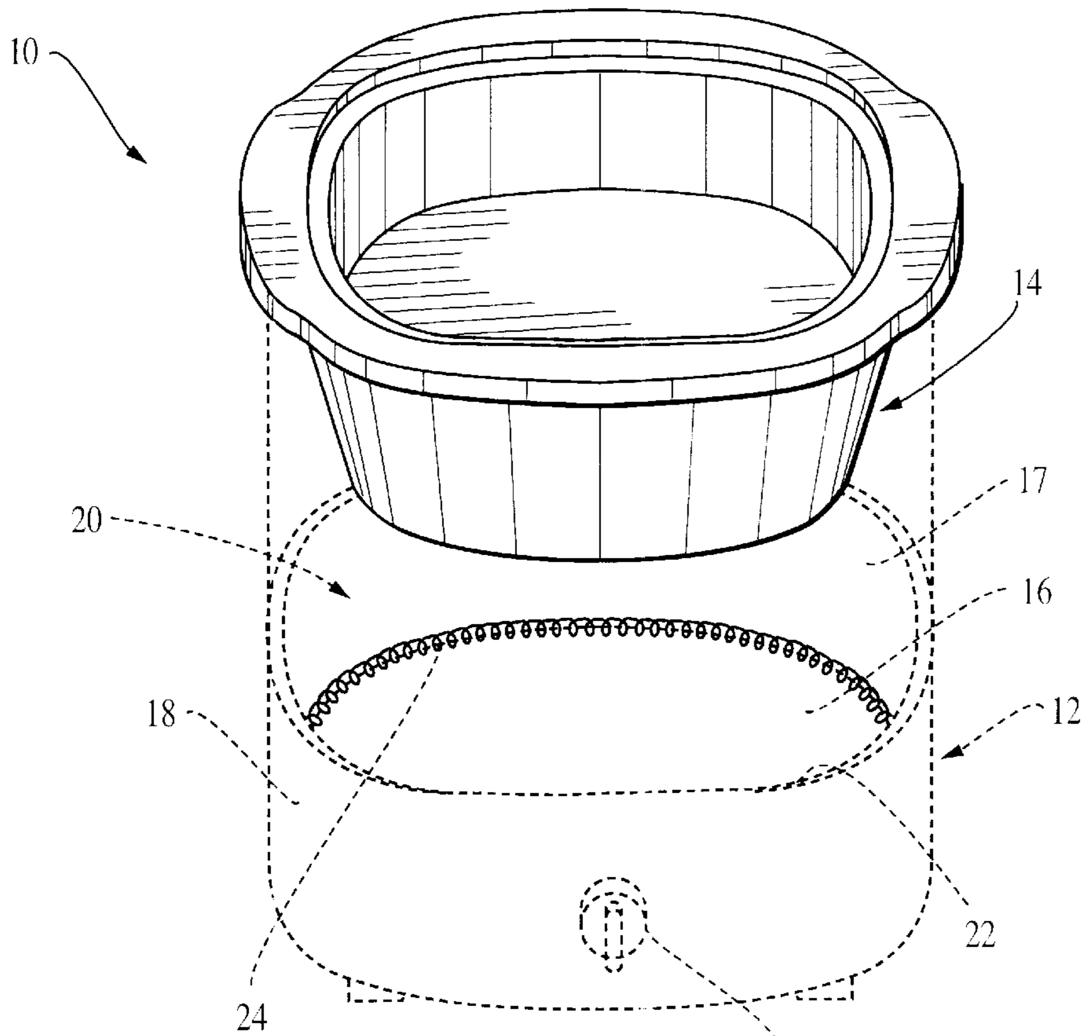
FIG. 1 PRIOR ART
