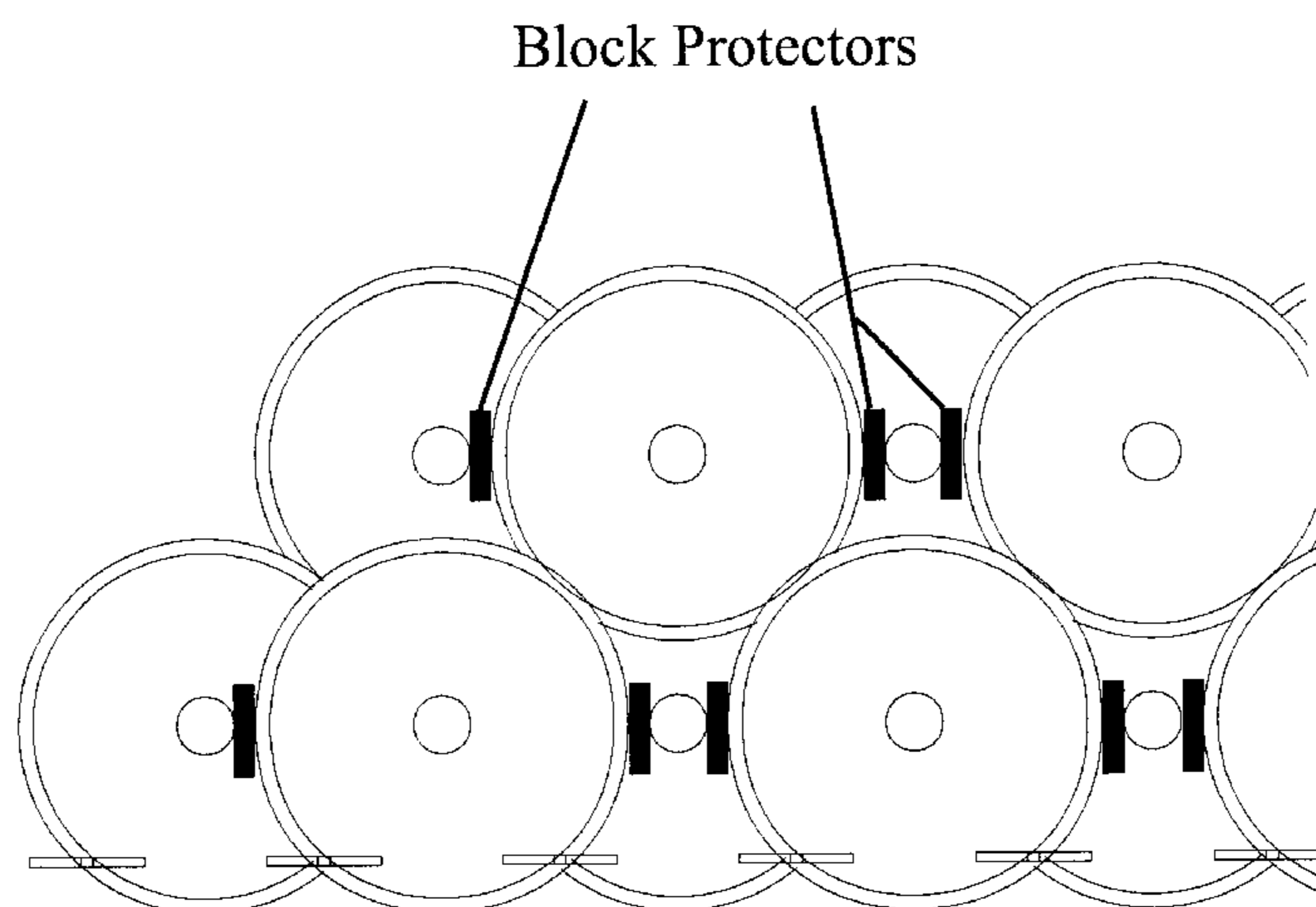
Figure 12 Block shaped protectors placed between roller bearings and adjacent wheel flanges.
