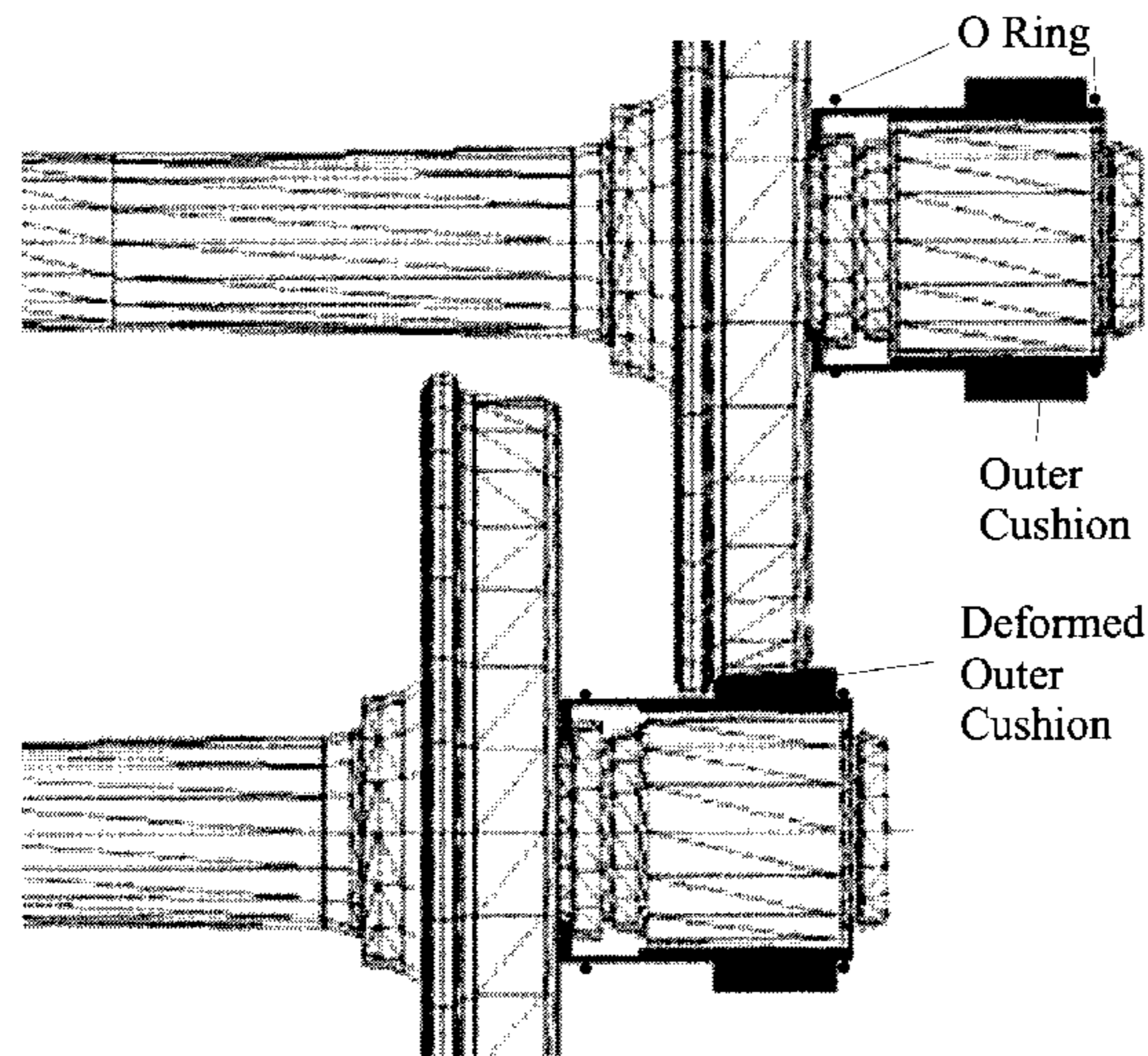
Figure 16 Deformation of roller bearing protector's outer cushion and removal any gap between roller bearing and adjacent wheel. Force of adjacent wheel is transmitted to the roller bearing over a greater area as compared to a point load from the wheel flange (when no protectors are used).
