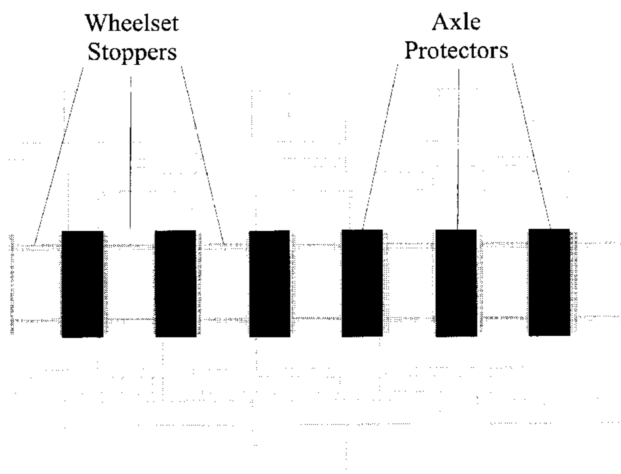
Figure 33 Top view. Wheelset fitted with proper sized axle protectors are immobilized between the wheelset stoppers. Size of axle protectors is large enough to eliminate any gaps between the wheelset axle and the wheelset stoppers.
