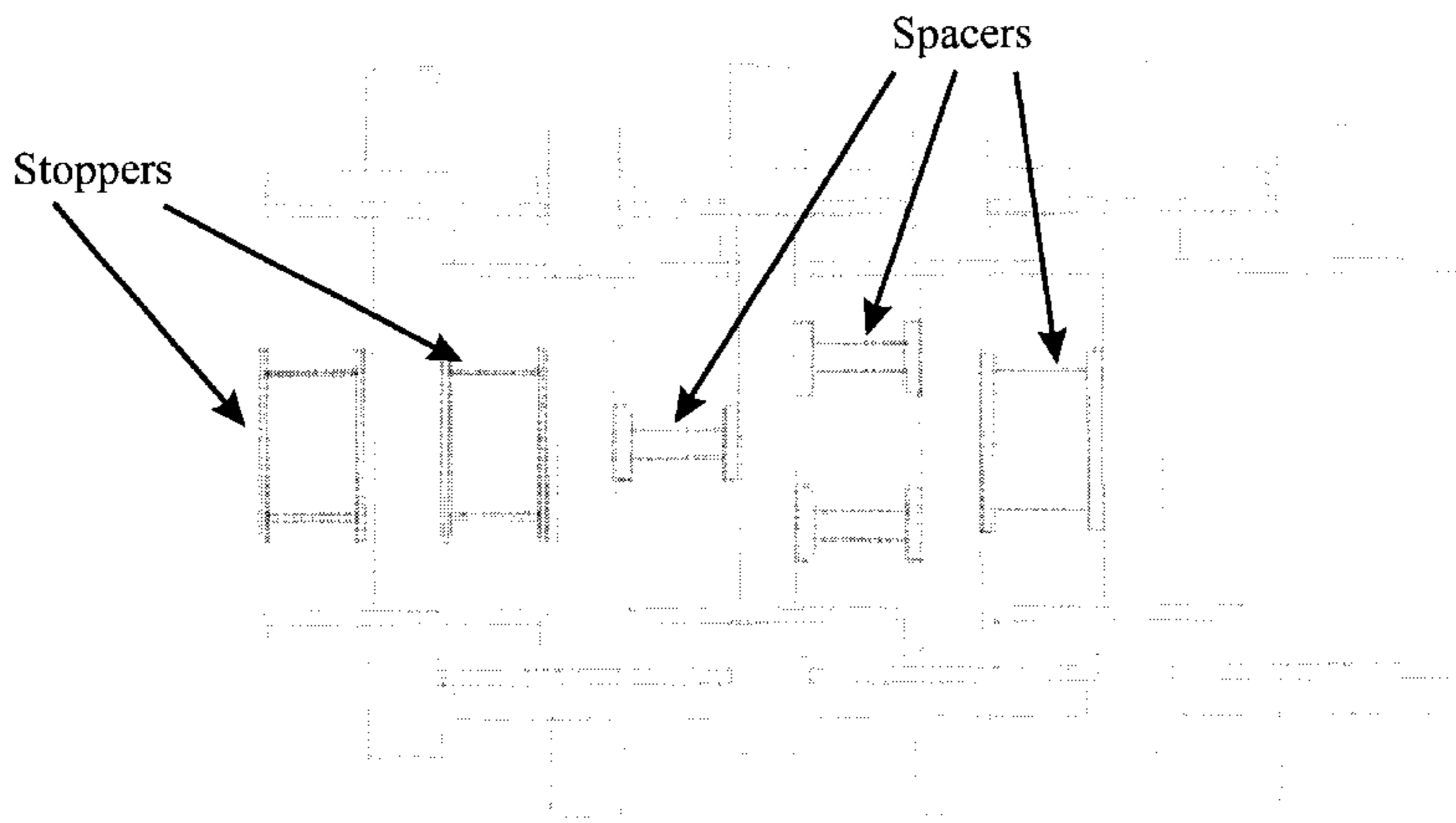
Figure 38 A single spacer centered could be used between a pair of adjacent axles to restrain the wheelsets. Using two spacers between pairs of adjacent axles increases stability. Increased stability could also be obtained if the spacer is wider as shown above.
