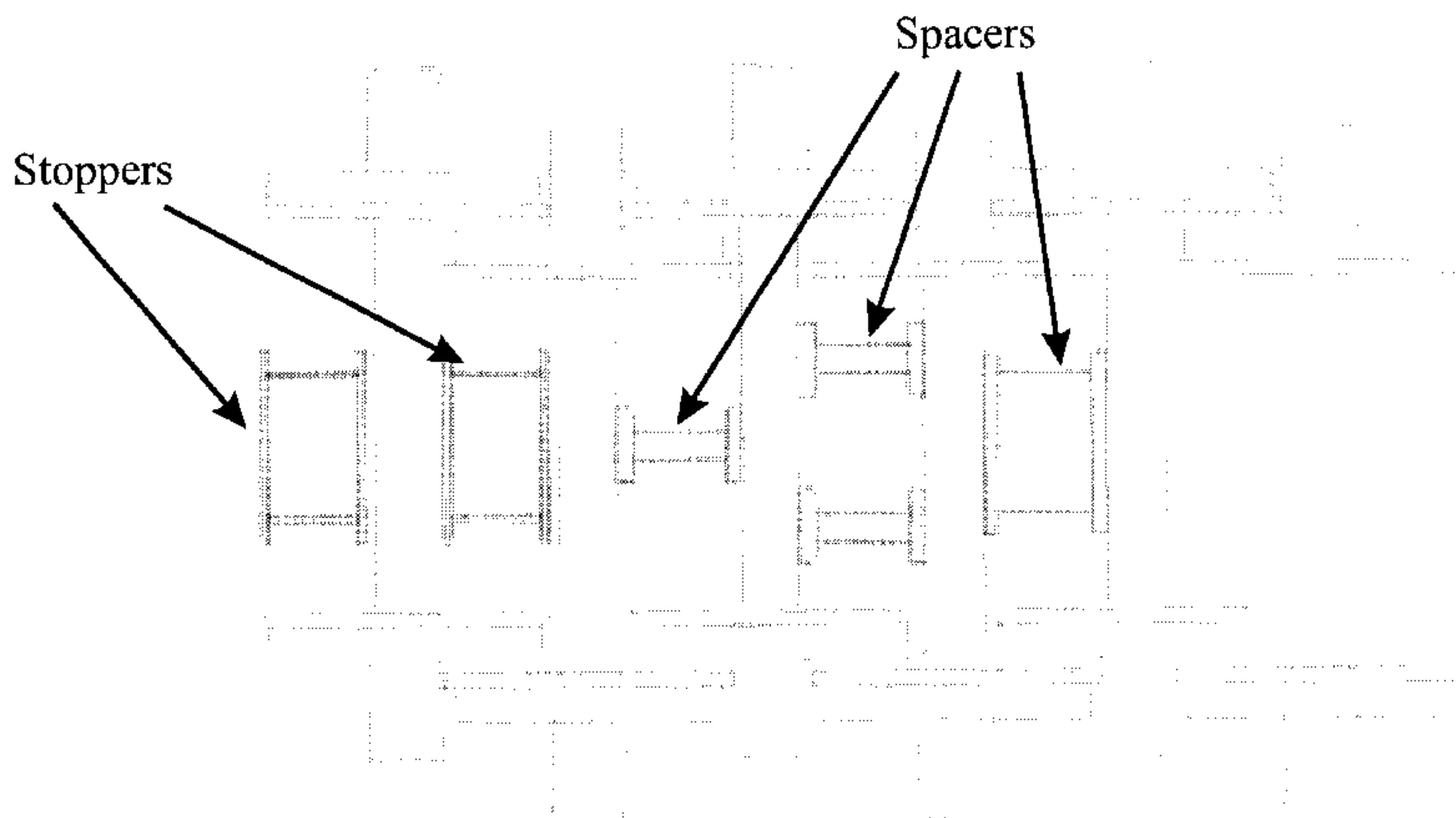
Figure 38 A single spacer centered could be used between a pair of adjacent axles to restrain the wheelsets. Using two spacers between pairs of adjacent axles increases stability. Increased stability could also be obtained if the spacer is wider as shown above.
