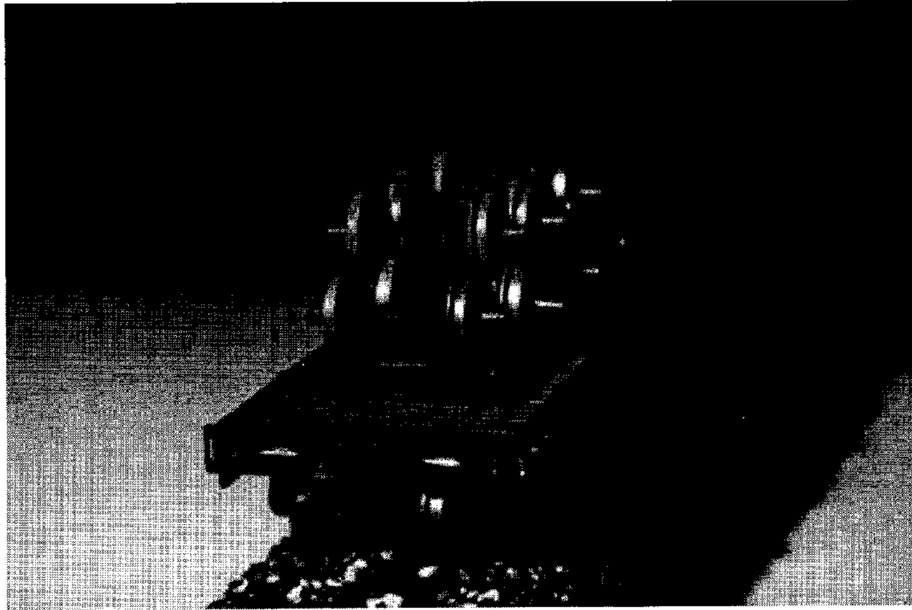
Figure 53 Axle protectors for the axles are required to prevent single point contact with the axle and the wheelset stoppers. Protector also prevents movement by removing any gaps between axle and wheelset stoppers.
