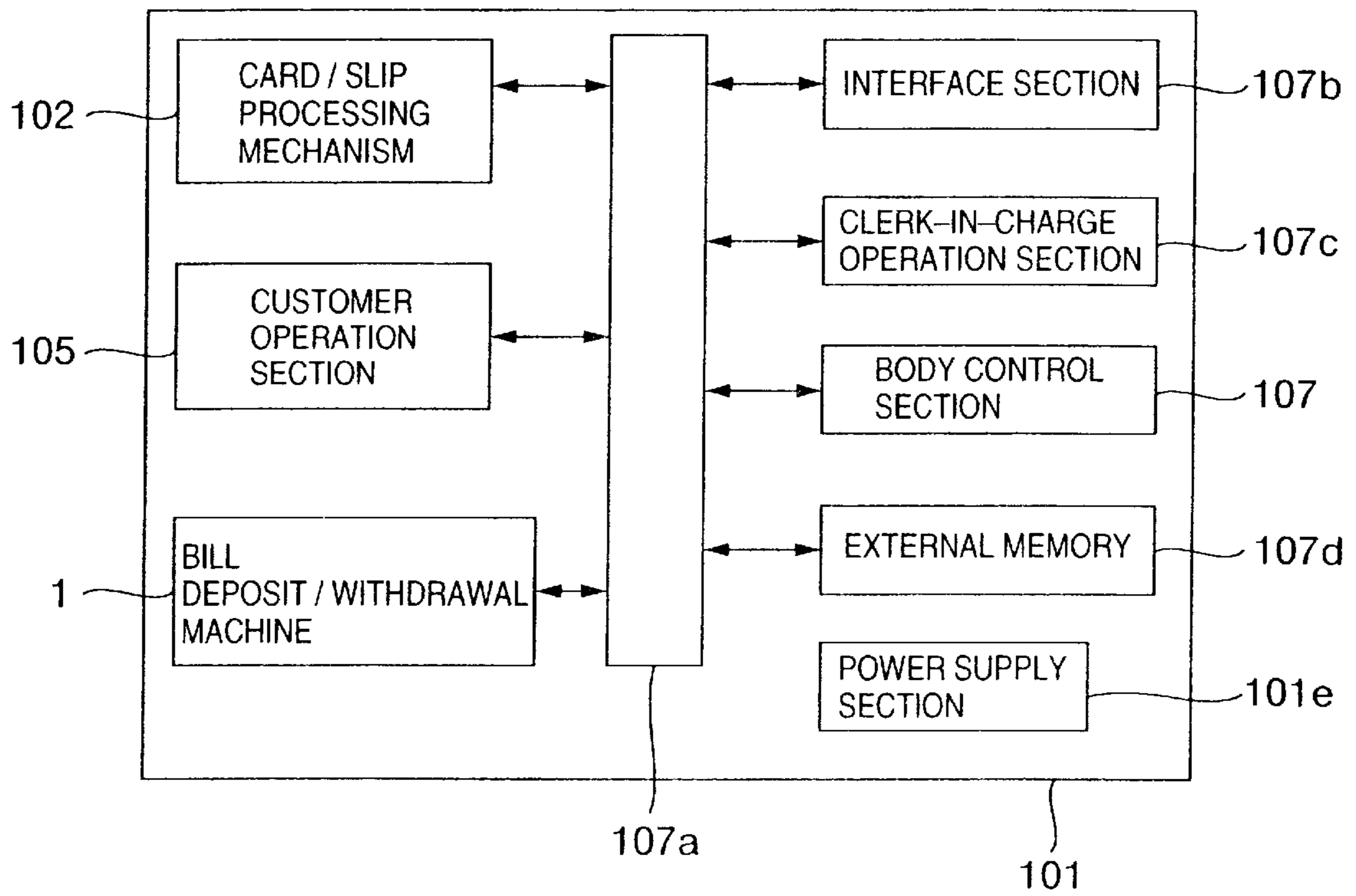
CONTROL BLOCK DIAGRAM OF AUTOMATED TELLER MACHINE 1
