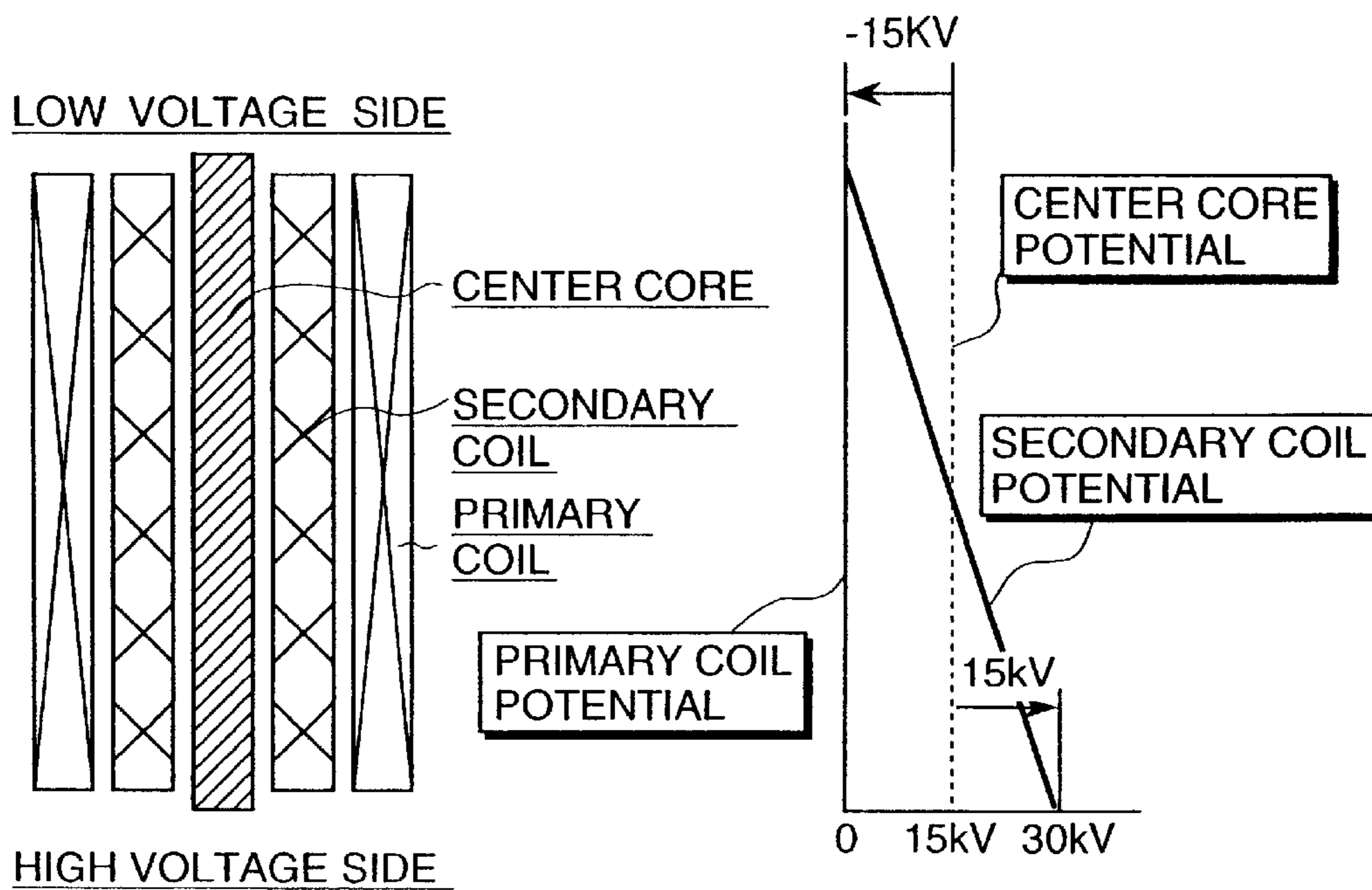
POTENTIALS OF SECONDARY COIL AND CENTER CORE
