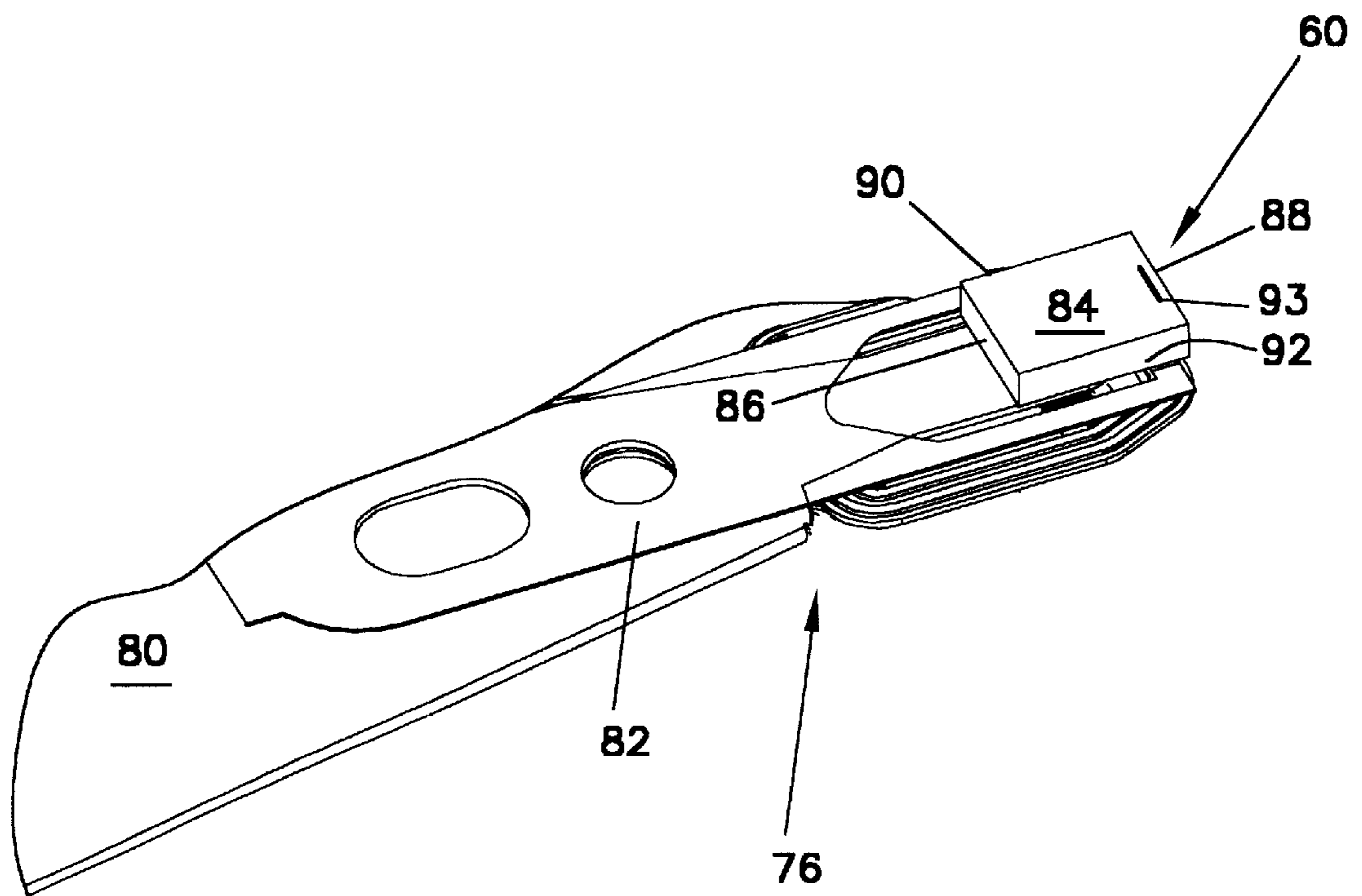
FIG. 3 ( PRIOR ART )
