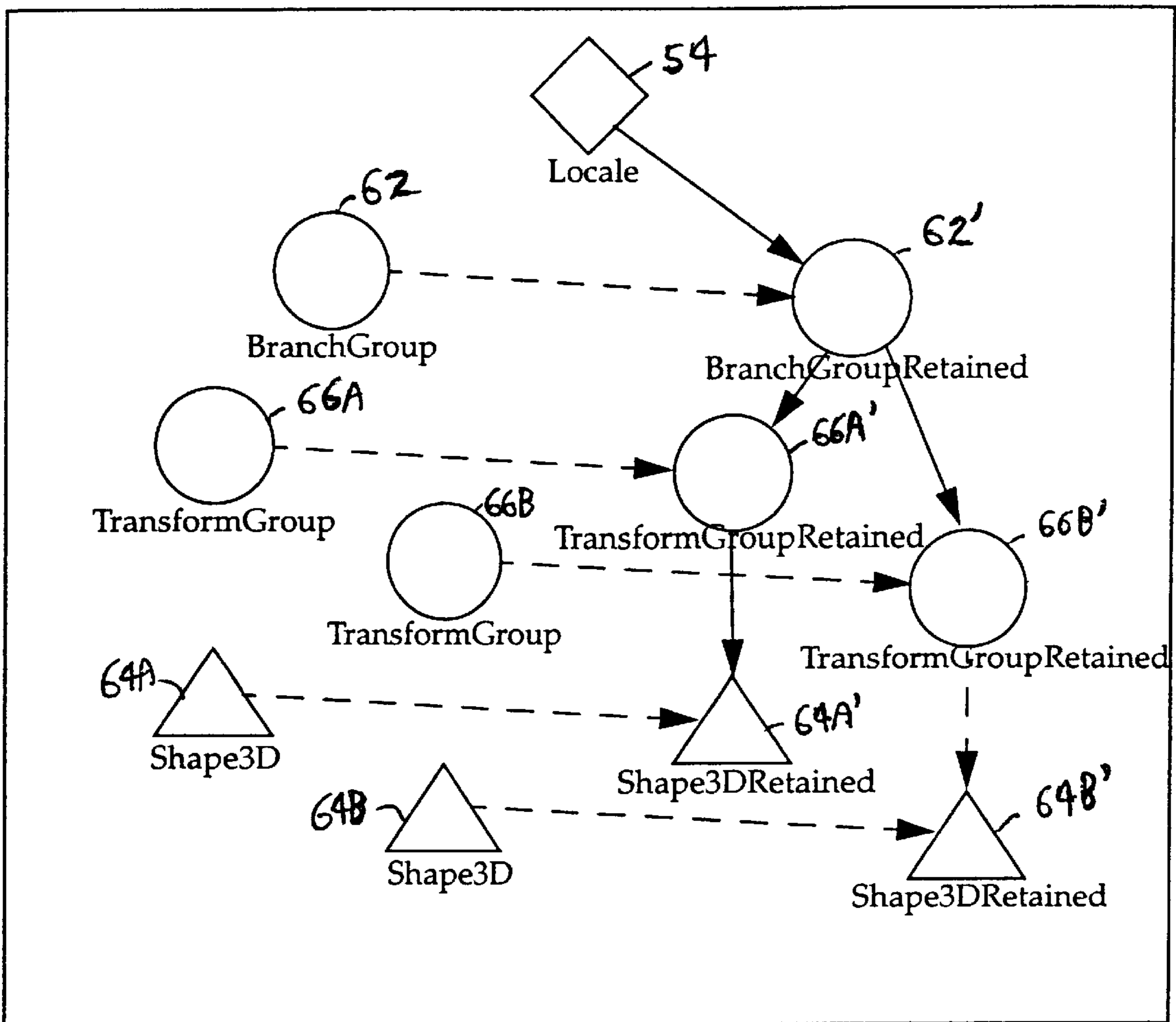
Figure 6 Scene Graph Internal Structure
