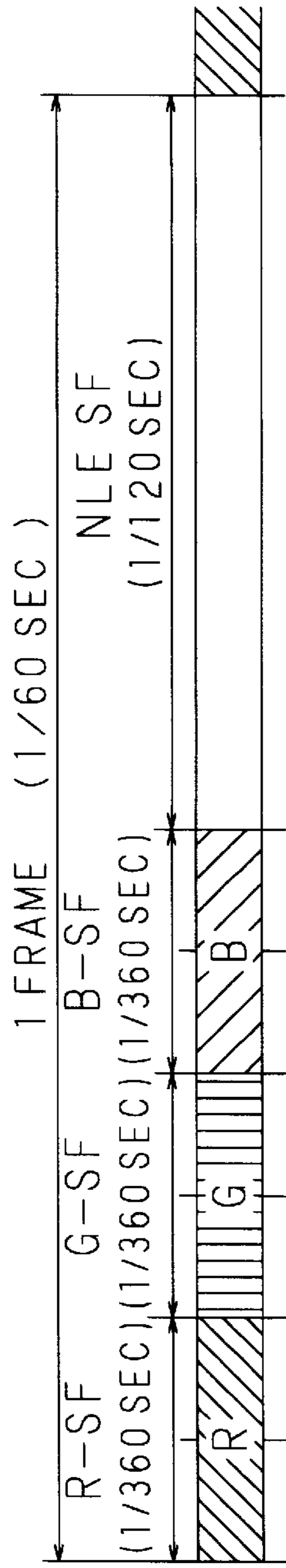
FIG. 1 2A BACK-LIGHT EMISSION
