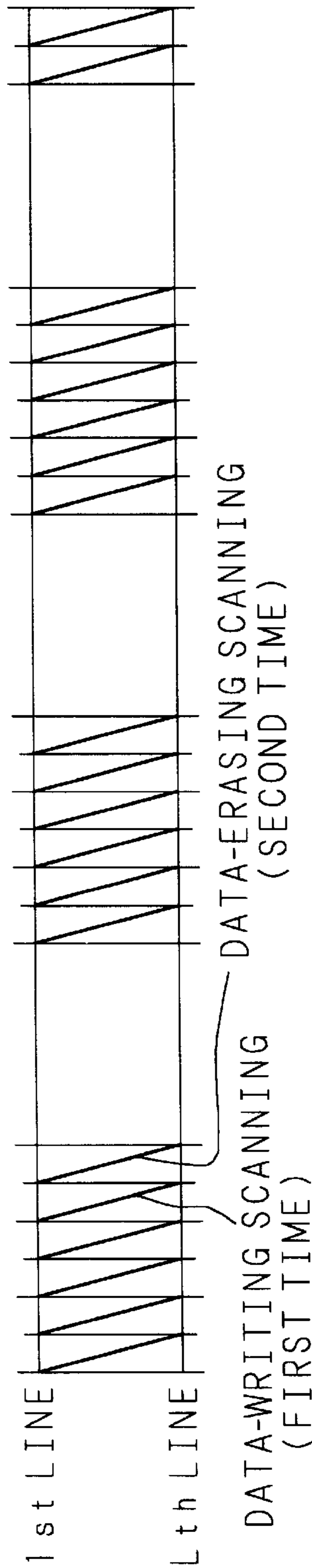
FIG. 16B LCD PANEL SCANNING
