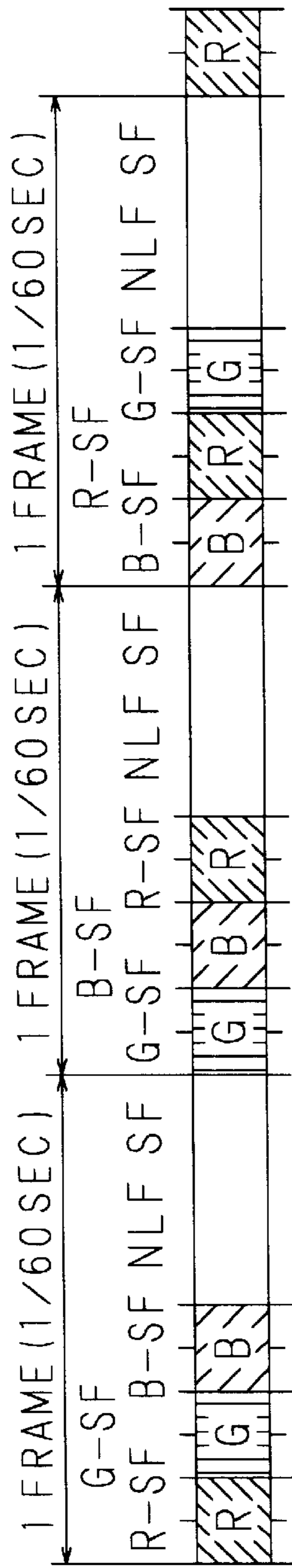
FIG. 16A BACK-LIGHT EMISSION
