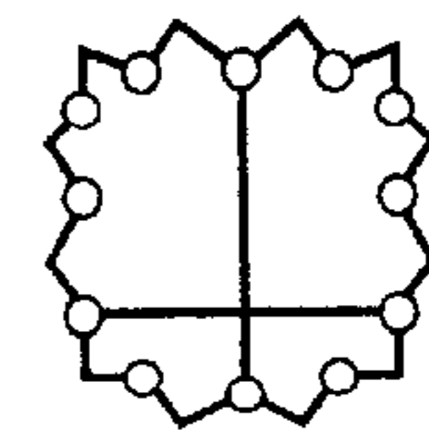
ZEOLITE B
