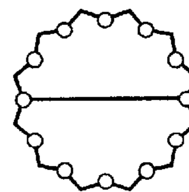
FAUASITE
