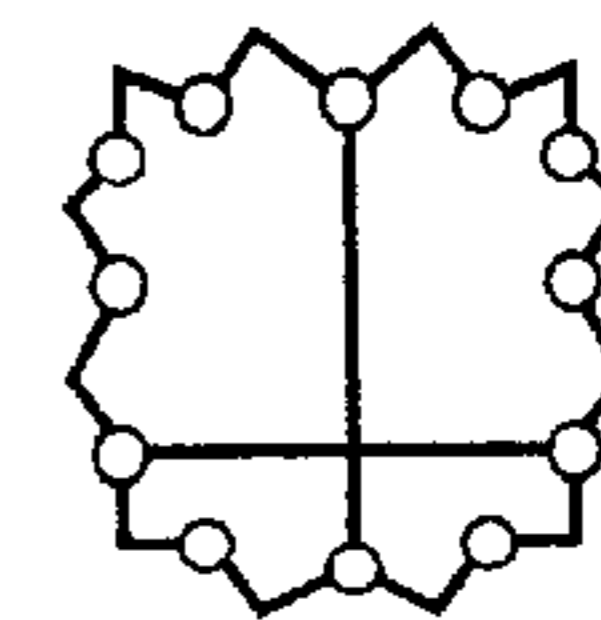
ZEOLITE B
