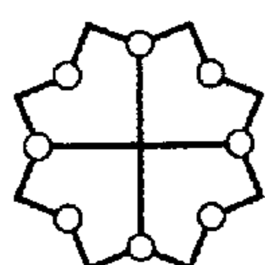
ZEOLITE A
