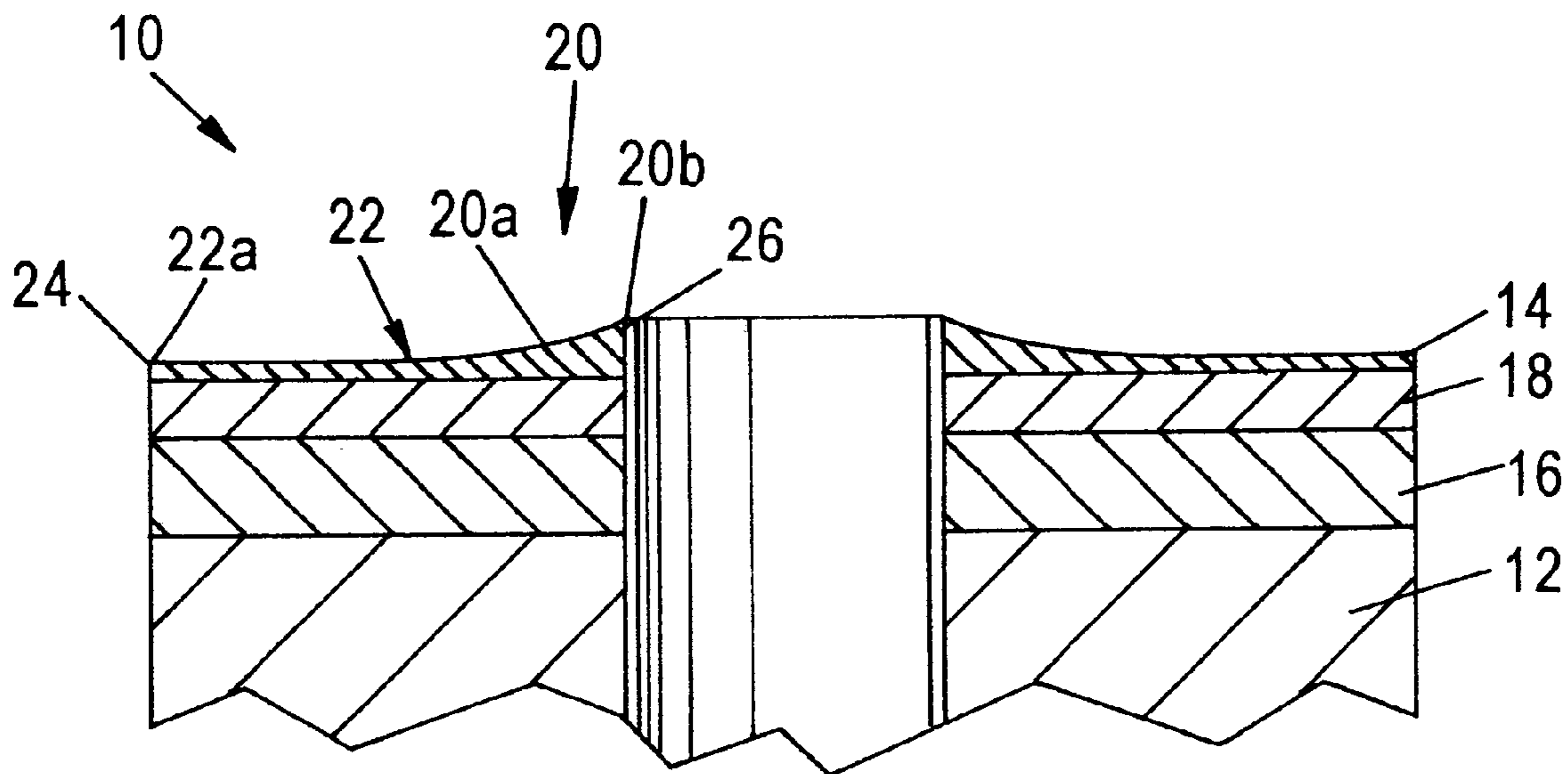
FIG. 1 (PRIOR ART)
