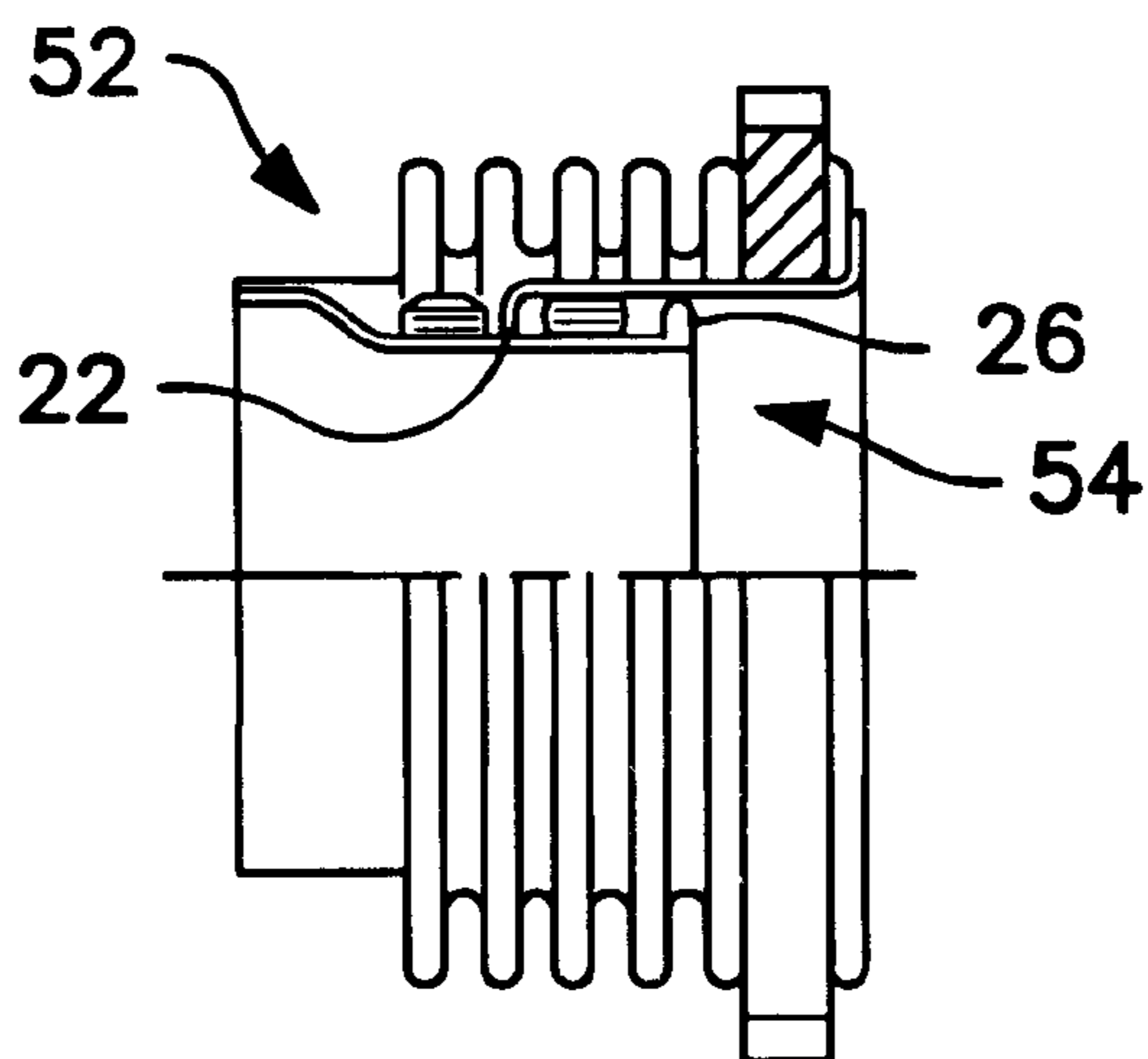
ASSEMBLE PART 1 TO PART 2
