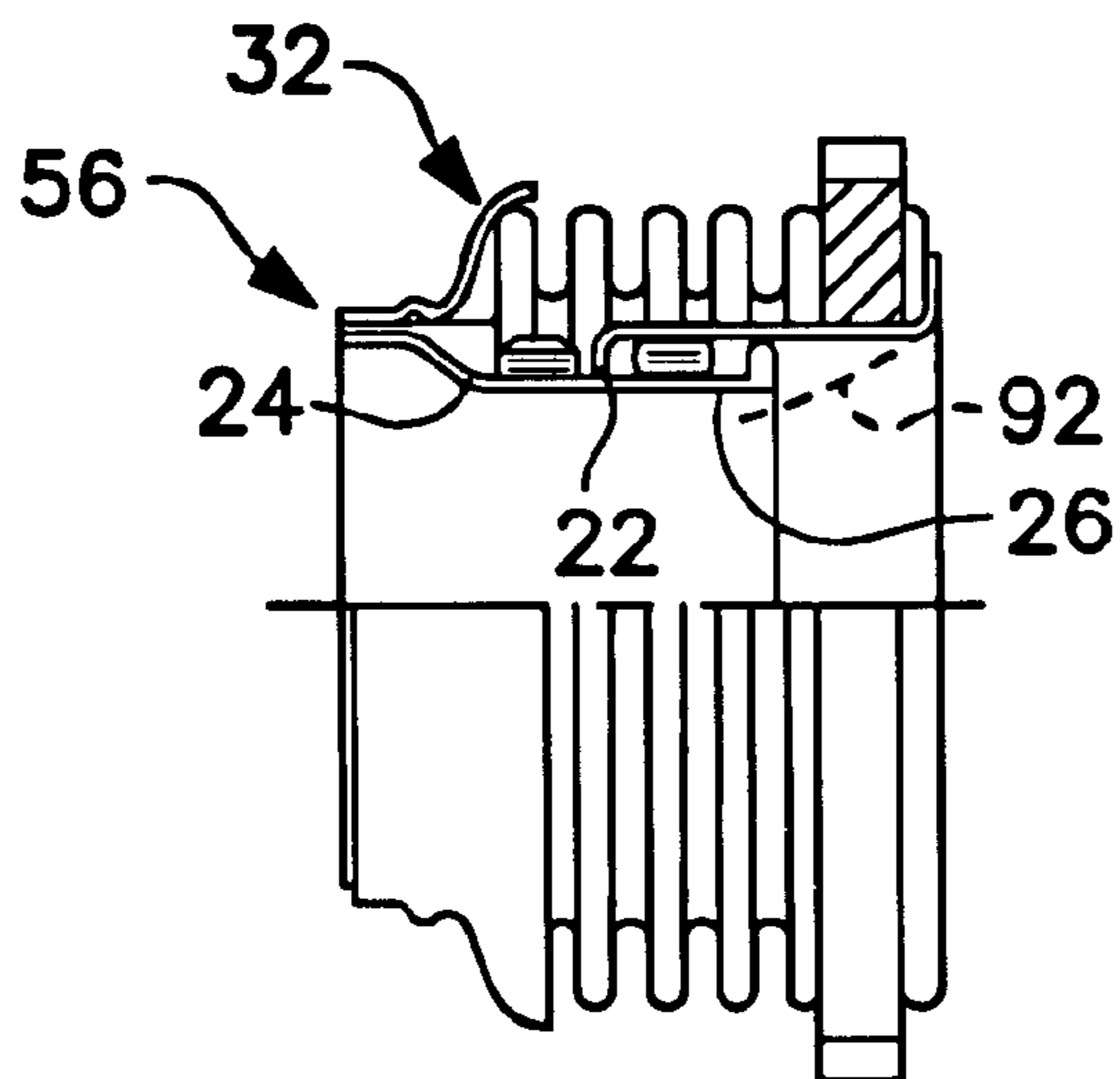
ASSEMBLE & SIZE END CAP
