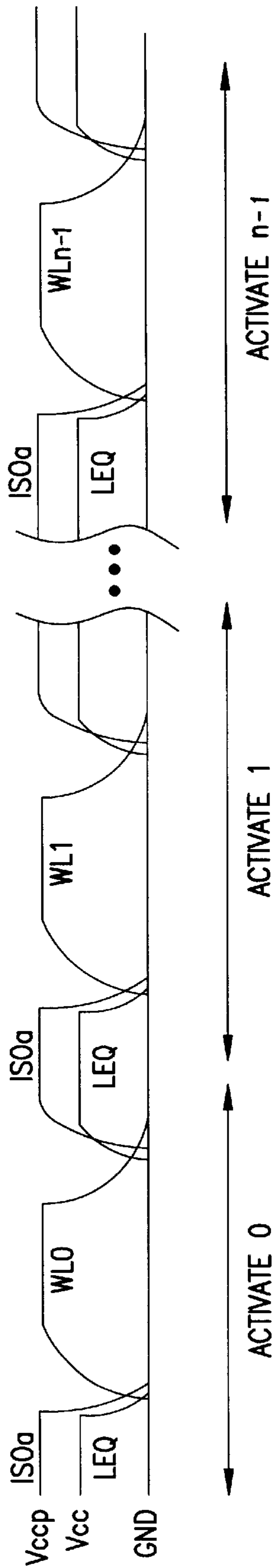
FIG. 4 (PRIOR ART)
