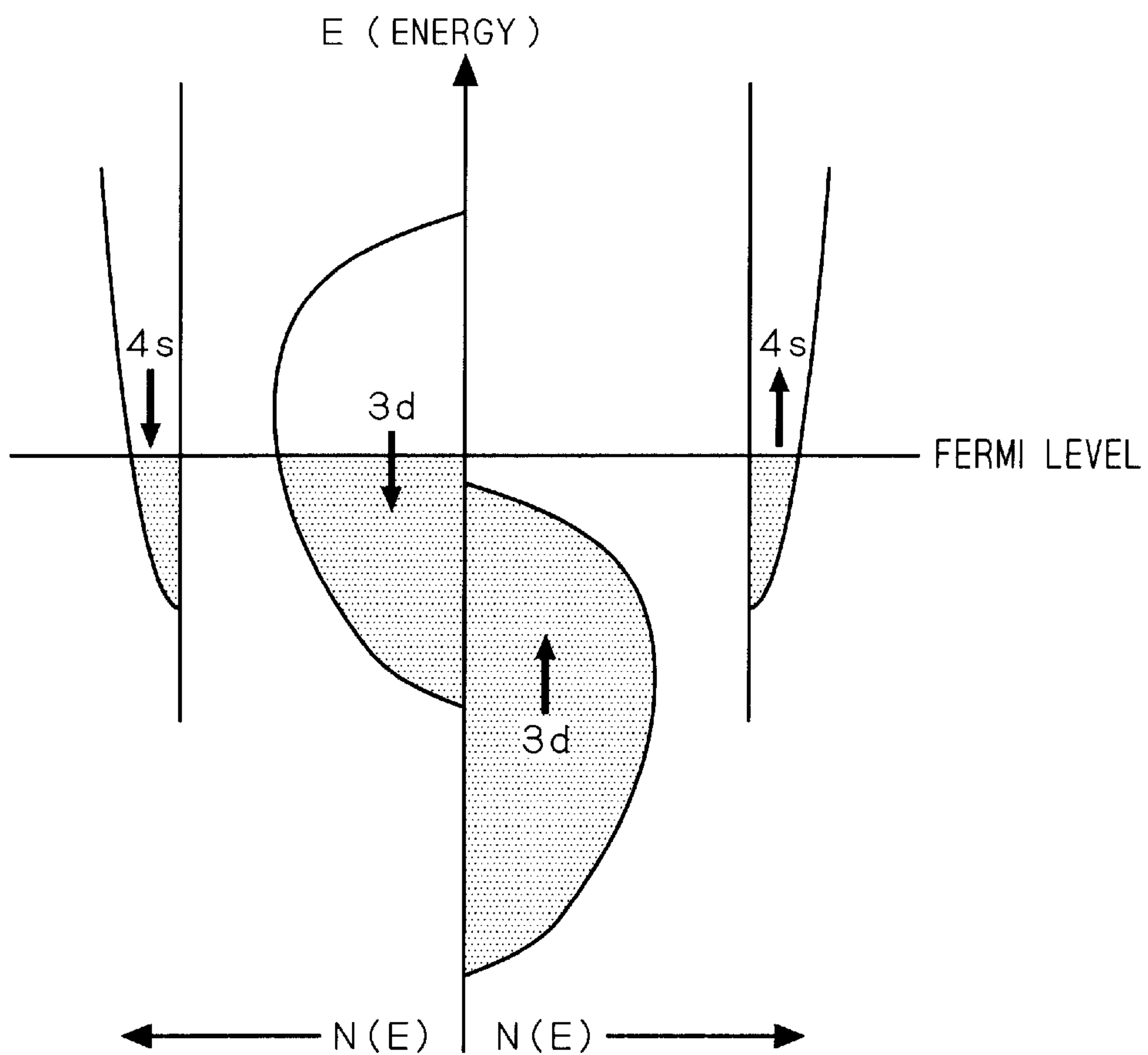
FIG. 68 (BACKGROUND ART)
