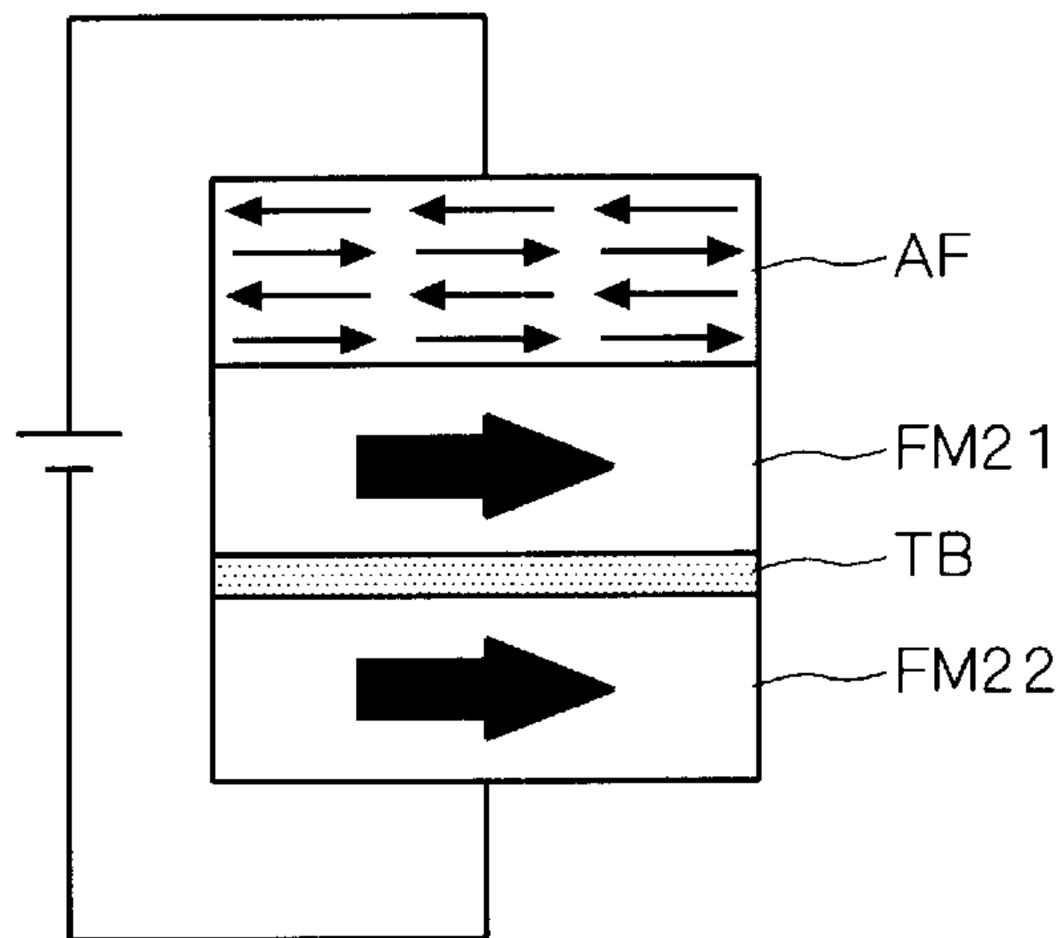
FIG. 71 (BACKGROUND ART)
