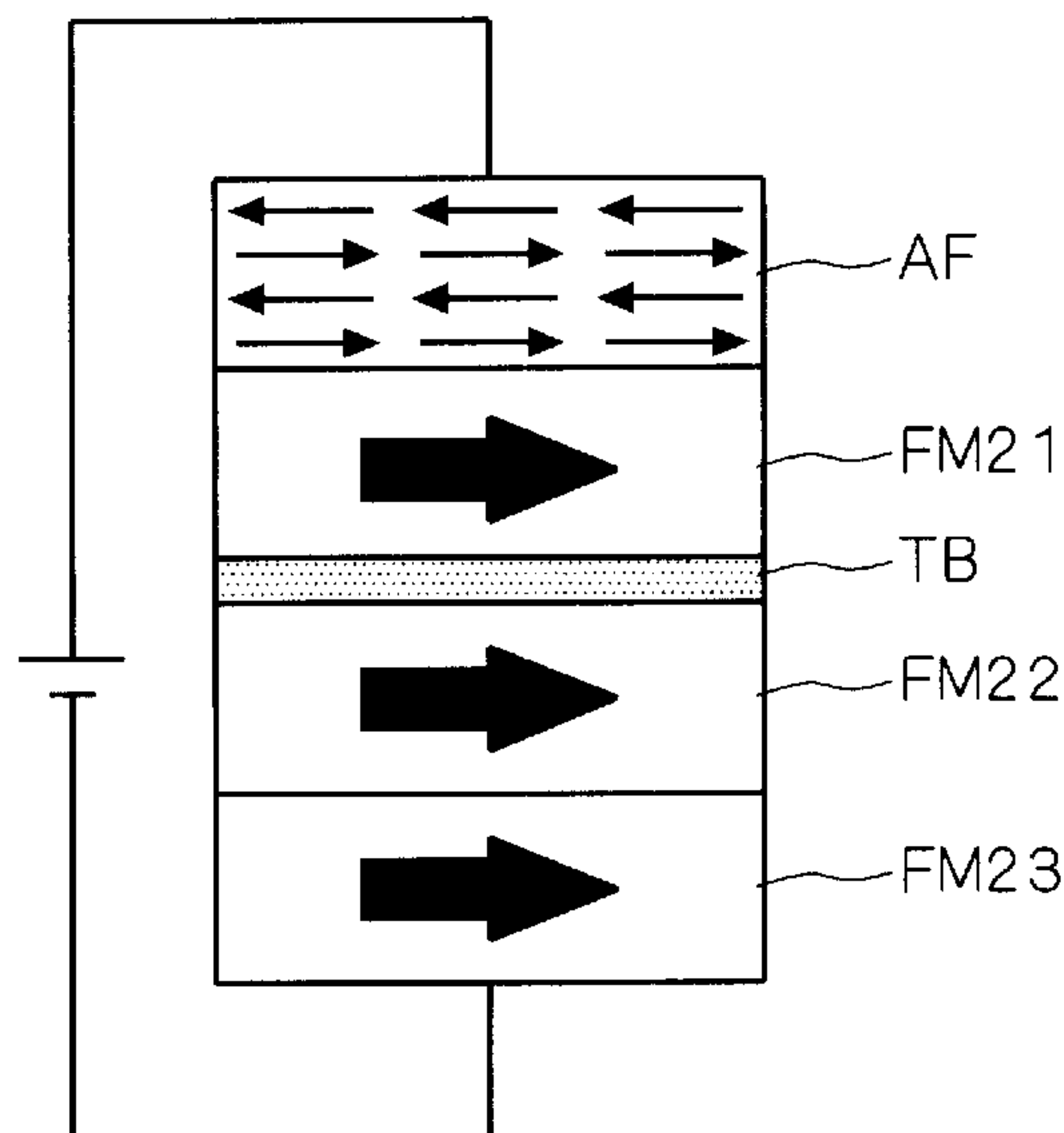
FIG. 72 (BACKGROUND ART)
