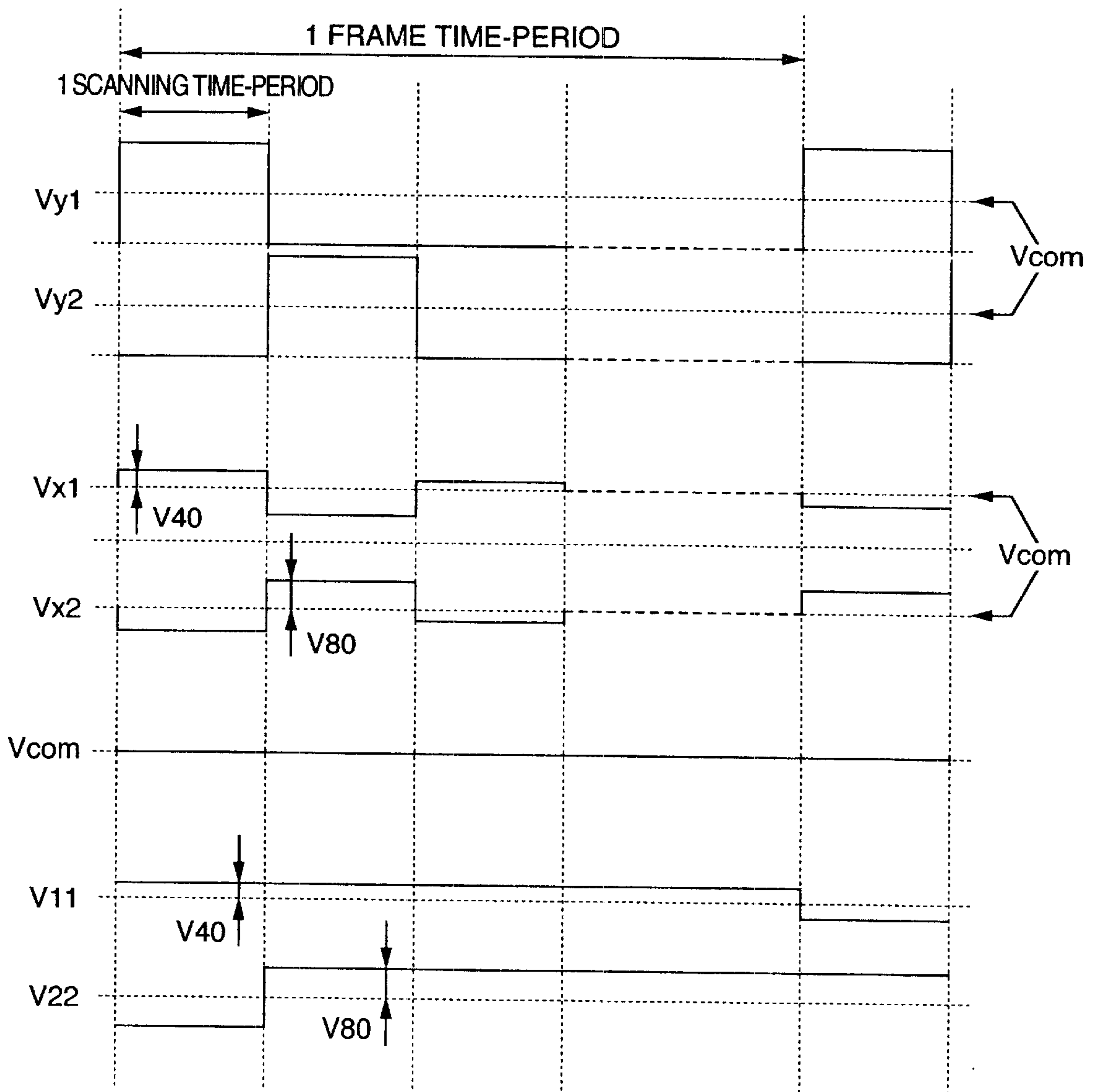
FIG.3 (PRIOR ART)
