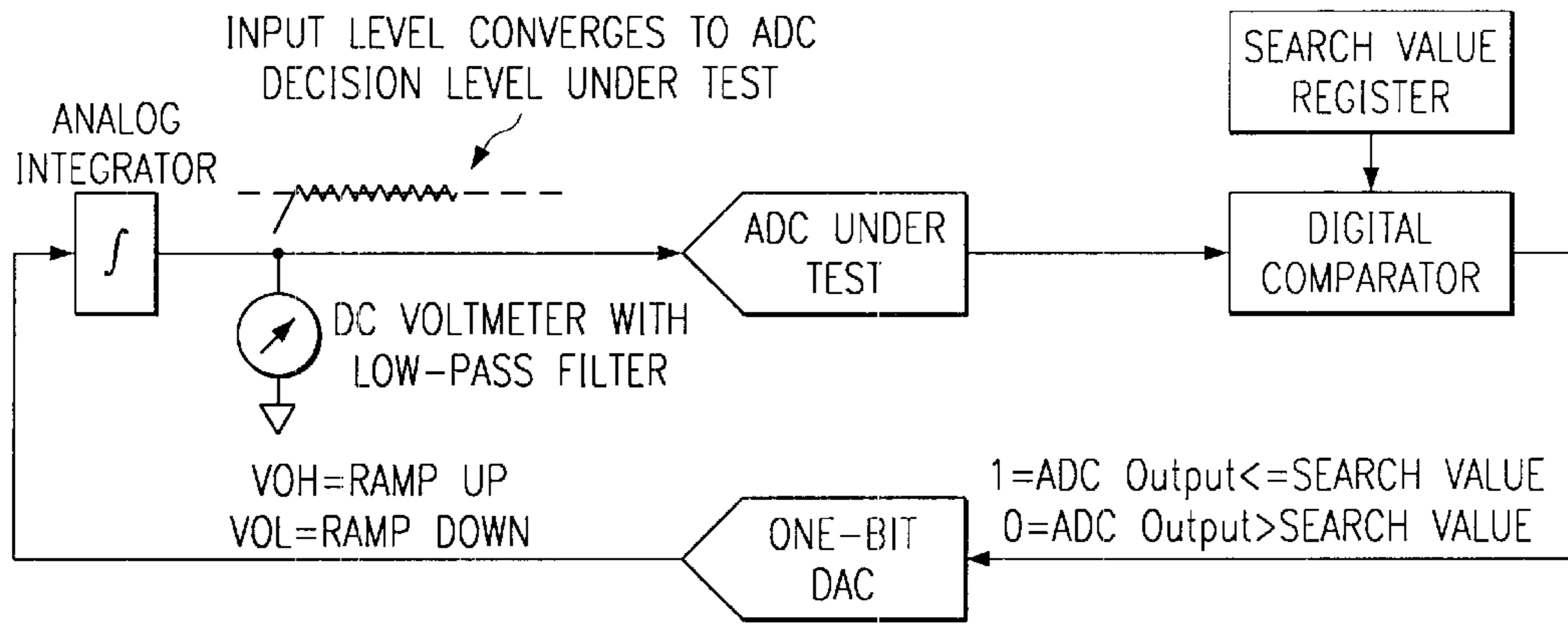
FIG. 1 (PRIOR ART)
