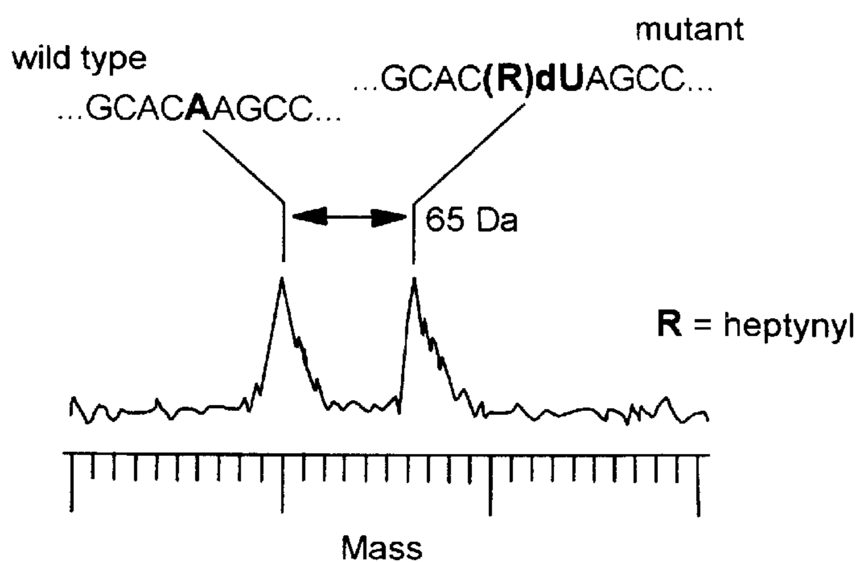
Mass Spectra of a heterozygous mix of wild type and mutant where A has mutated to T. T has been replaced by heptynyldeoxyuridine during amplification of the mutant region. Spectral peaks are now separated by 65 mass units.
