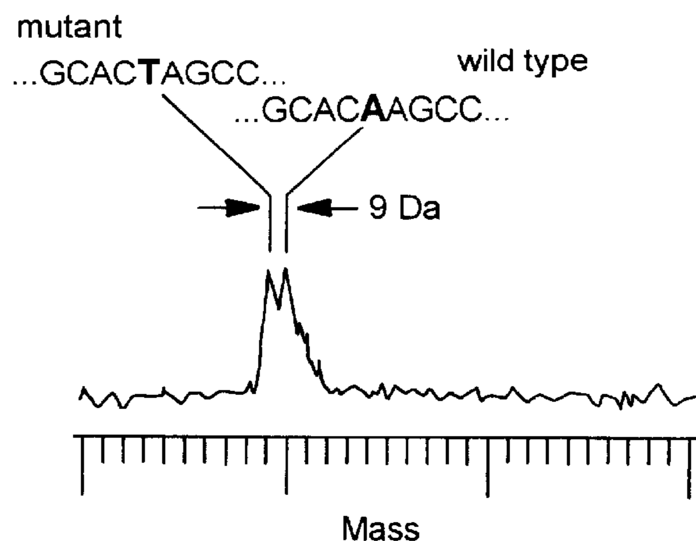
Mass Spectra of a heterozygous mix of wild type and mutant where A has mutated to T. Spectral peaks are separated by 9 mass units.
