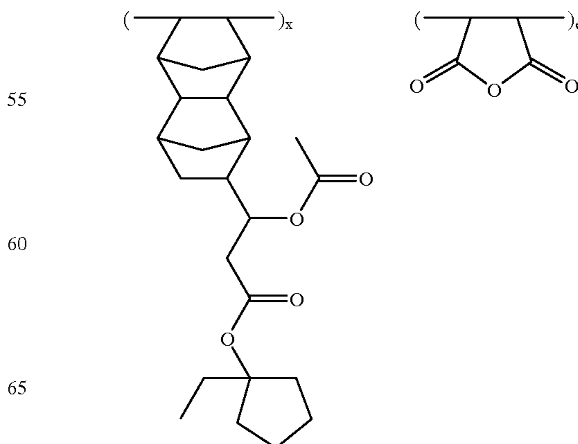
(x = 0.50, e = 0.50, Mw = 15,100)
