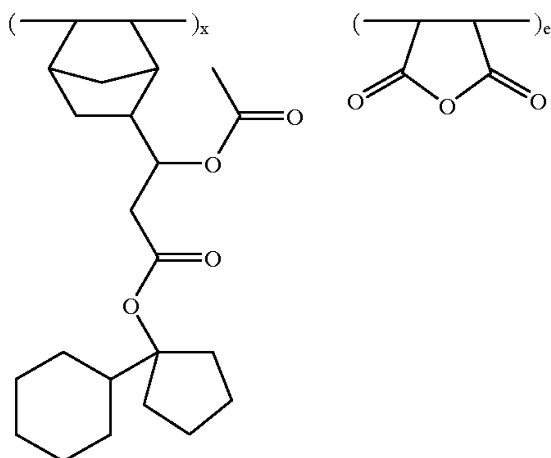
(Polymer 2) (x = 0.50, e = 0.50, Mw = 14,300)
