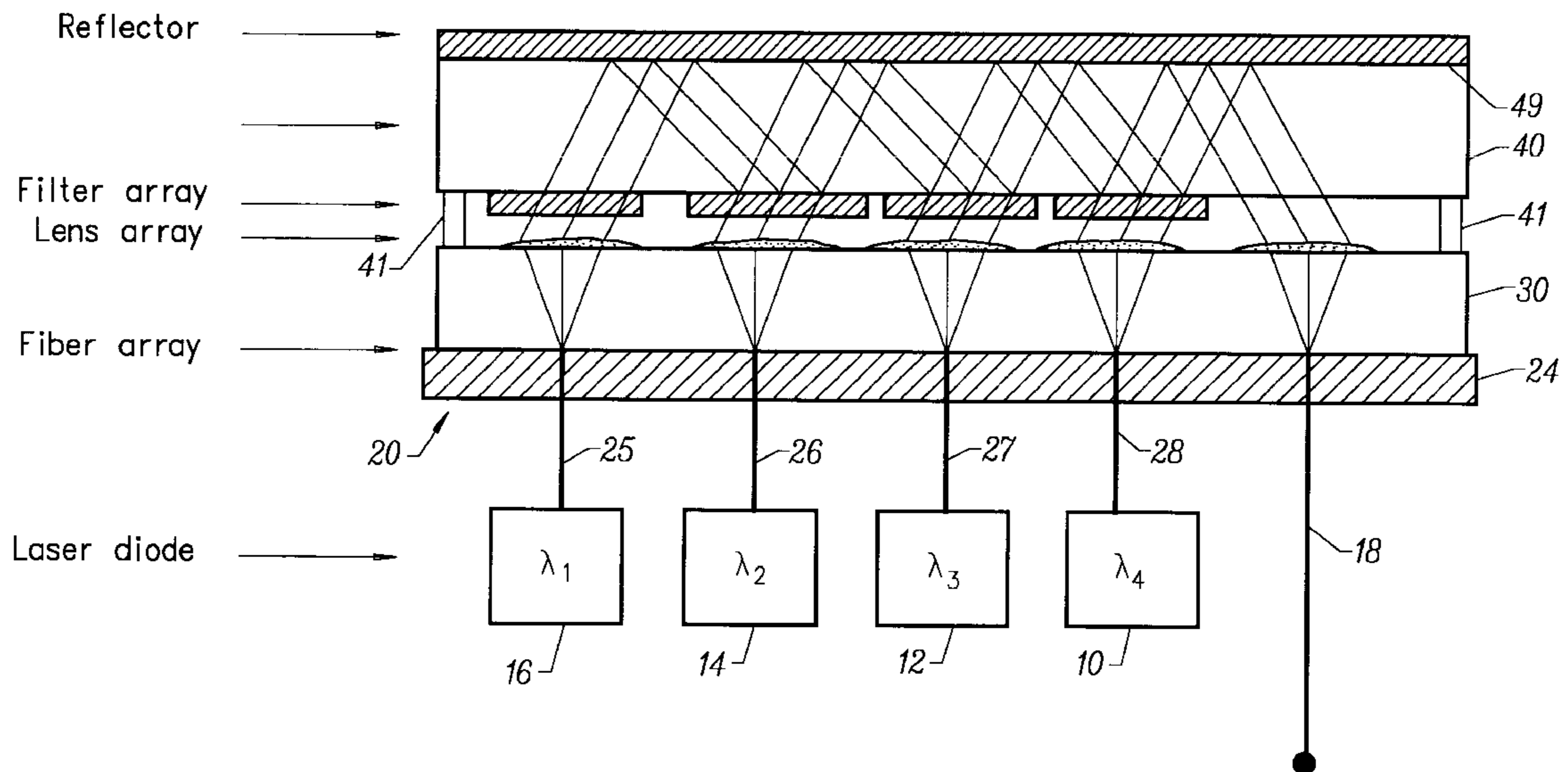
Multiplexer (MUX) consisting of light-source, fiber array, lens array and filter array
