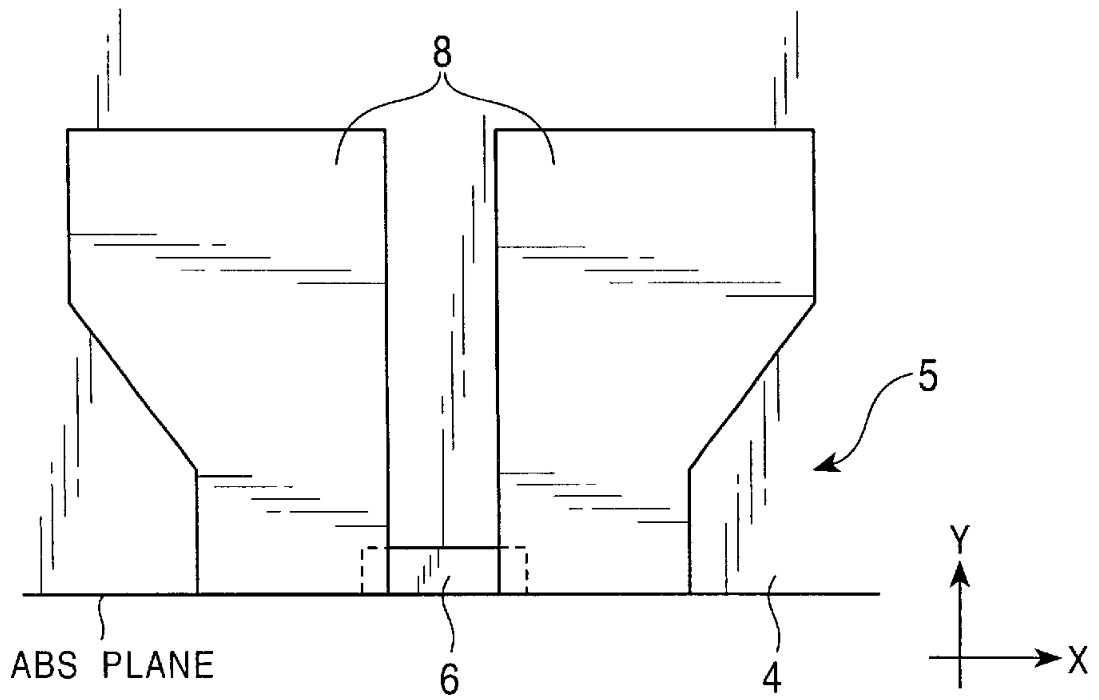
FIG. 22 PRIOR ART
