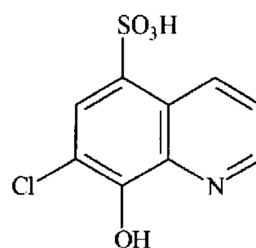
7-Chloro-8-hydroxy-5-quinolinesulfonic acid
