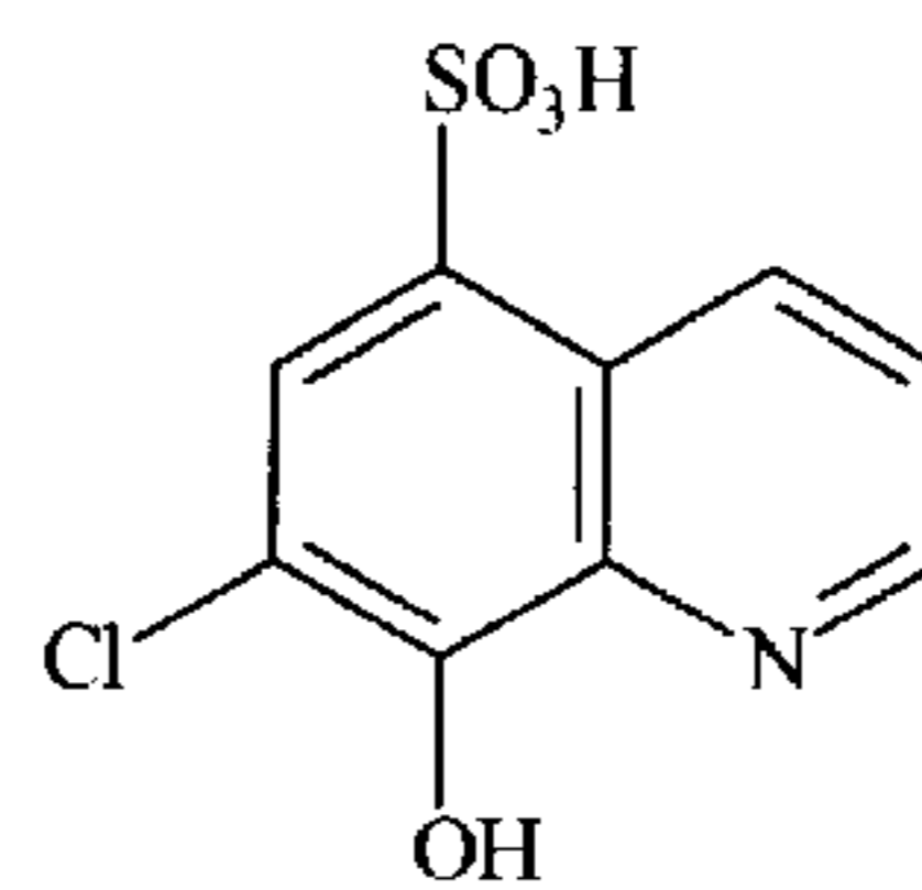
7-Chloro-8-hydroxy-5-quinolinesulfonic acid
