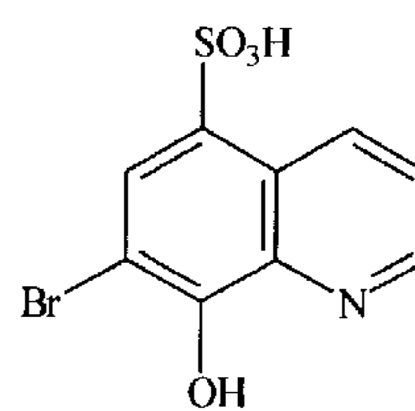
7-Bromo-8-hydroxy-5-quinolinesulfonic acid
