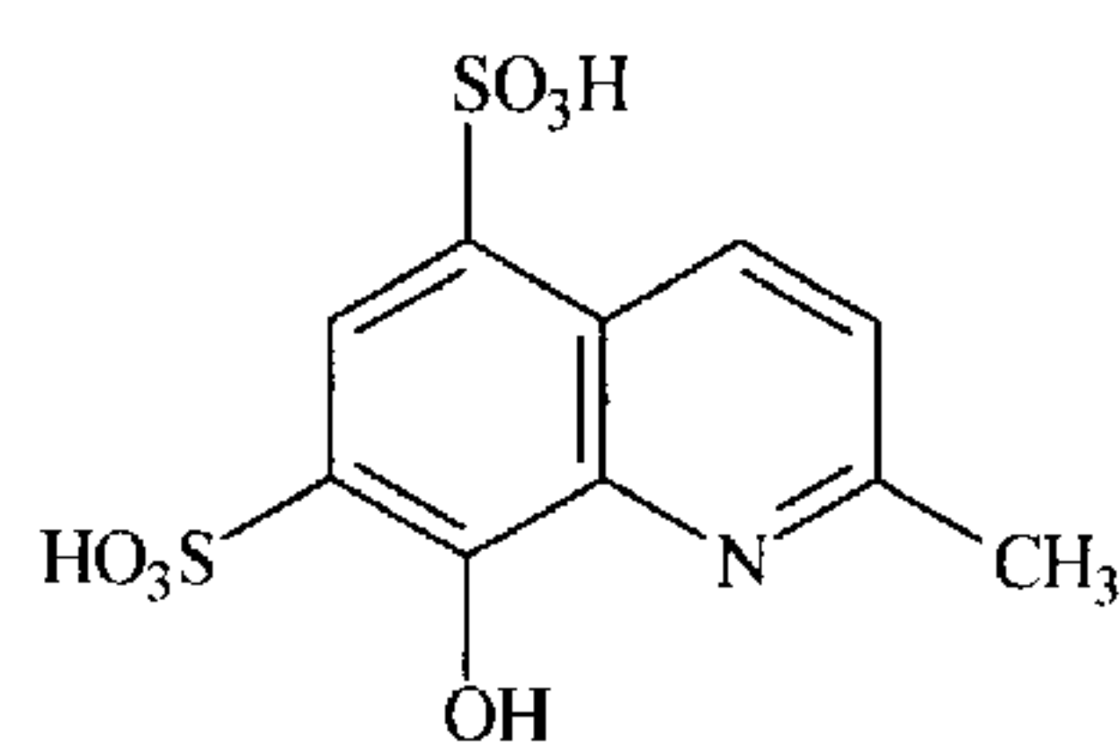
8-hydroxy-2-methyl-5,7-quinolinedisulfonic acid
