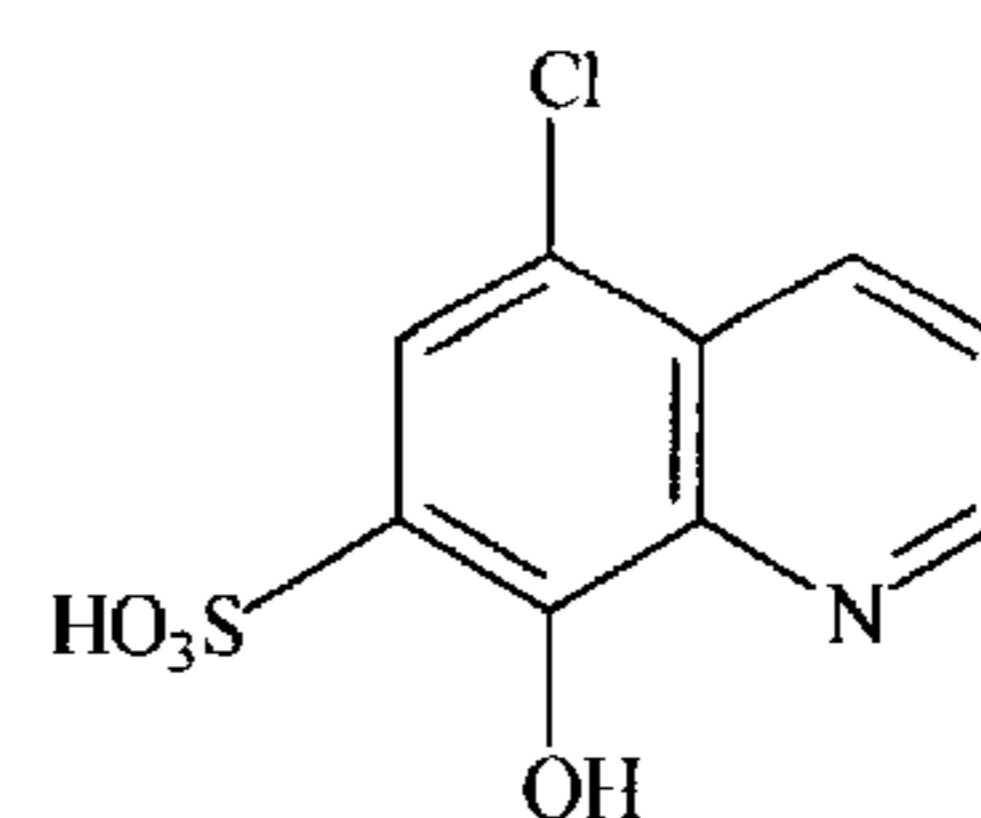
5-Chloro-8-hydroxy-7-quinolinesulfonic acid
