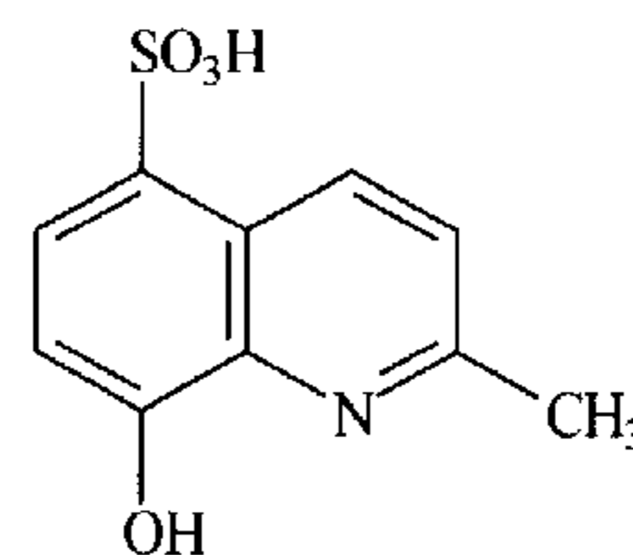
8-hydroxy-2-methyl-5-quinolinesulfonic acid
