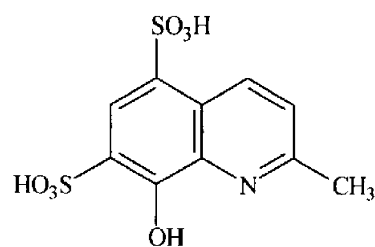
8-hydroxy-2-methyl-5,7-quinolinedisulfonic acid
