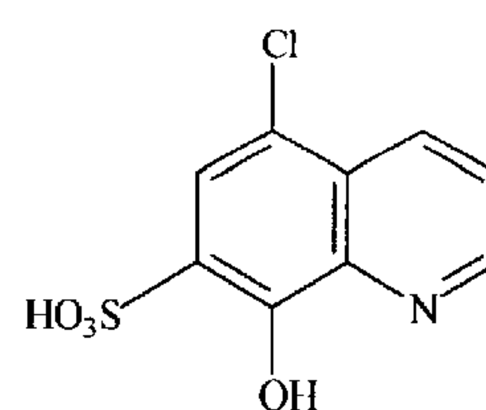
5-Chloro-8-hydroxy-7-quinolinesulfonic acid
