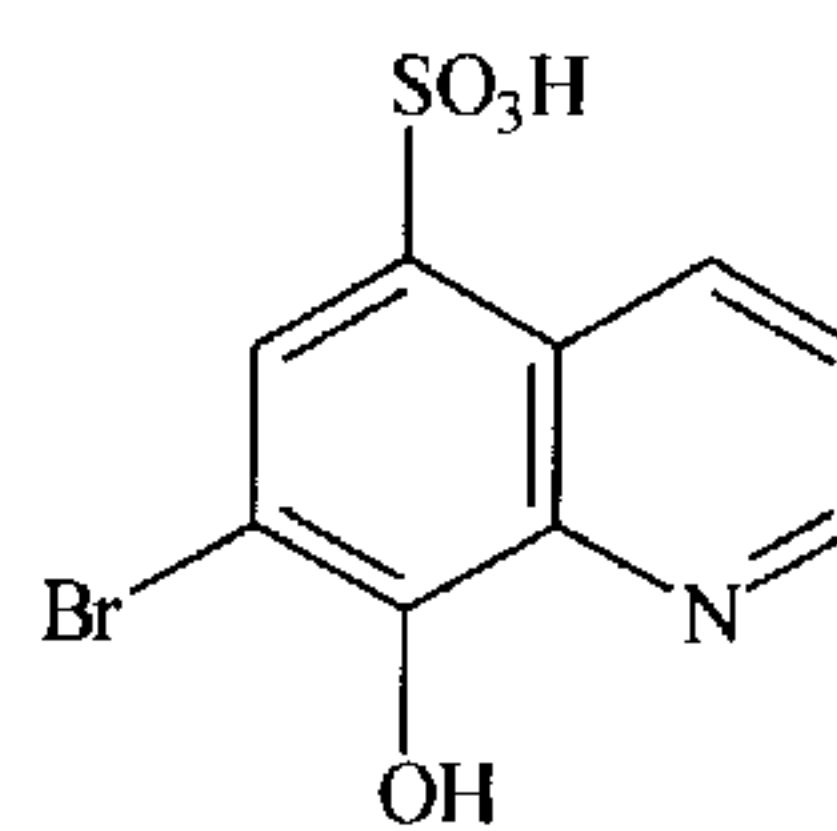
7-Bromo-8-hydroxy-5-quinolinesulfonic acid
