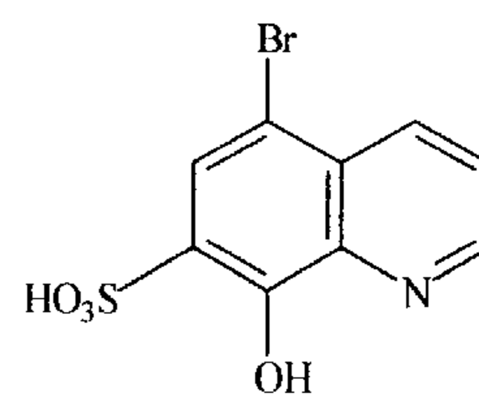
5-Bromo-8-hydroxy-7-quinolinesulfonic acid
