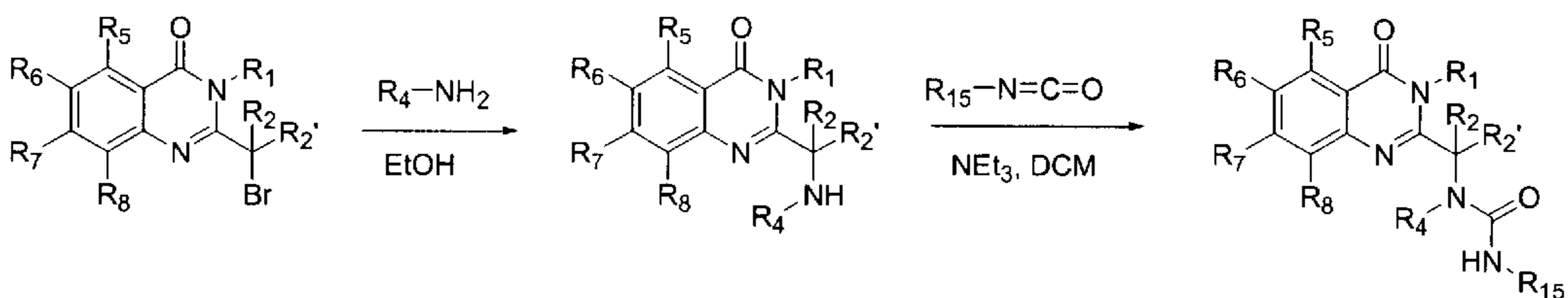
Figure 5d: Primary and Secondary Amine R4 Synthesis
