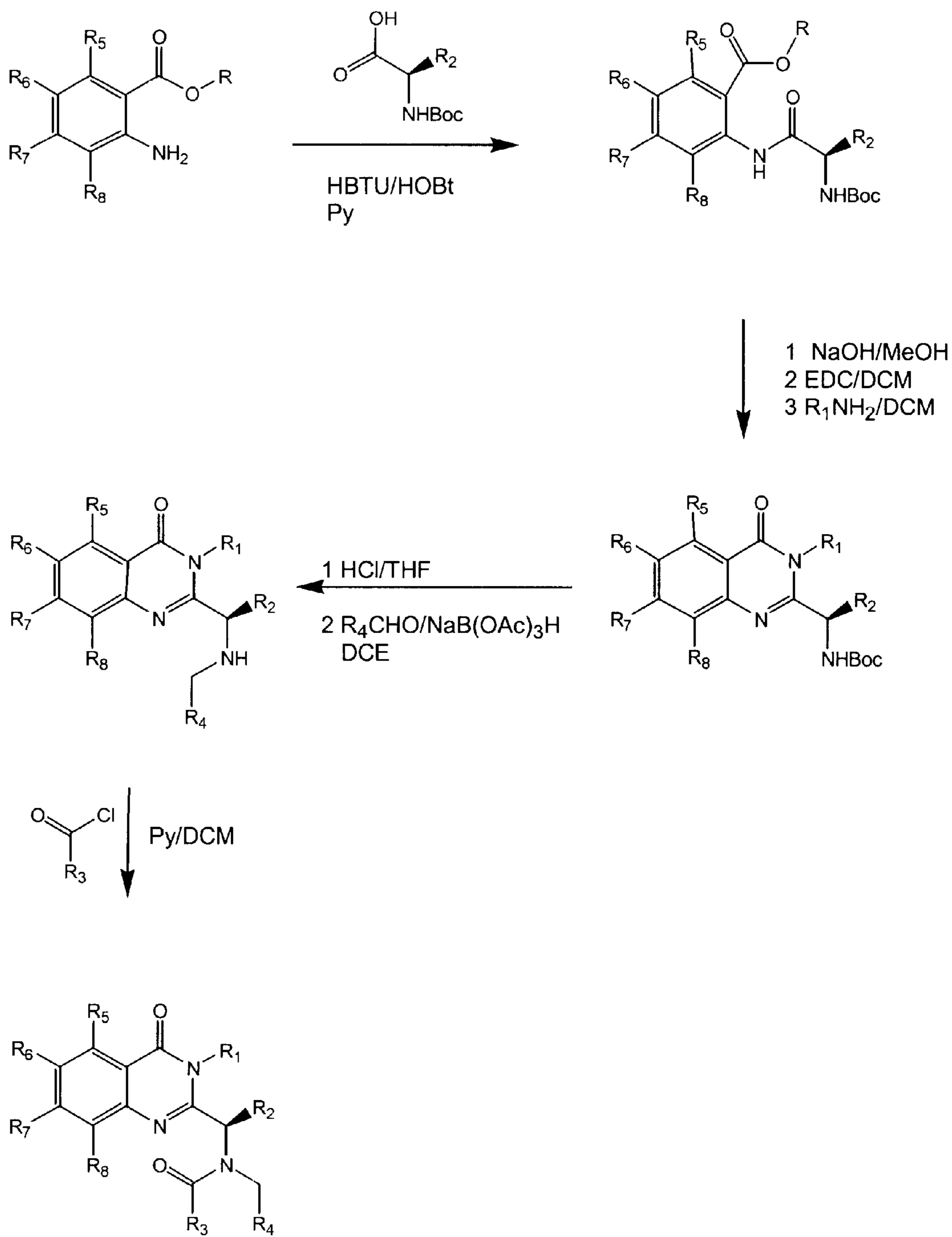
Figure 4: Asymmetric Synthesis
