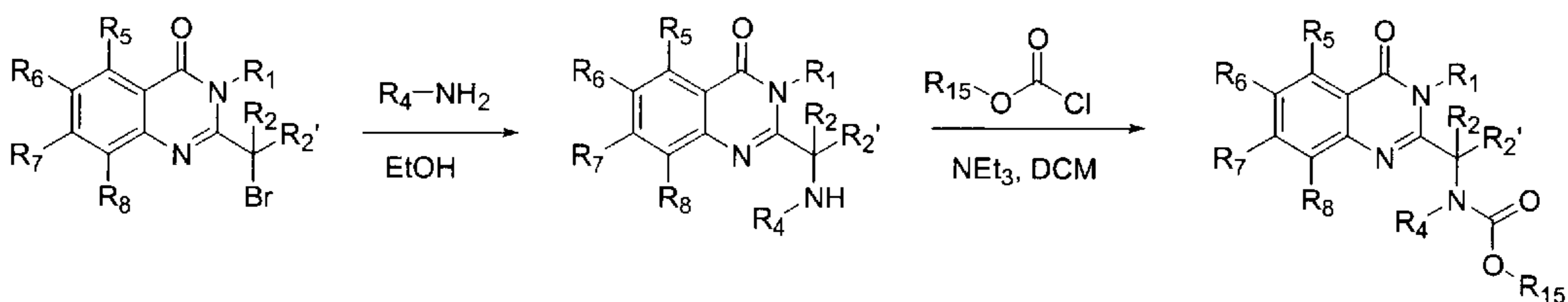
Figure 5c: Urea Synthesis
