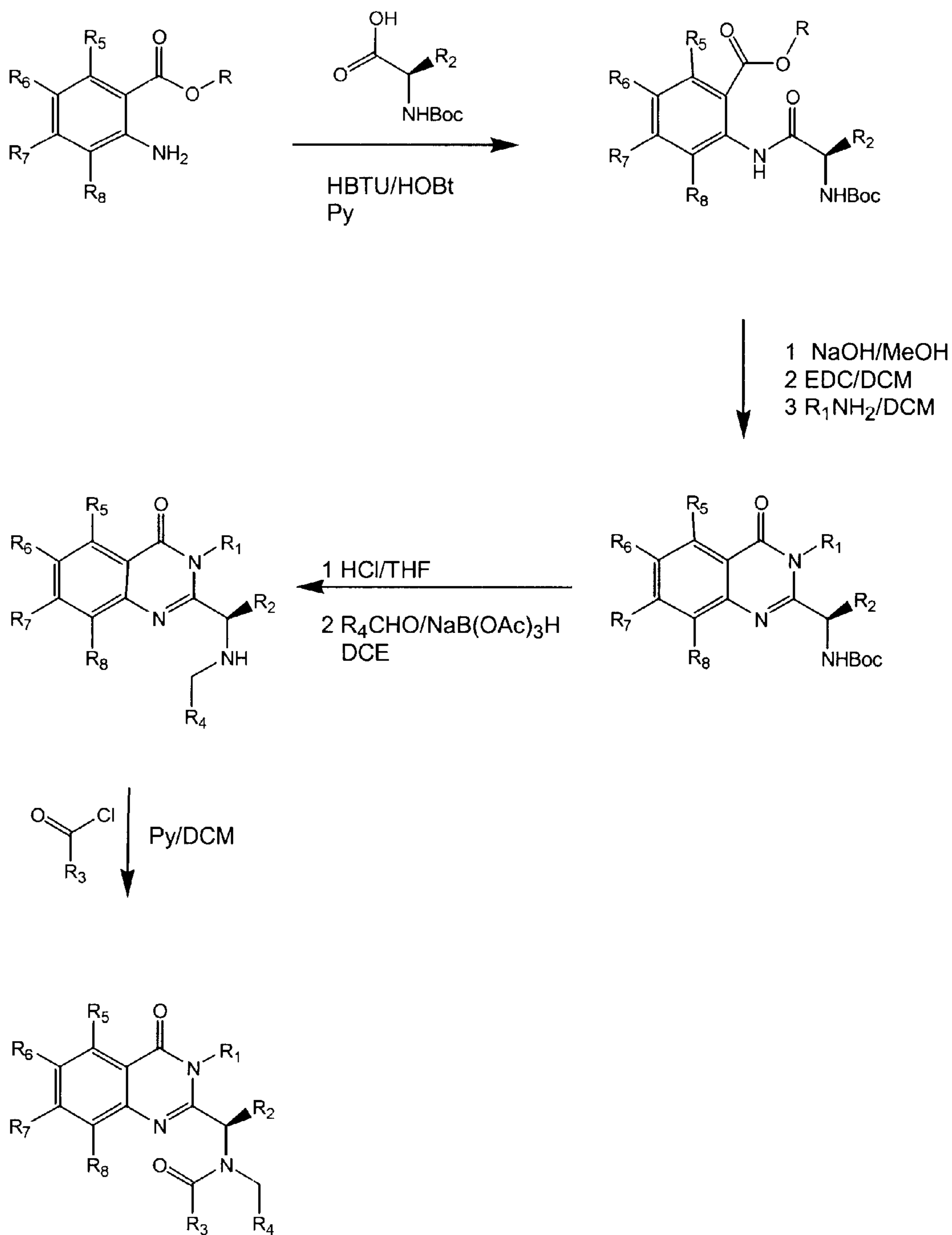
Figure 4: Asymmetric Synthesis
