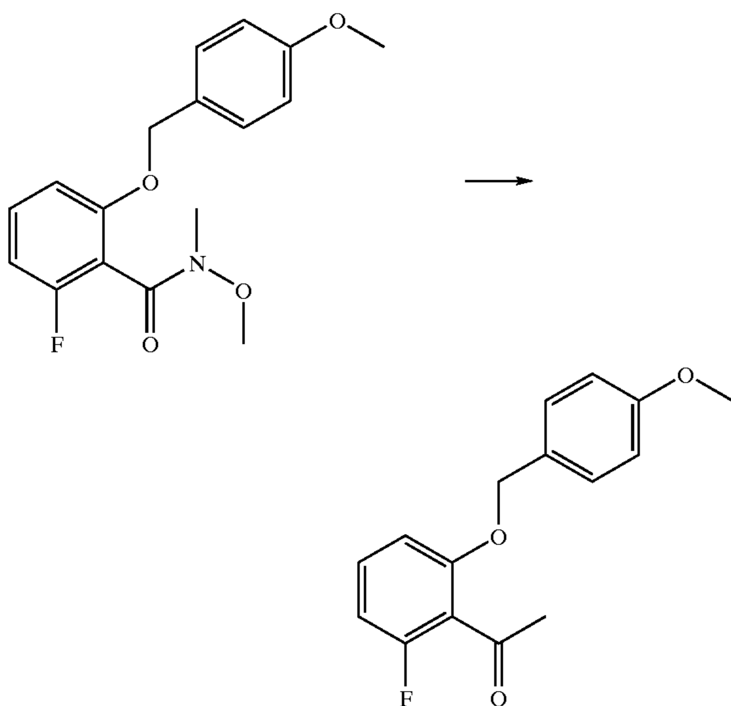
(Starting compound 1I)
