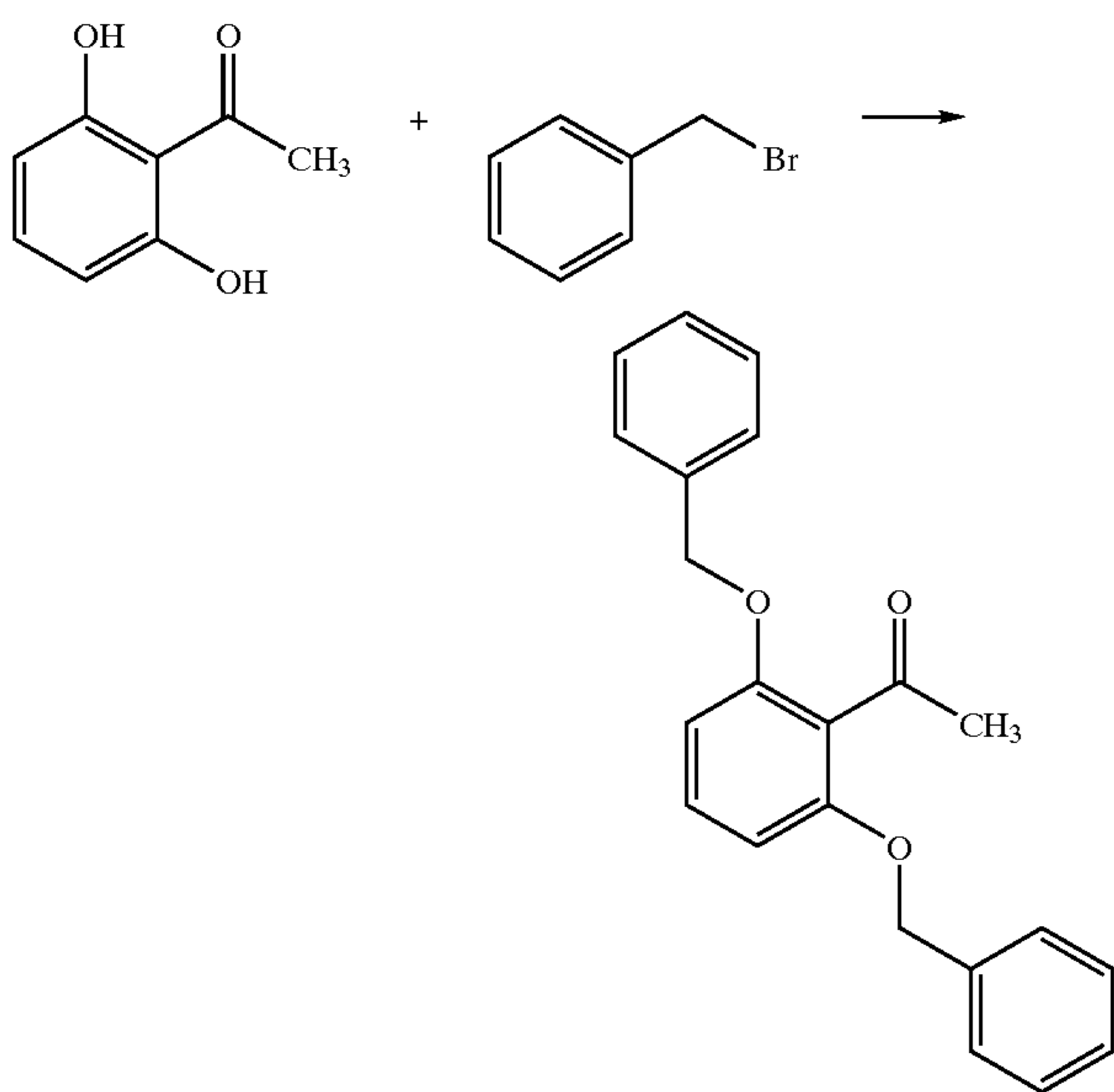
(Starting compound 1E)
