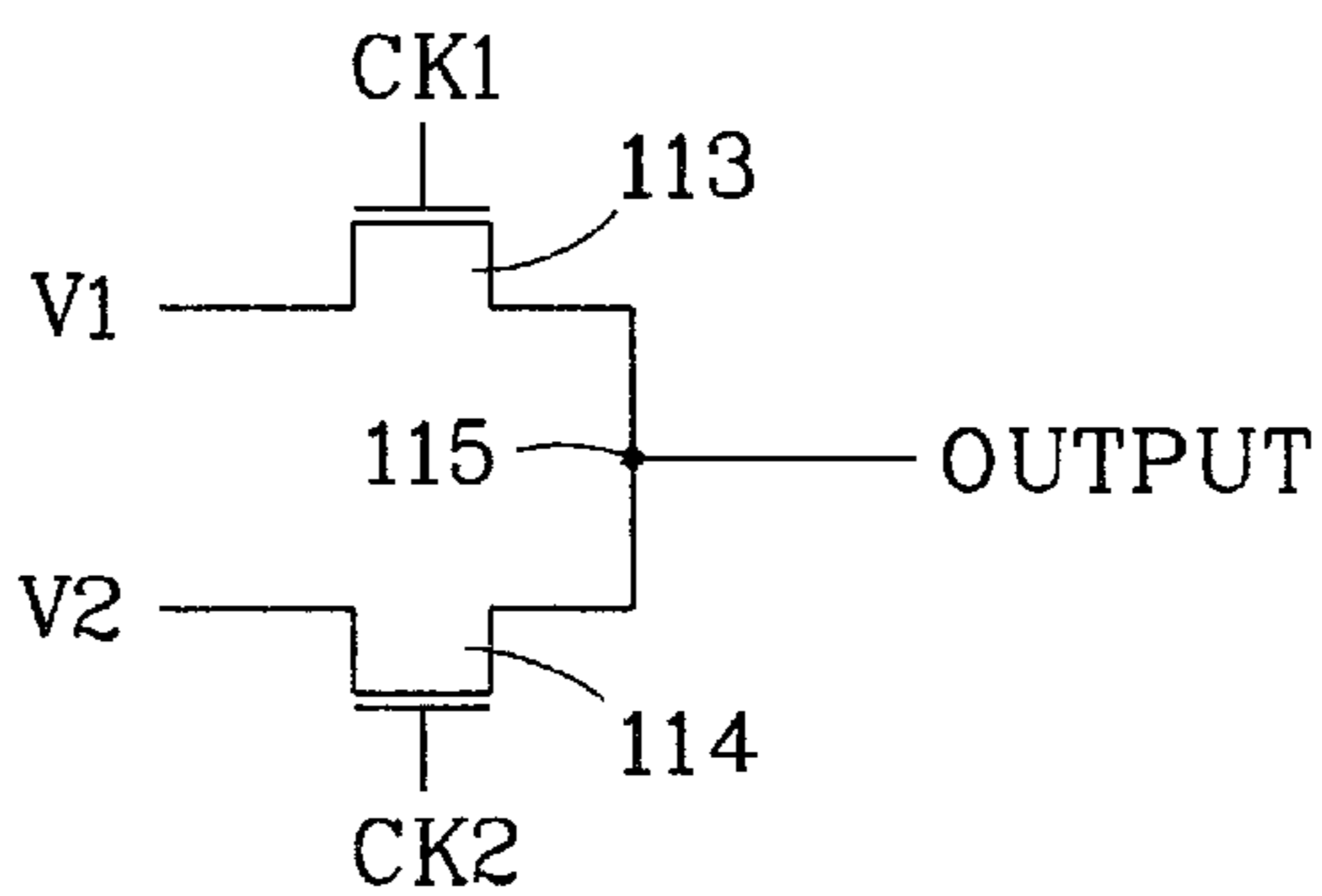
FIG. 1C PRIOR ART
