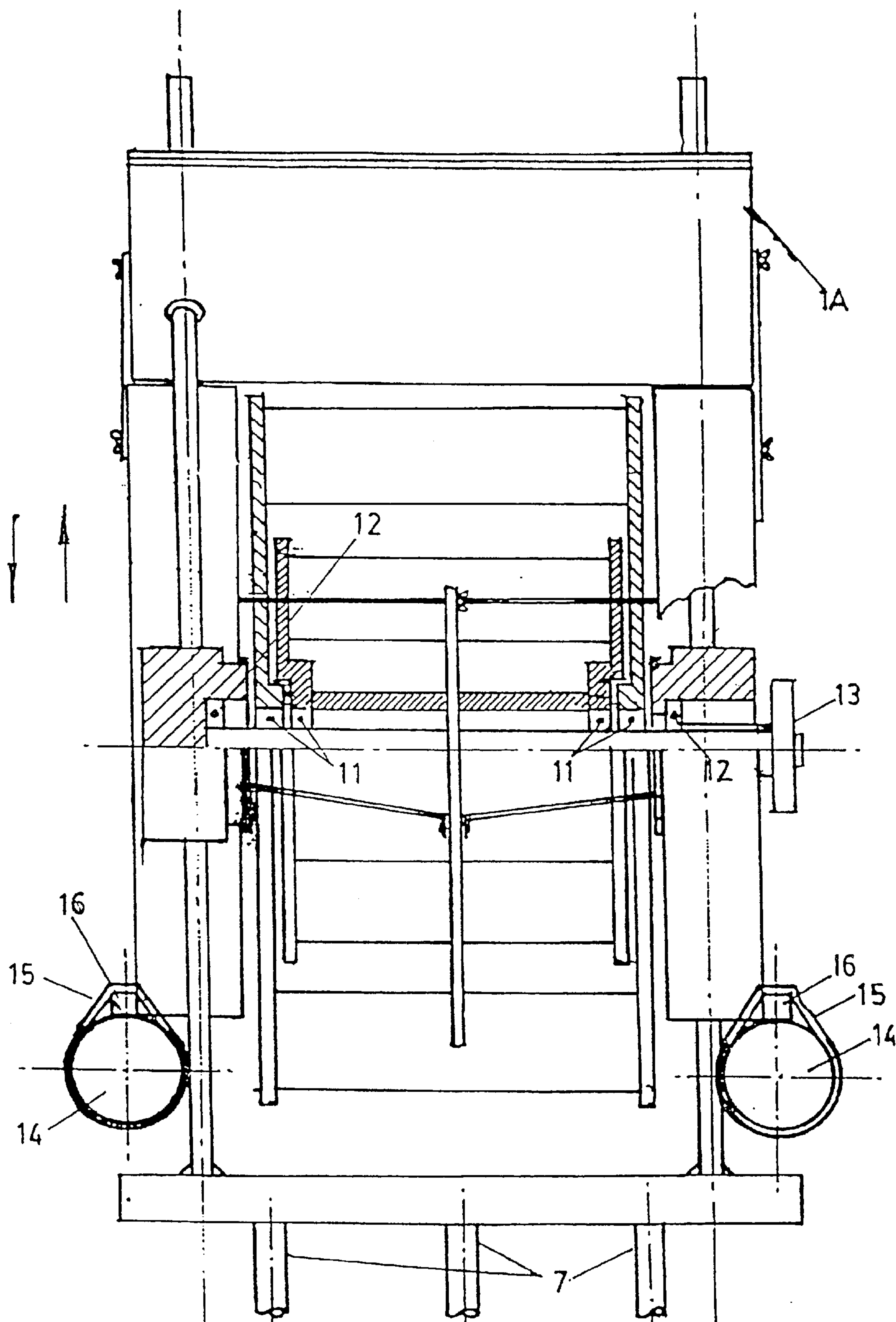
FIG 2 SIDE VIEW "B"
