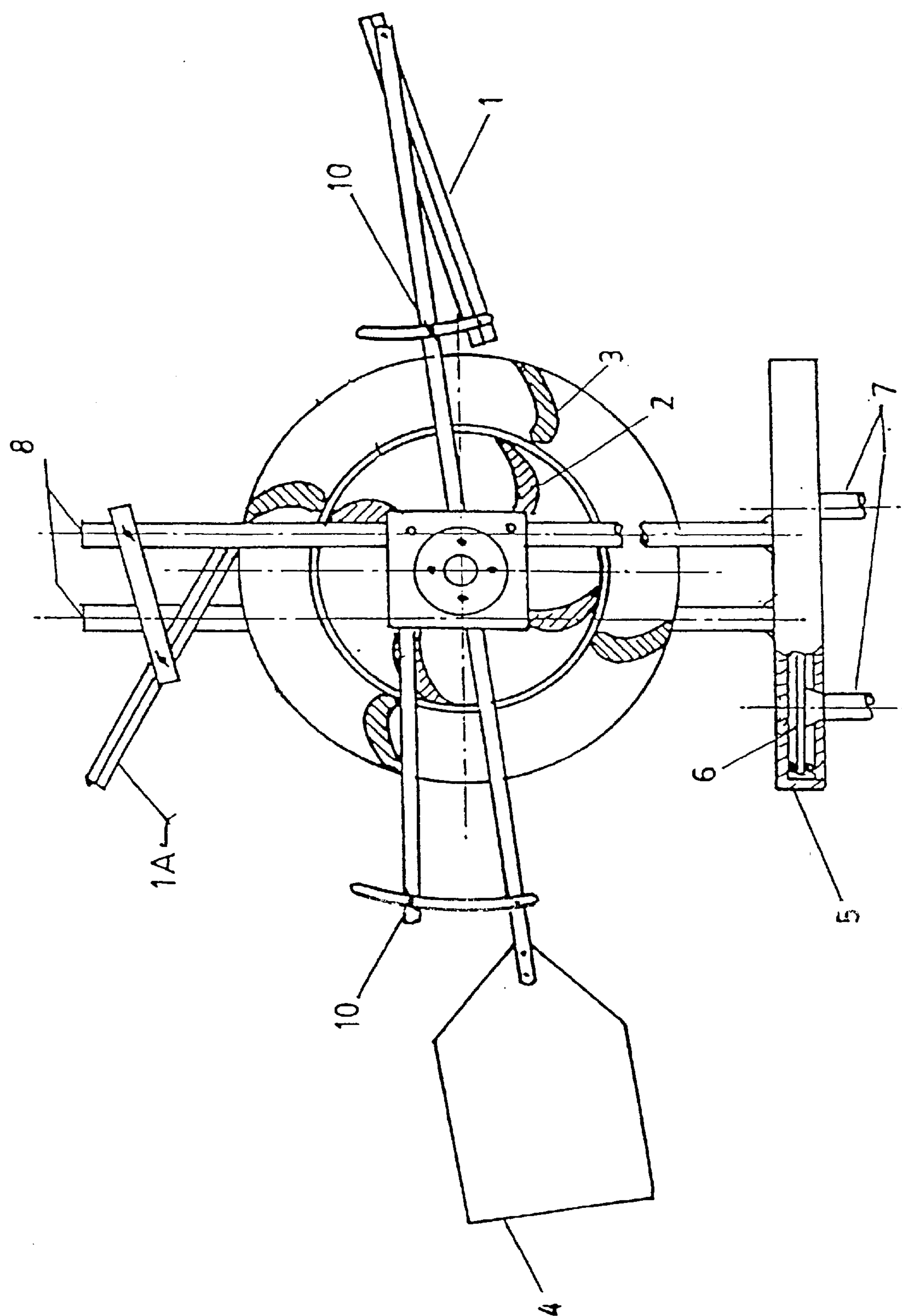
FIG 5 FRONT ELEVATION
