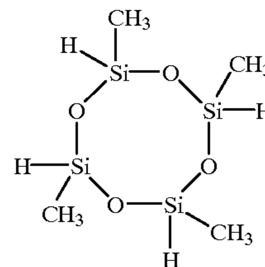
Chemical Formula 16
