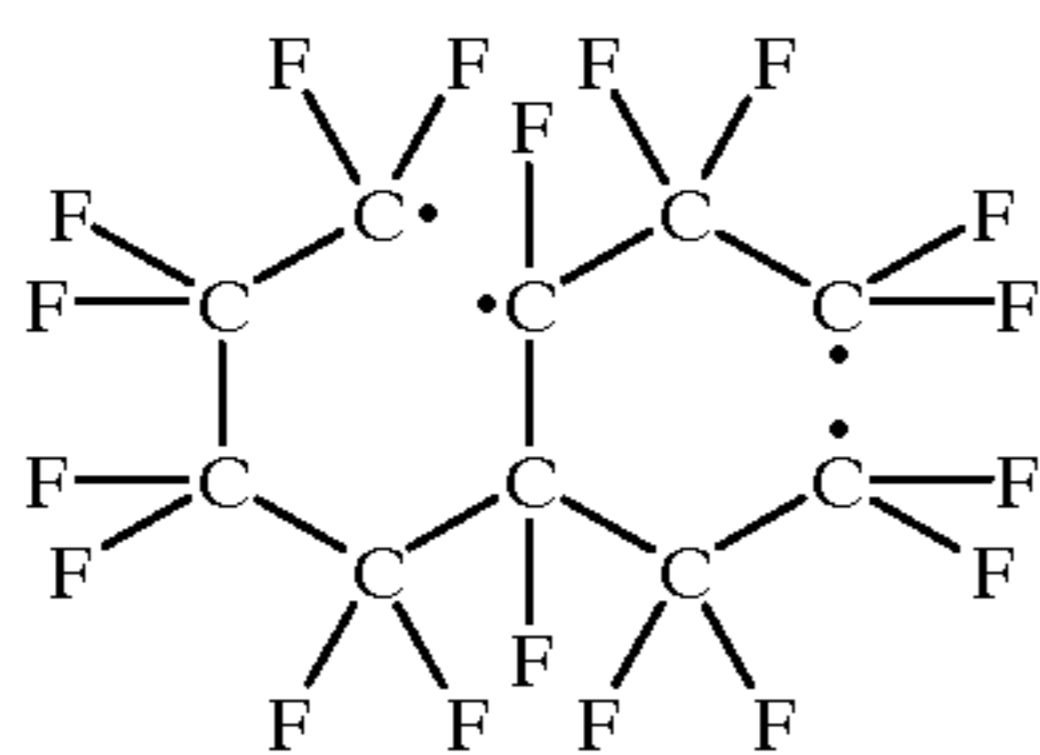
Chemical Formula 8
