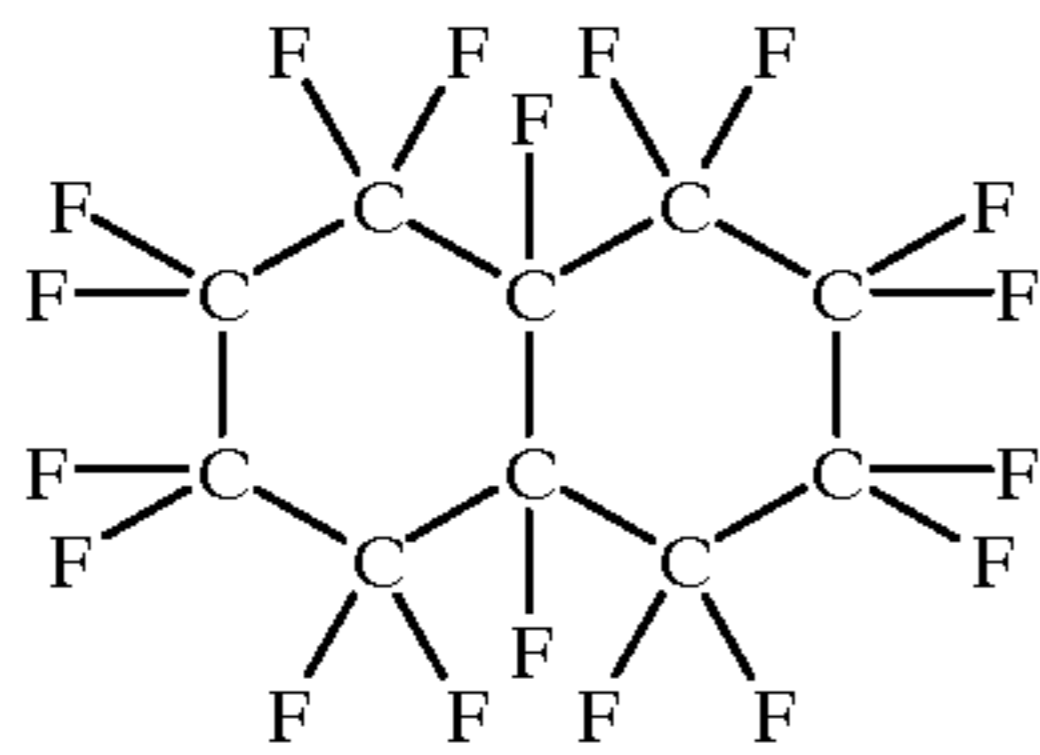
Chemical Formula 7
