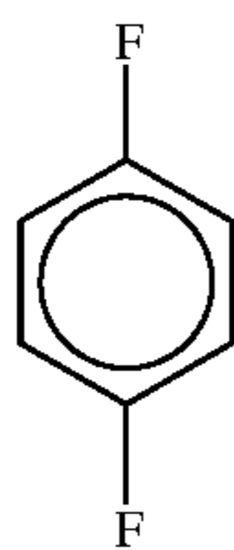
Chemical Formula 13
