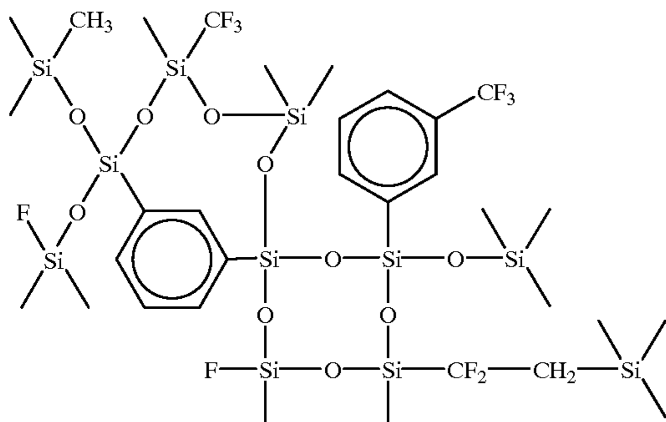
Chemical Formula 15
