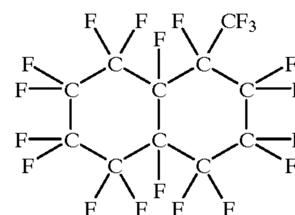
Chemical Formula 10
