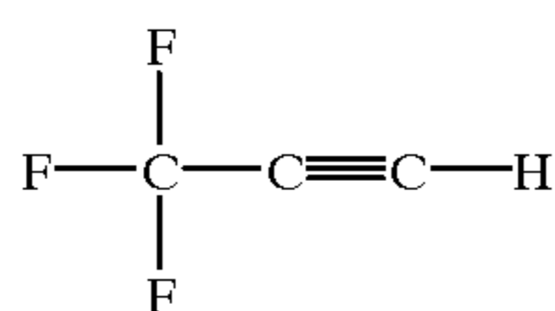
Chemical Formula 5
