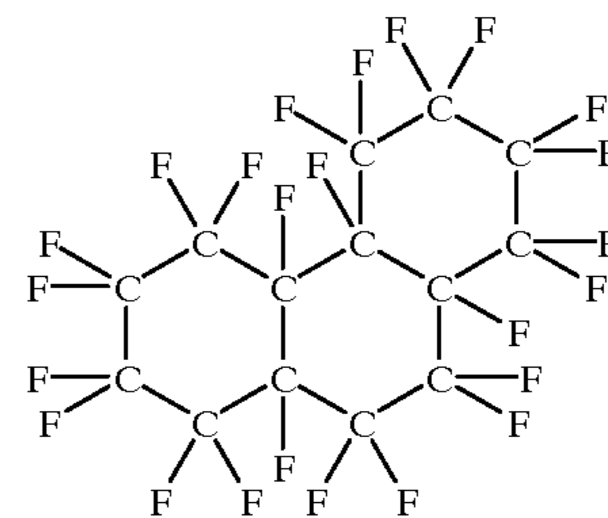
Chemical Formula 11
