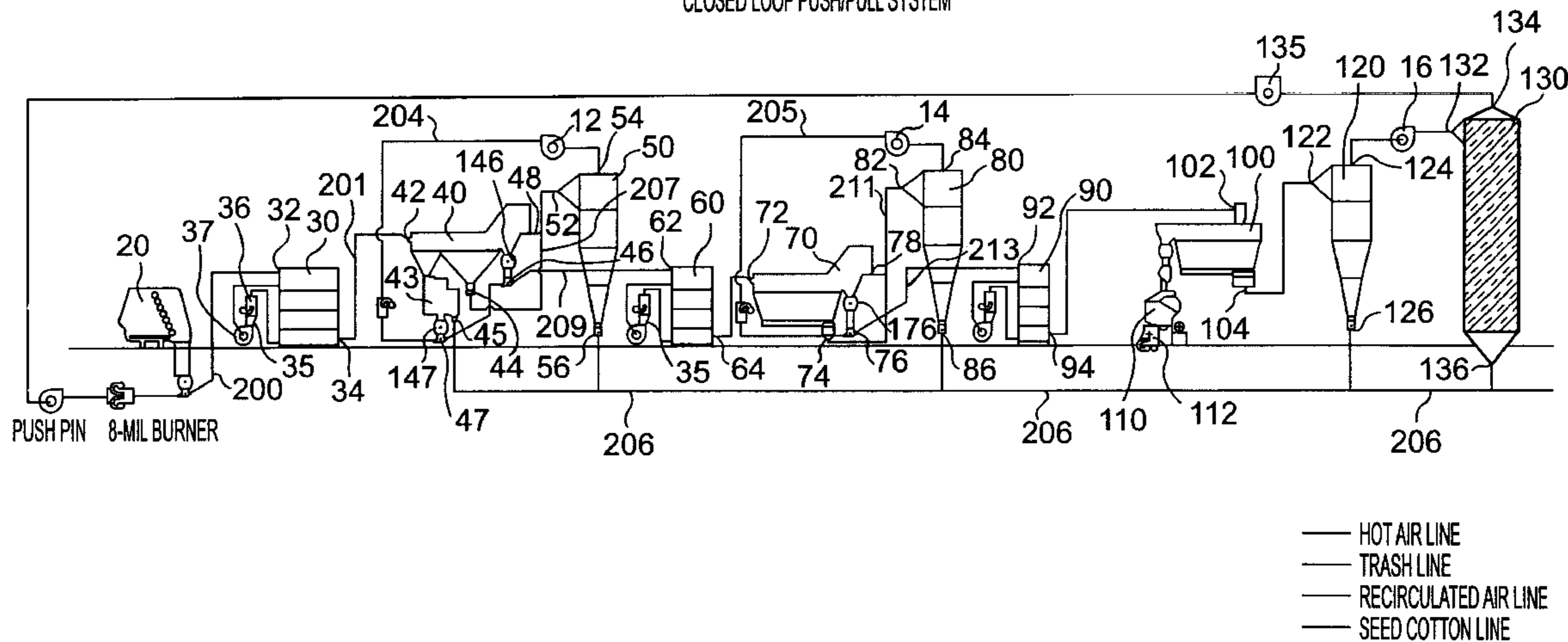
CLOSED LOOP PUSH/PULL SYSTEM
