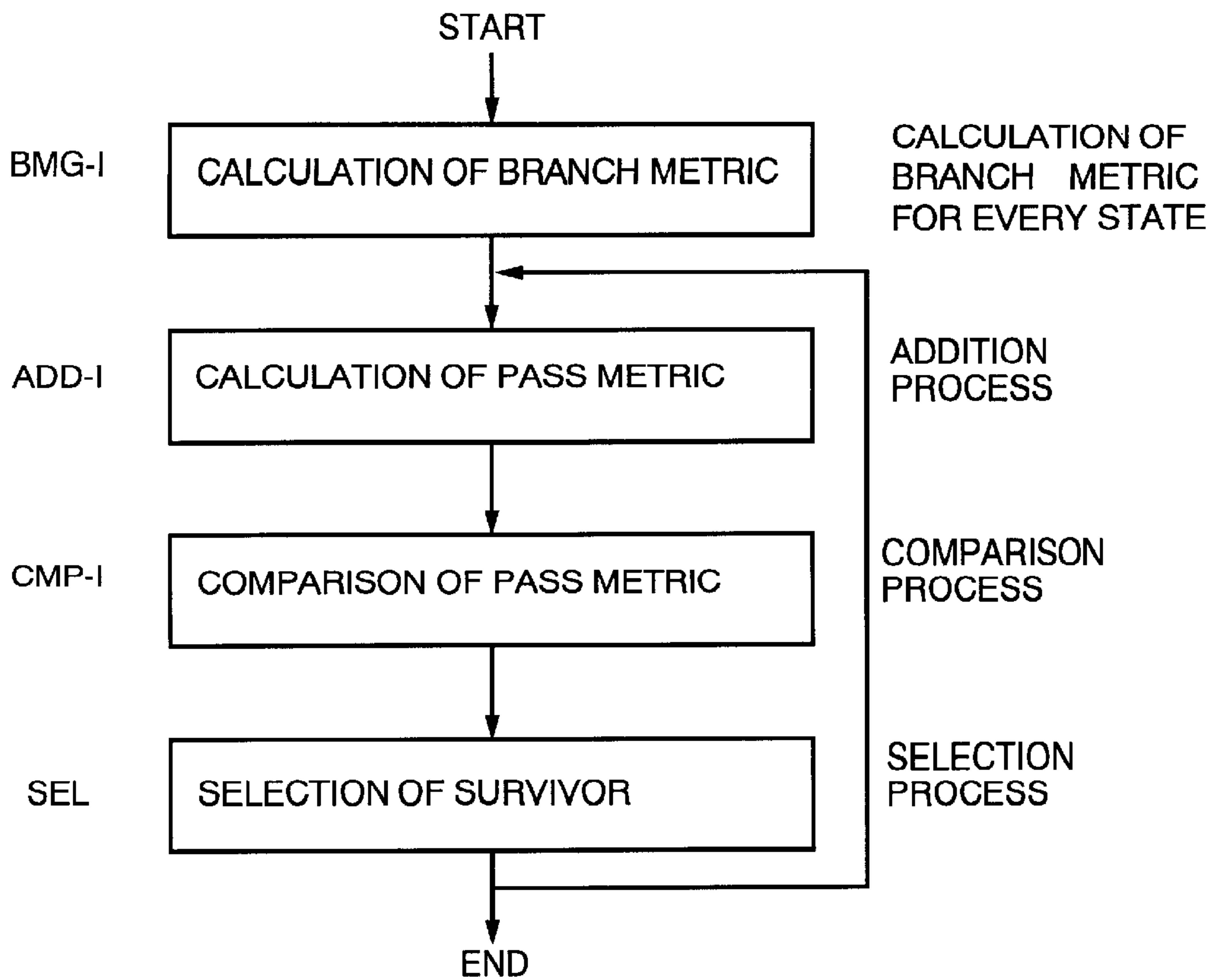
FIG. 20 (PRIOR ART)
