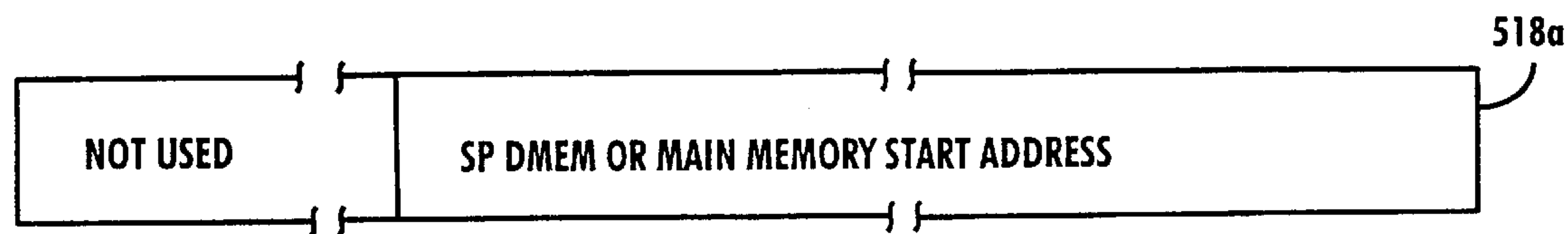
Fig. 21A DP CMD DMA START ADDRESS REGISTER (R/W)
