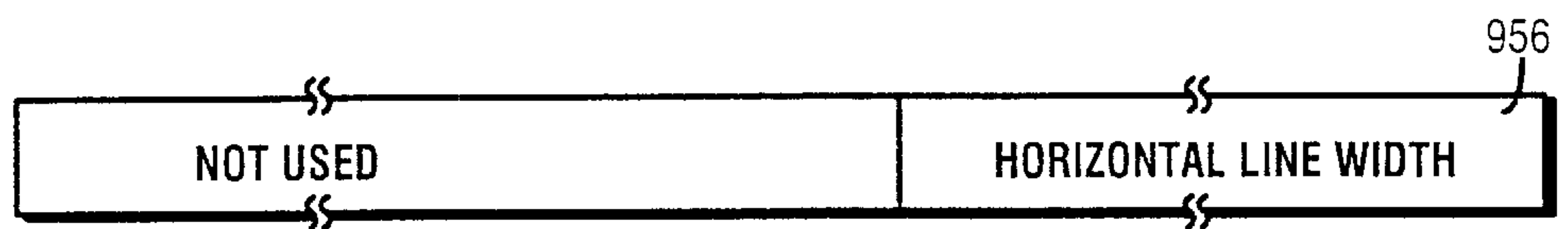
Fig. 35C VIDEO INTERFACE LINE WIDTH REGISTER (R/W)
