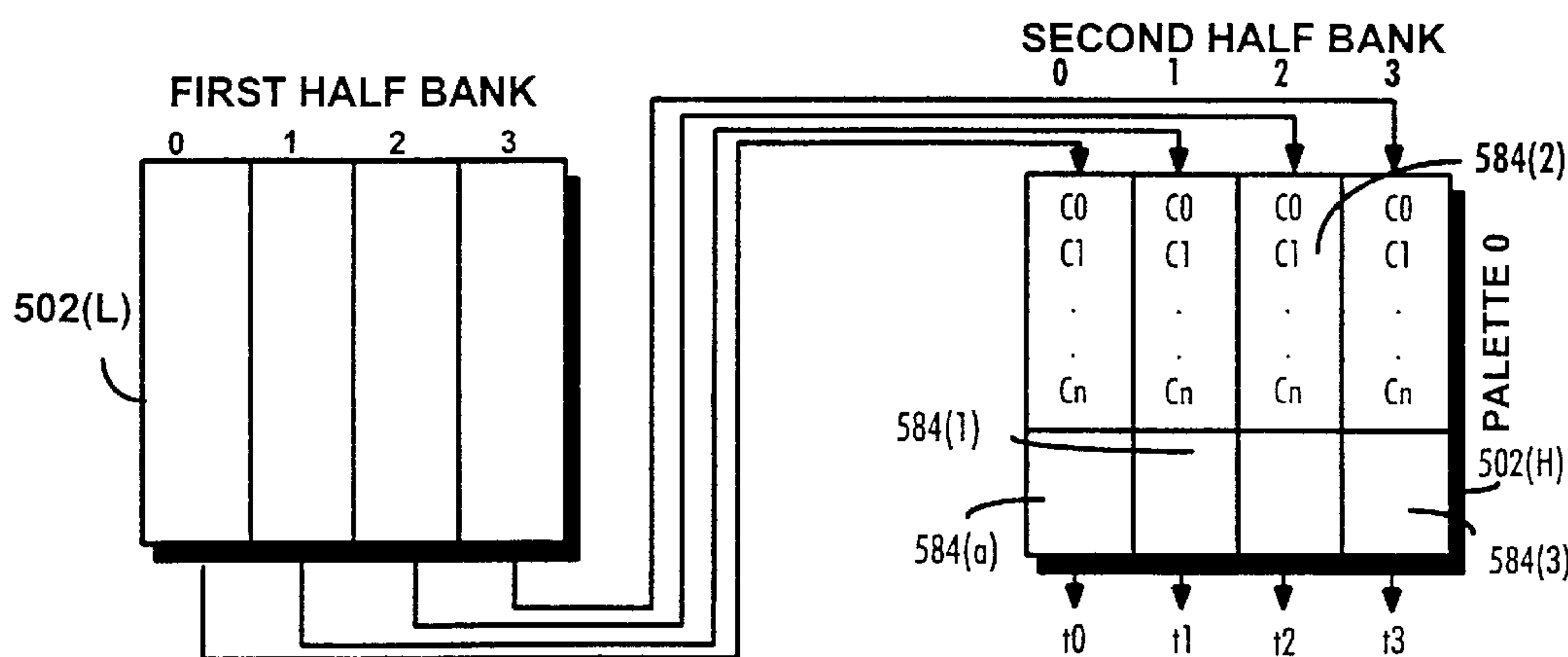
Fig. 25 TEXTURE MEMORY STORING COLOR INDEXED TEXTURES
