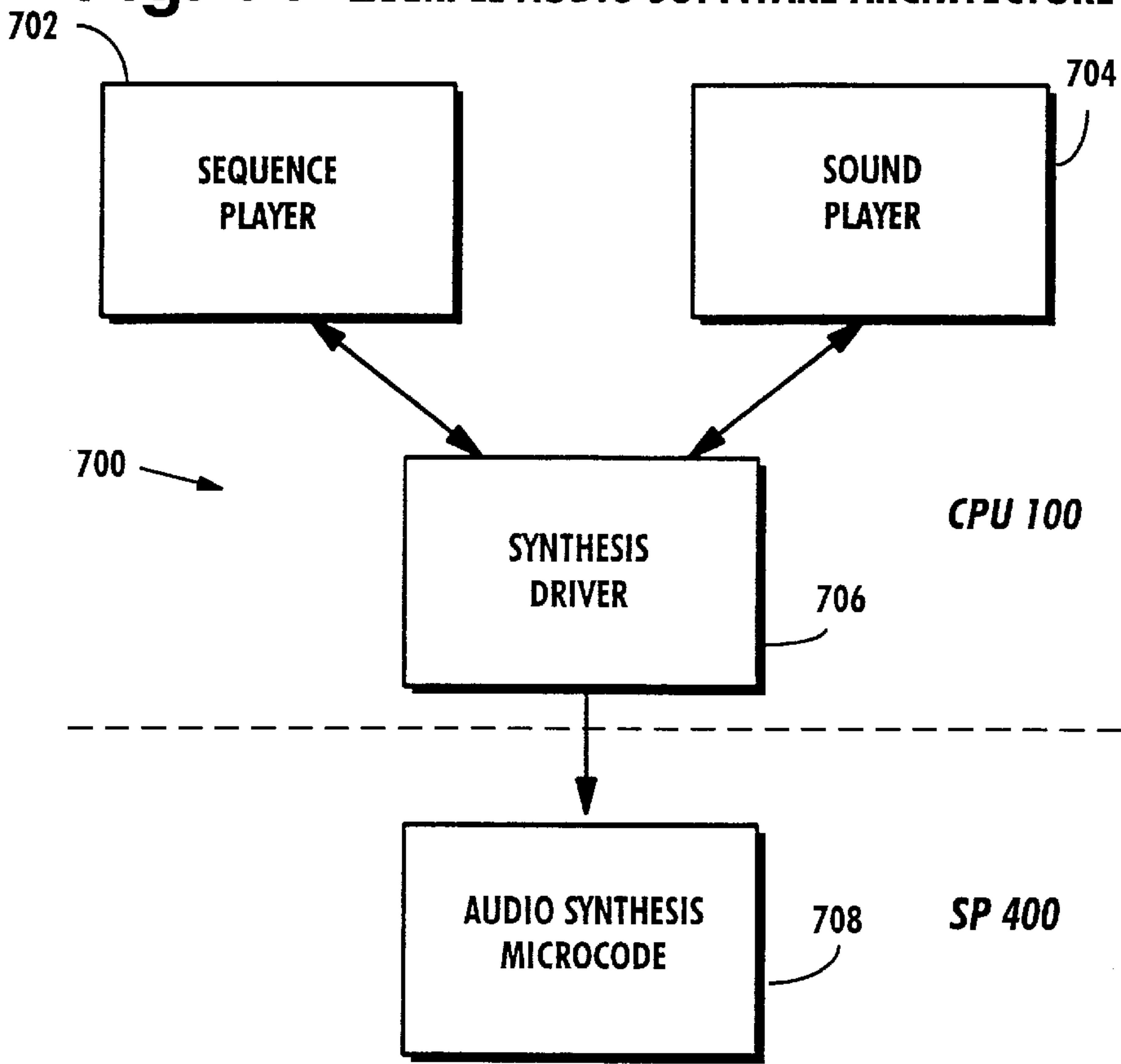
Fig. 14 EXAMPLE AUDIO SOFTWARE ARCHITECTURE
