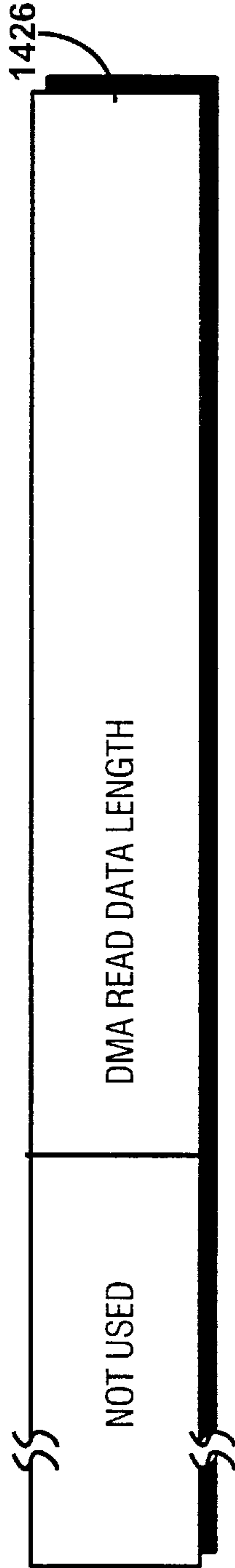
Fig. 45C PI DMA READ LENGTH (R/W)
