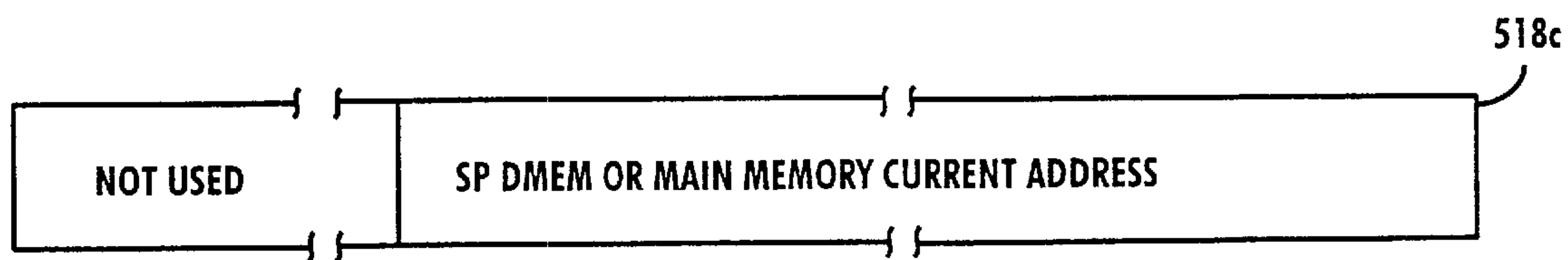
Fig. 21C DP CMD DMA CURRENT ADDRESS REGISTER (R/W)
