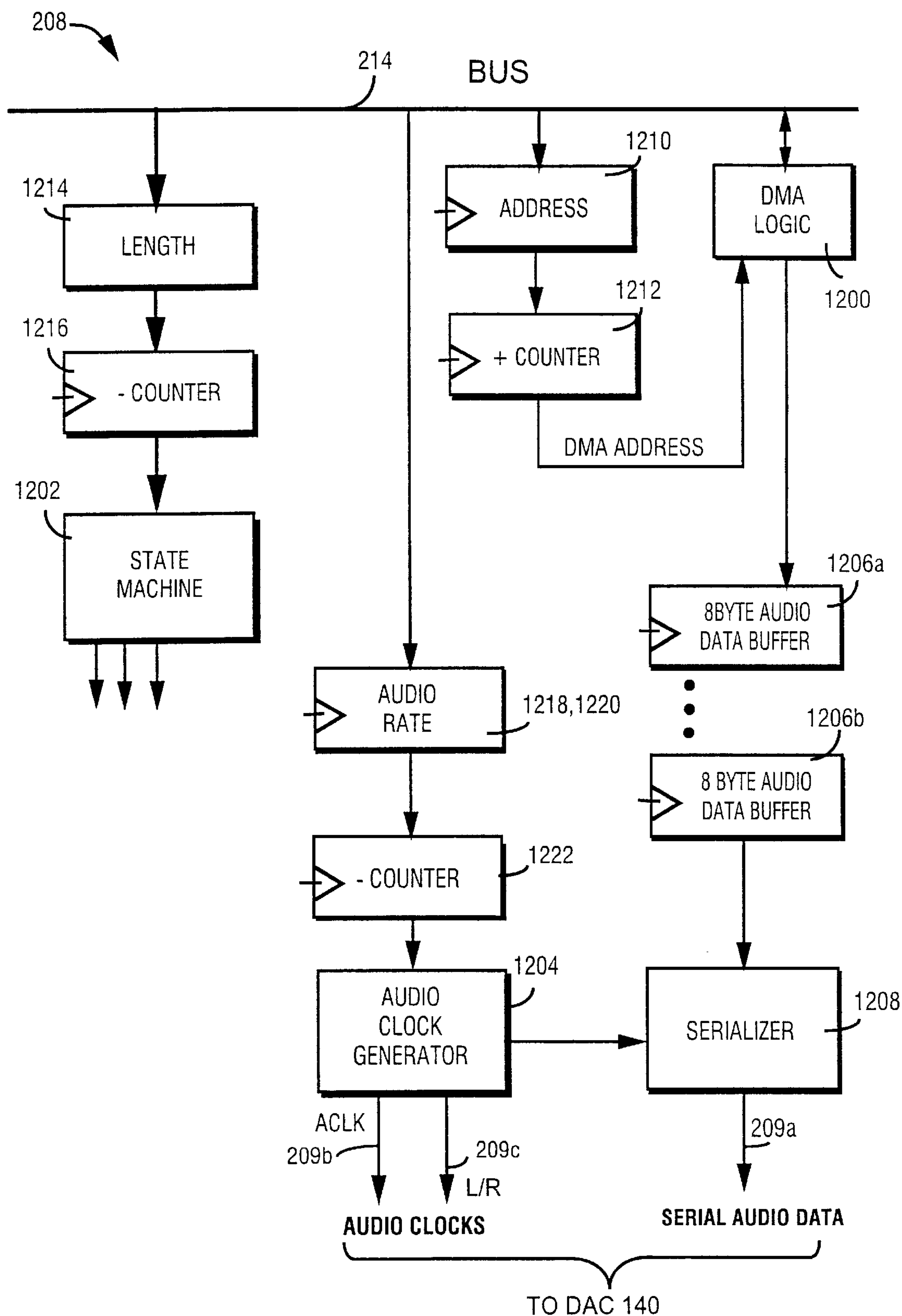
Fig. 40 EXAMPLE AUDIO INTERFACE ARCHITECTURE
