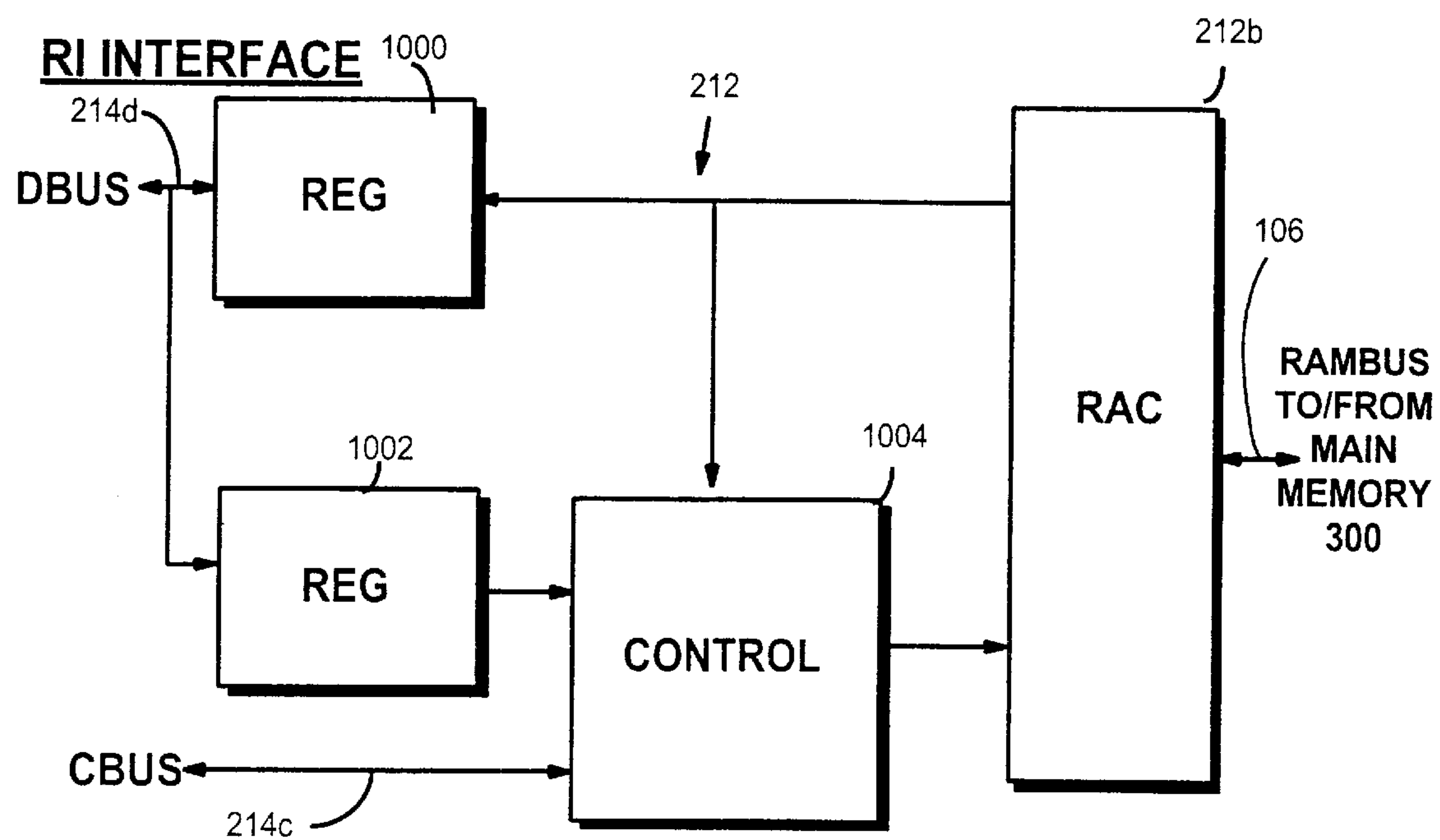
Fig. 36 EXAMPLE MEMORY INTERFACE
