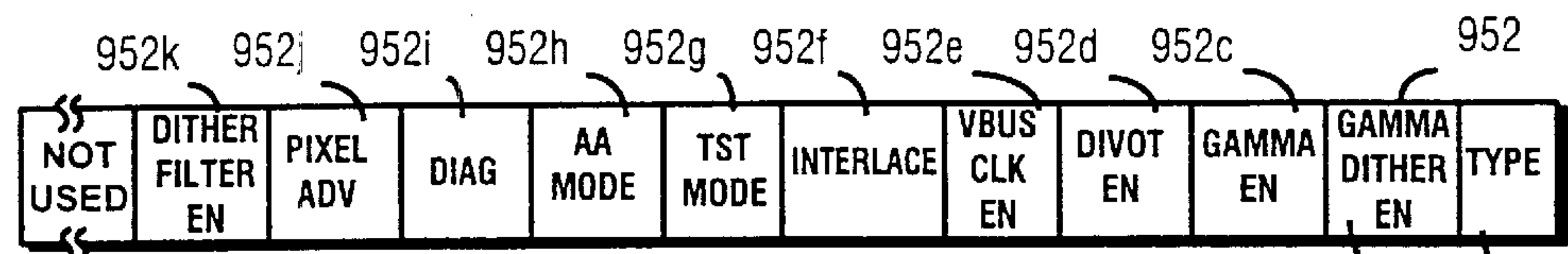
Fig. 35A VIDEO INTERFACE CONTROL REGISTER (R/W)
