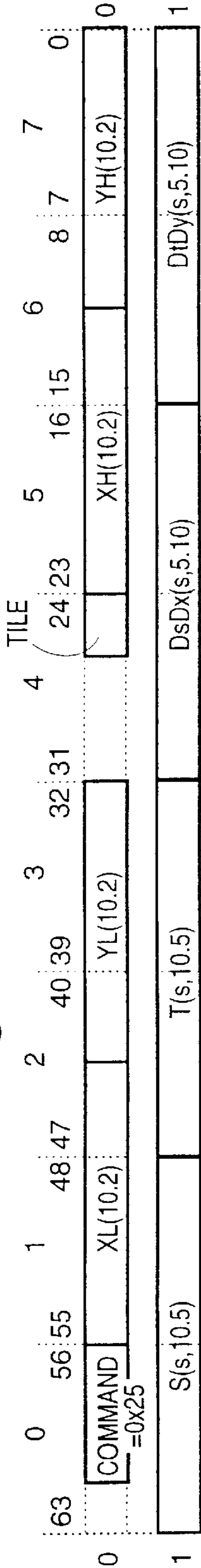
Fig. 81 Texture Rectangle Flip
