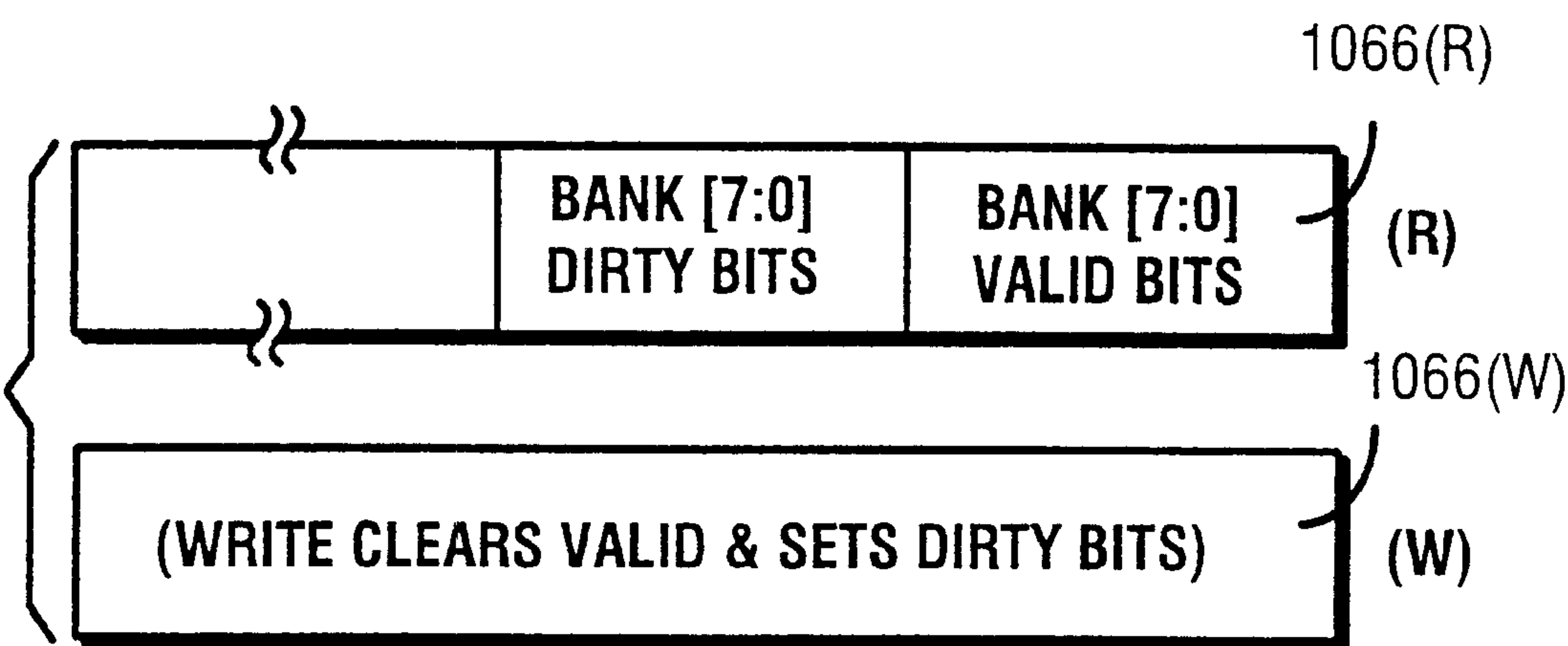
Fig. 37H BANK STATUS REG
