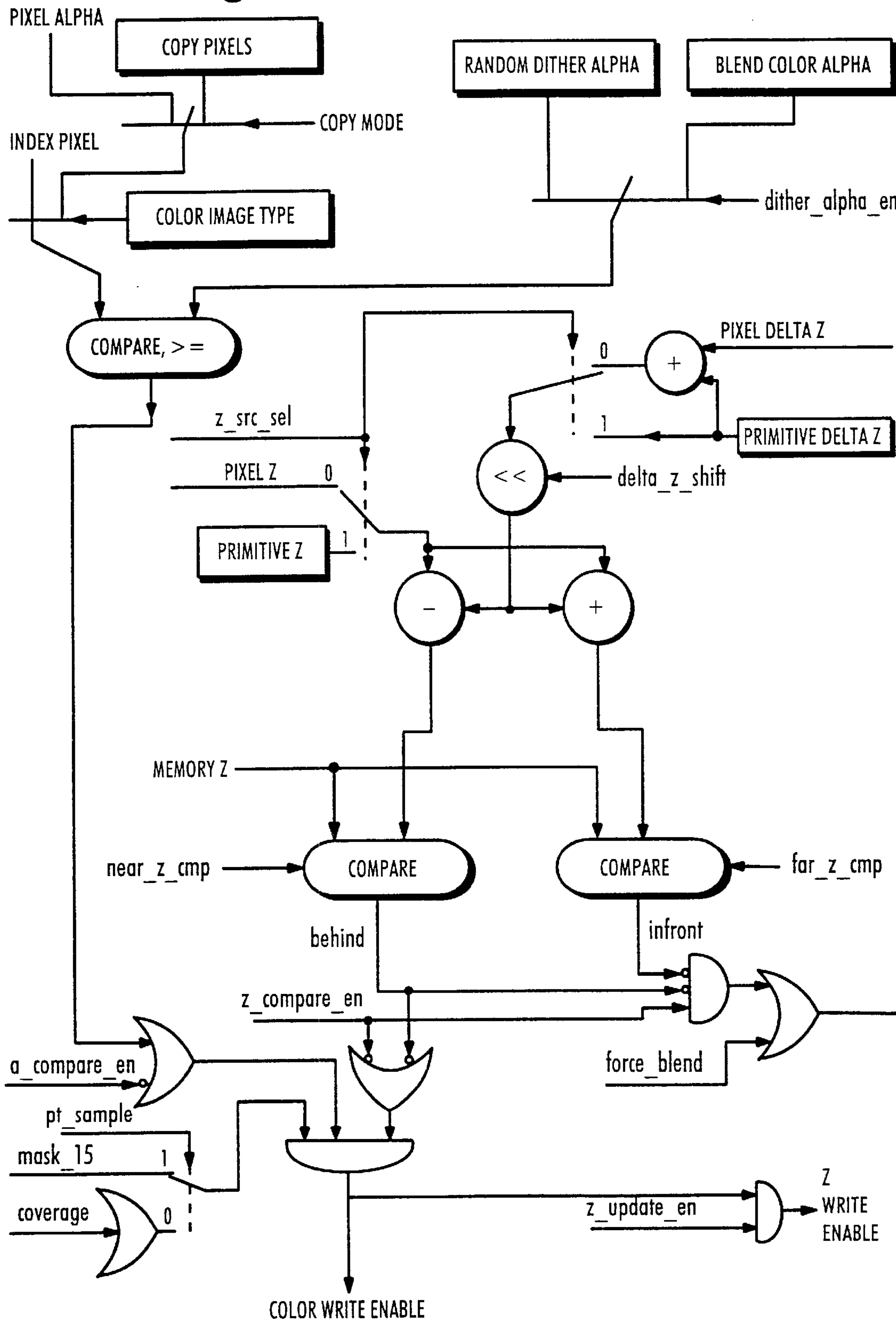
Fig. 33A WRITE ENABLE GENERATION
