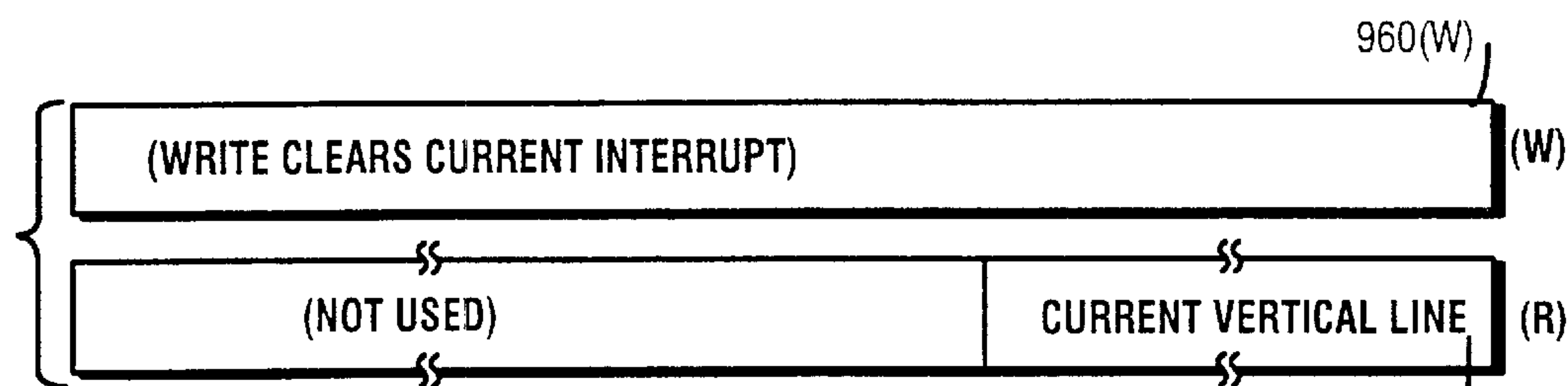
Fig. 35E VIDEO INTERFACE CURRENT LINE REGISTER
