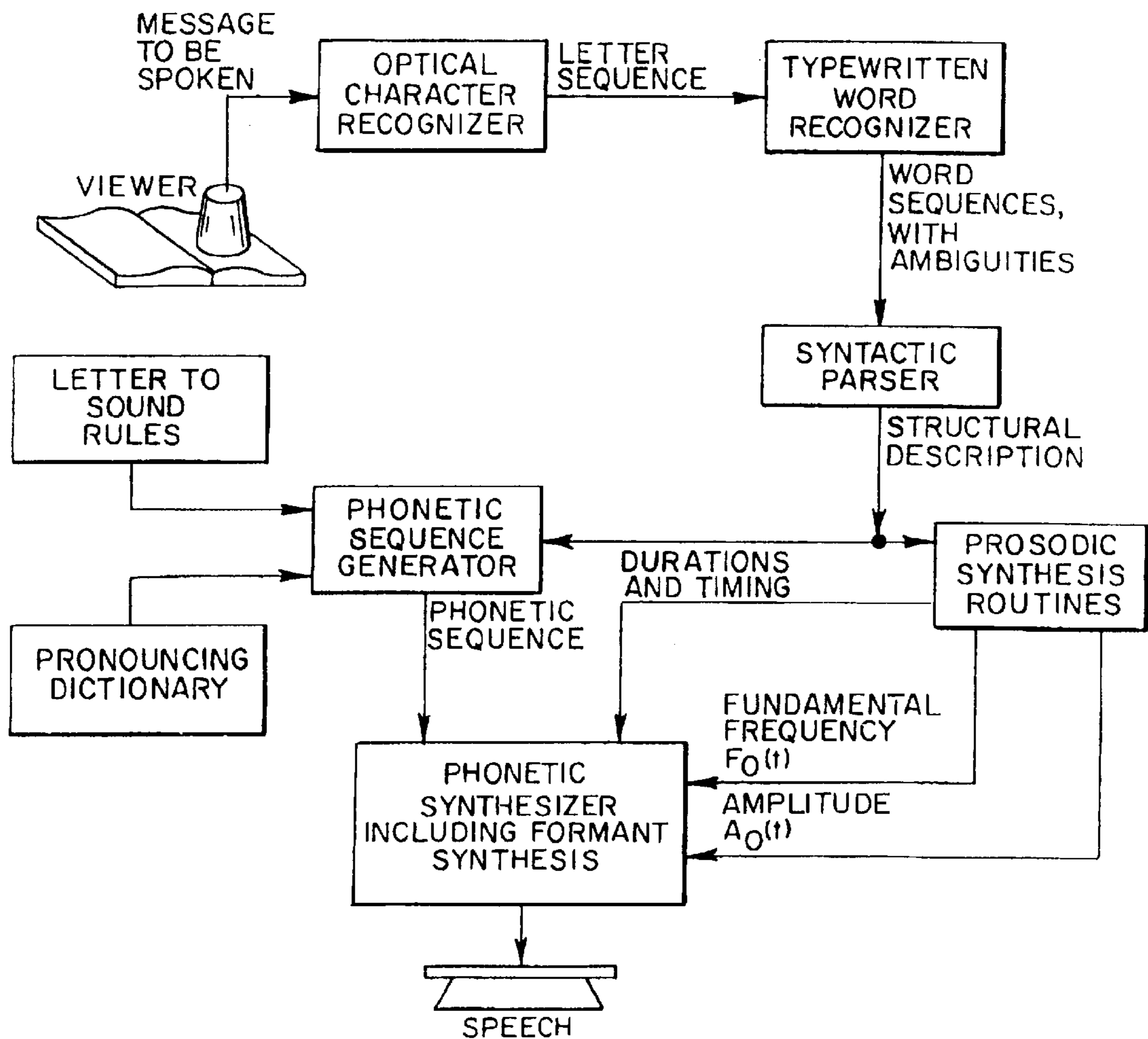
TEXT TO SPEECH SYSTEM FOR GENERATING COMPLEX SENTENCES WITH LARGE VOCABULARIES
