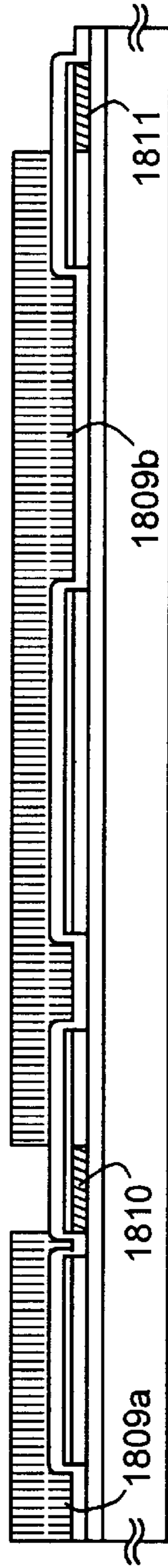
FIG. 18D STEP OF ADDING N-TYPE IMPURITY
