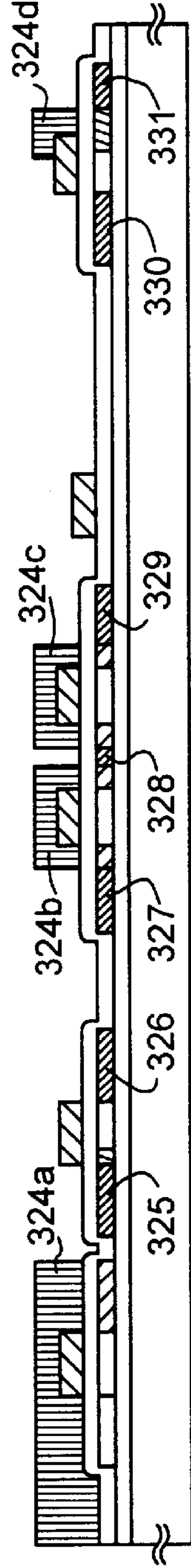
FIG. 5B STEP OF ADDING N-TYPE IMPURITY
