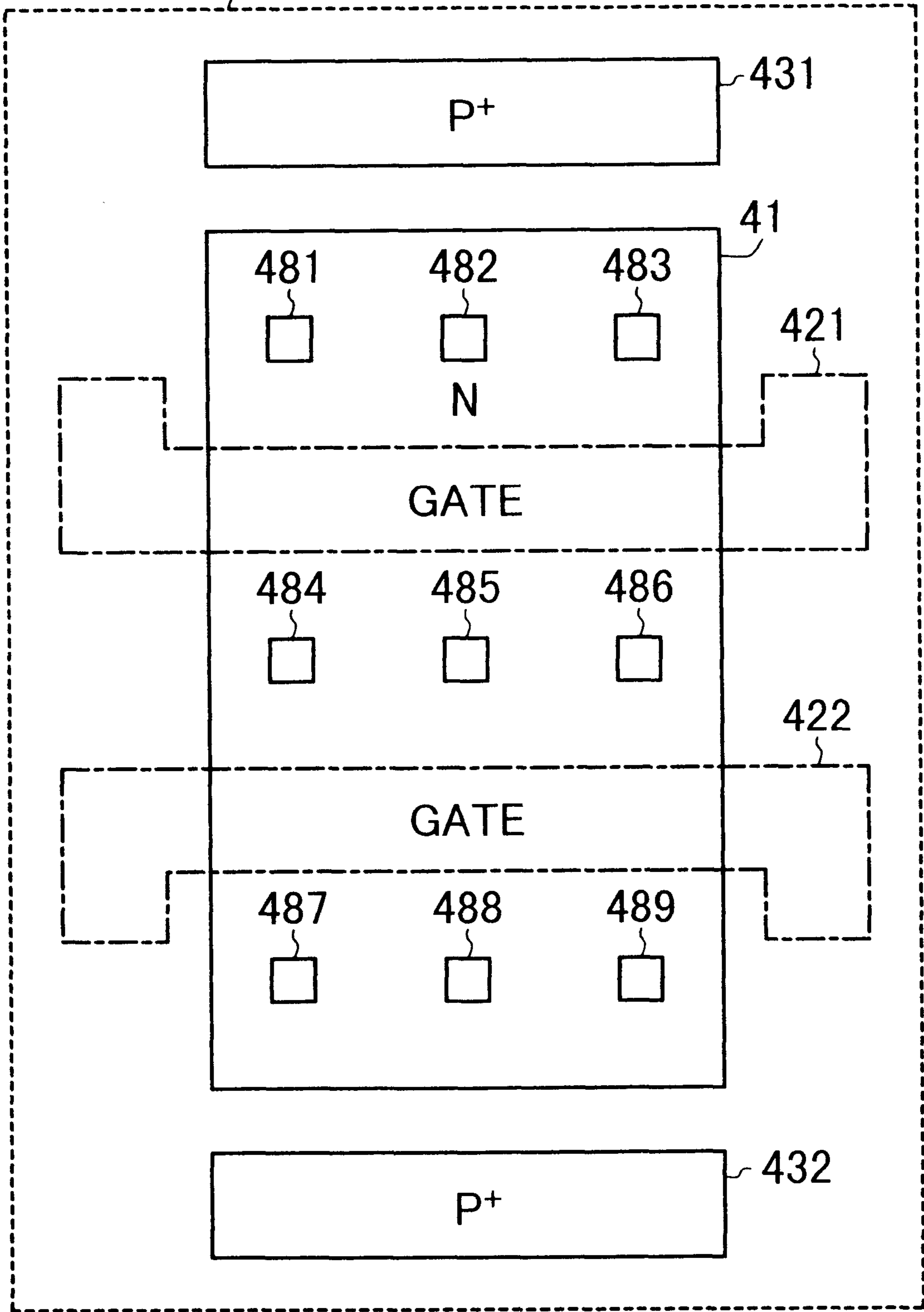
40 BASIC CELL PTRN
