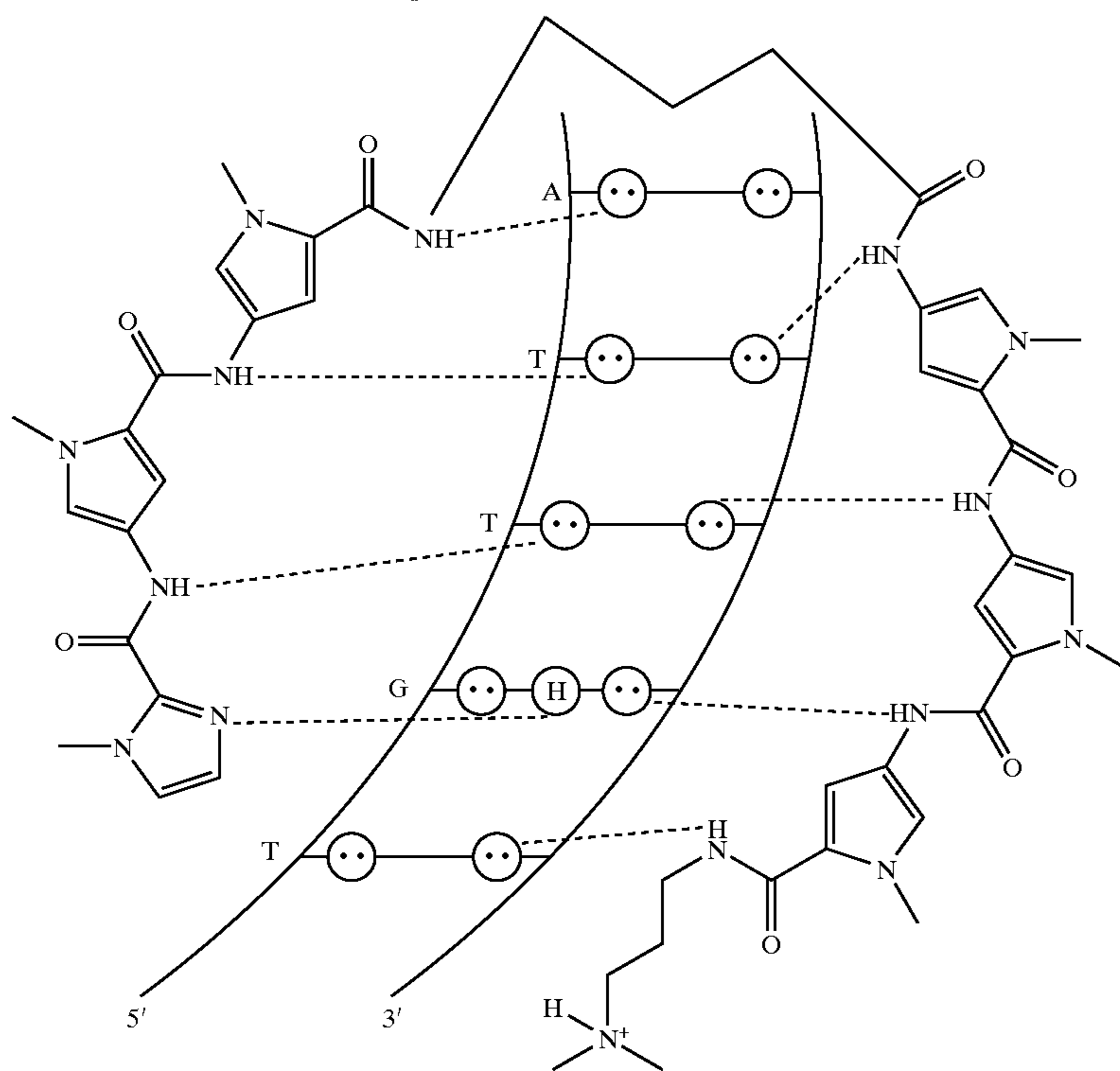
ImPyPy- \gamma -PyPyPy-Dp•TGTTA K_a = 8 \times 10^7 \text{ M}^{-1}
