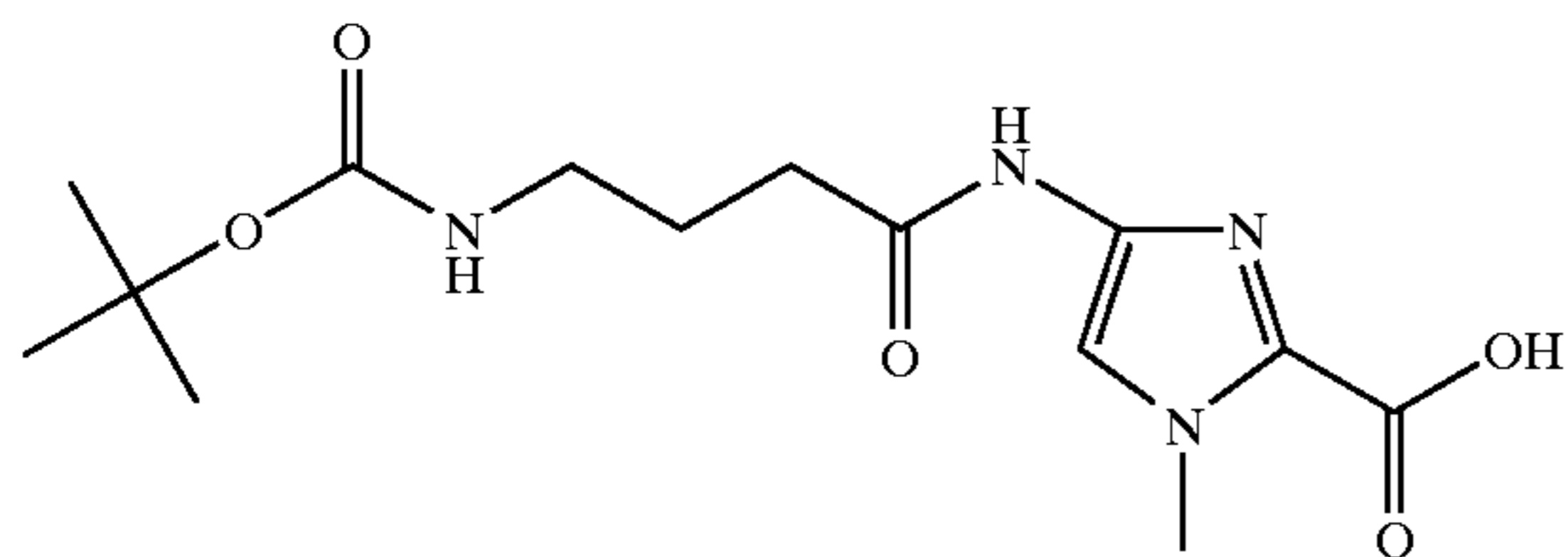
10. γ-[(tert-butoxycarbonyl)amino]-butyric acid-(4-carboxamido-1-methyl-imidazole)-2-carboxylic acid
