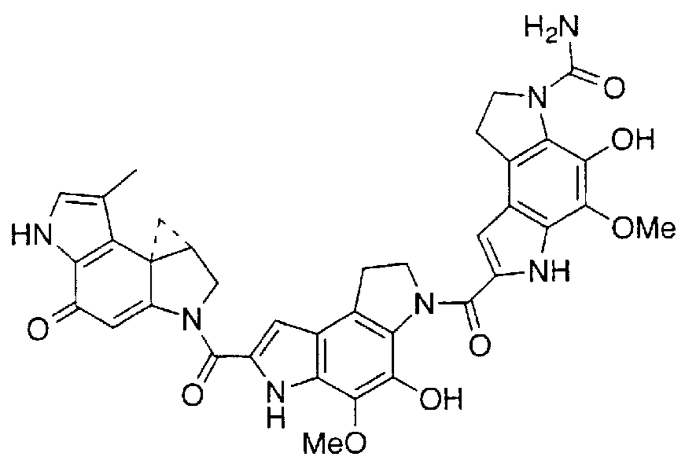
(+)- CC-1065
