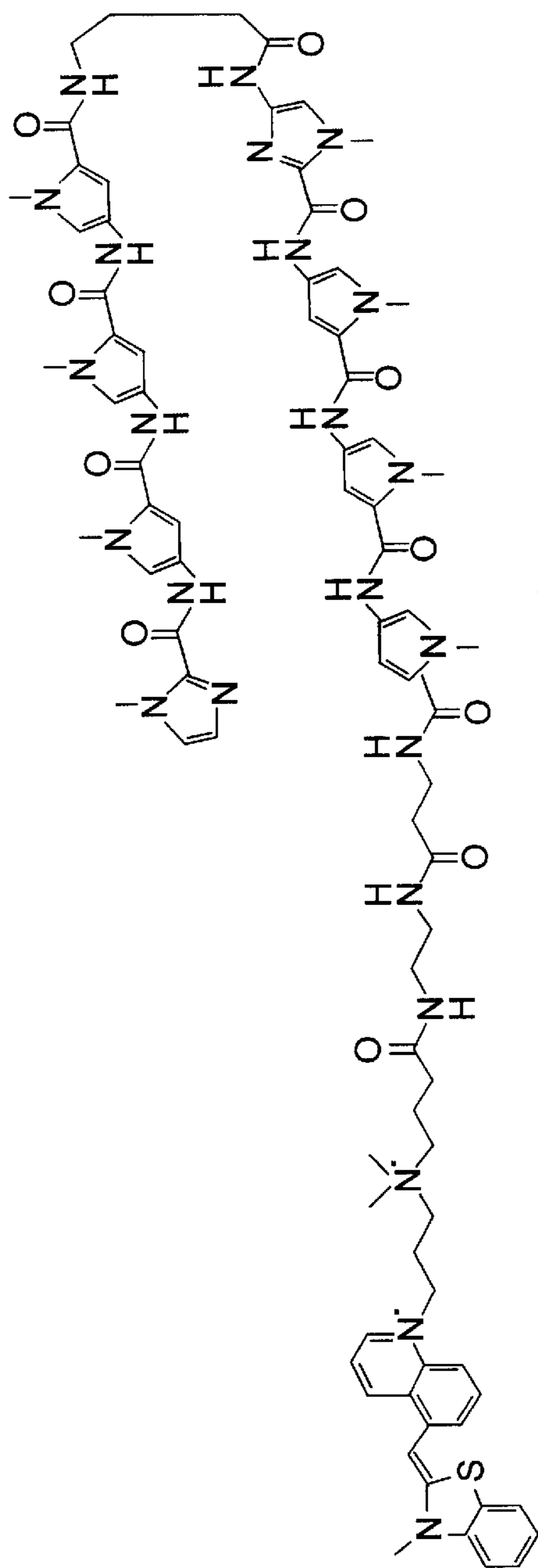
ImPyPyPy-β-ImPyPyPy-β-ED-TO
