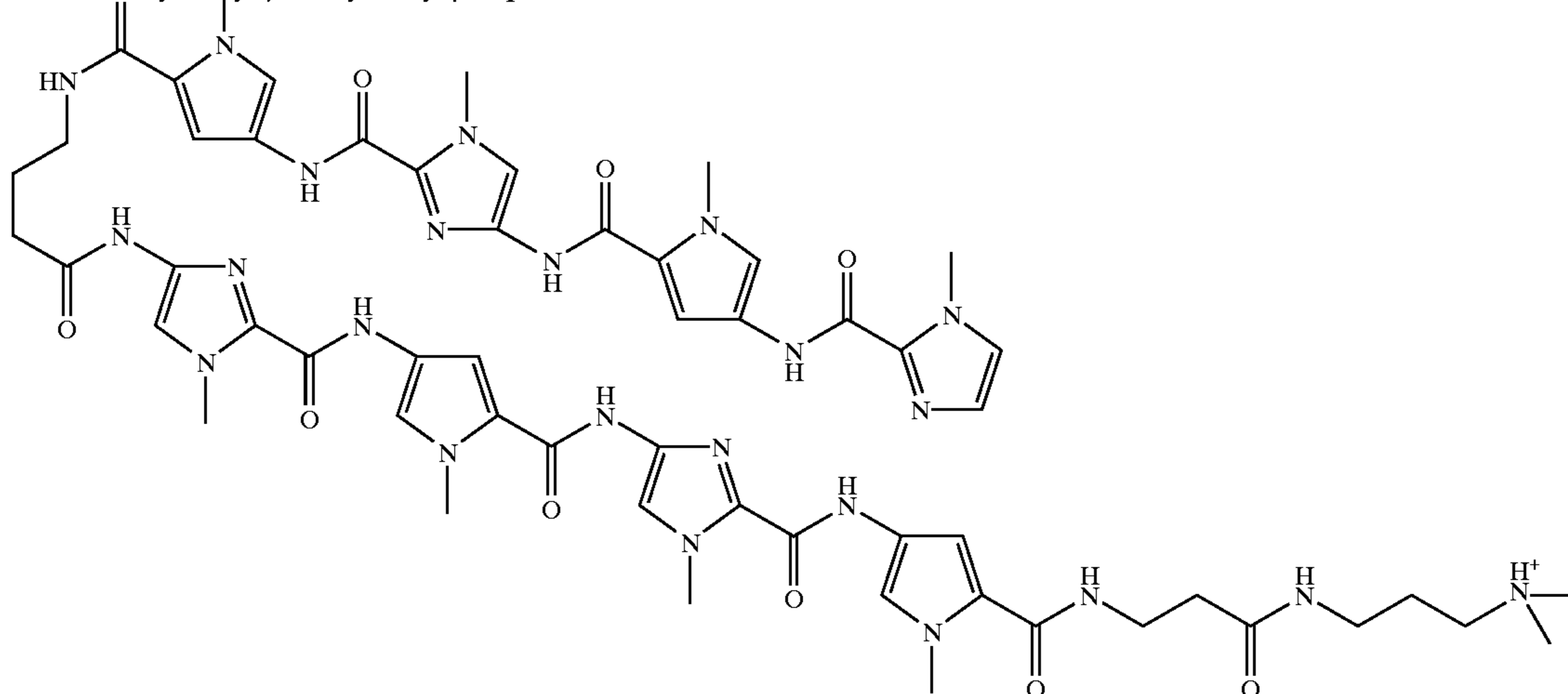
51. ImPyImPy- \gamma -ImPyImPy- \beta -Dp
