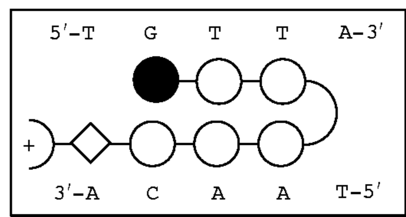
ImPyPy- \gamma -PyPyPy- \beta -Dp \cdot 5'-TGTTA-3'
