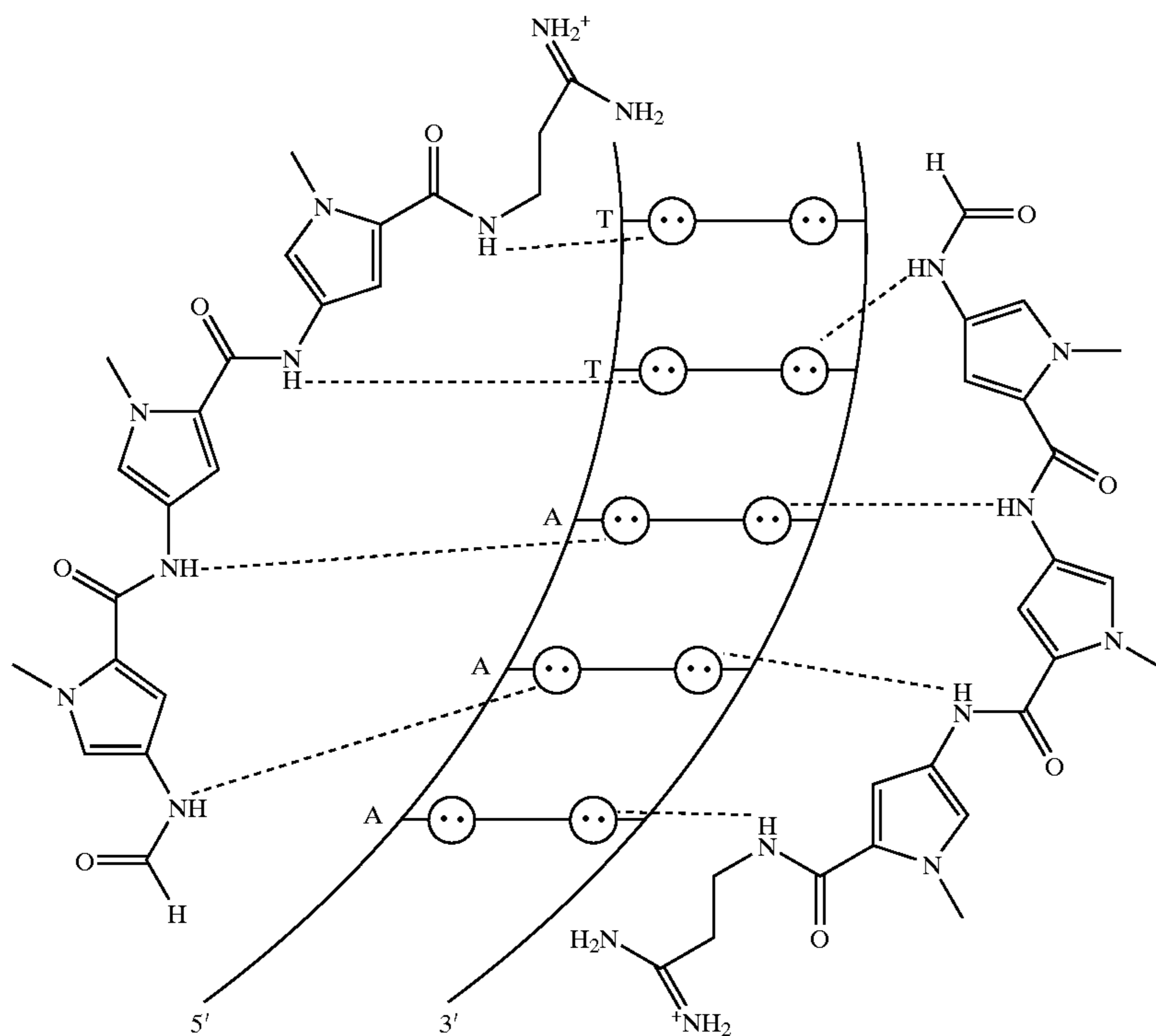
1:1 Distamycin•DNA Complex
