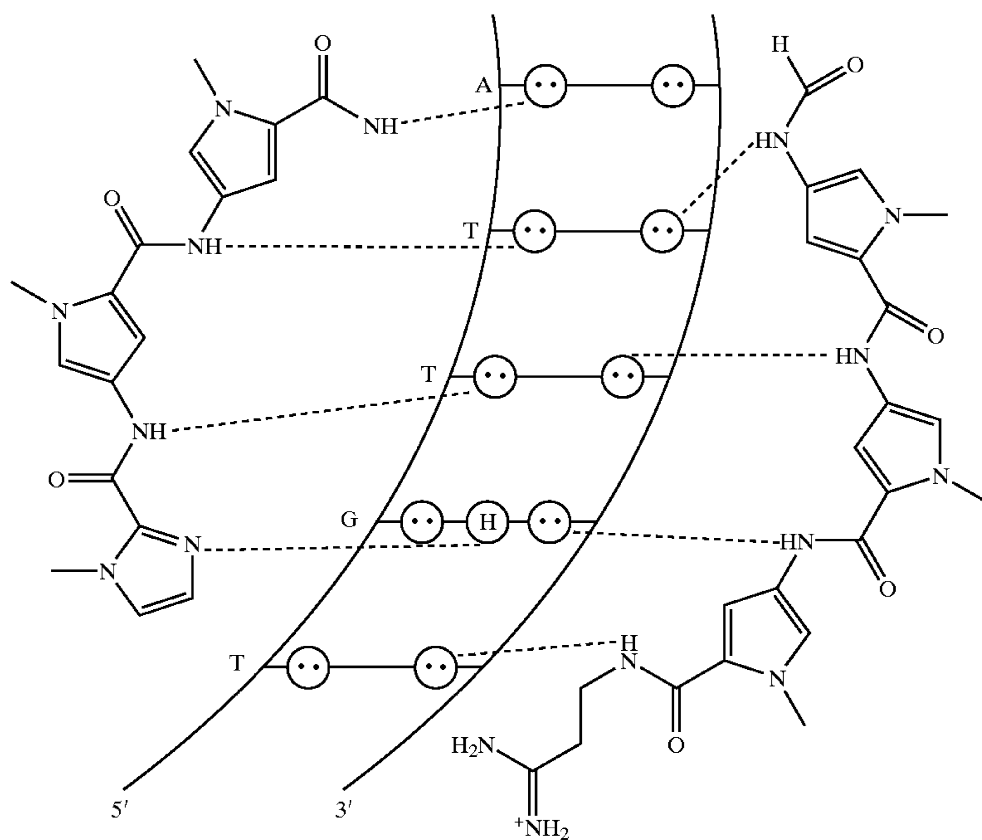
ImPyPy-Dp/PyPyPy•TGTTA K_a \sim 2 \times 10^5 \text{ M}^{-1}
