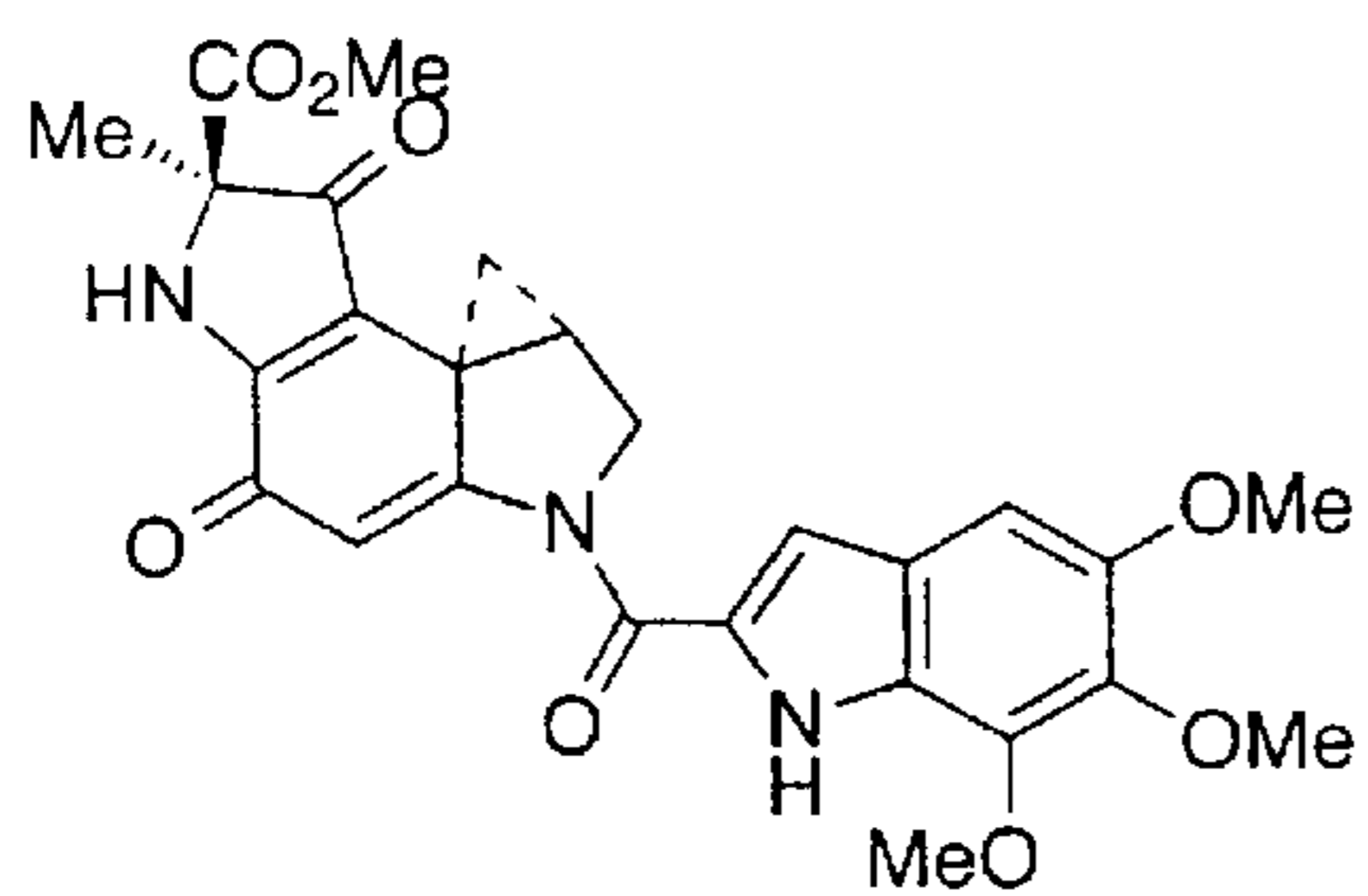
(+)- Duocarmycin A
