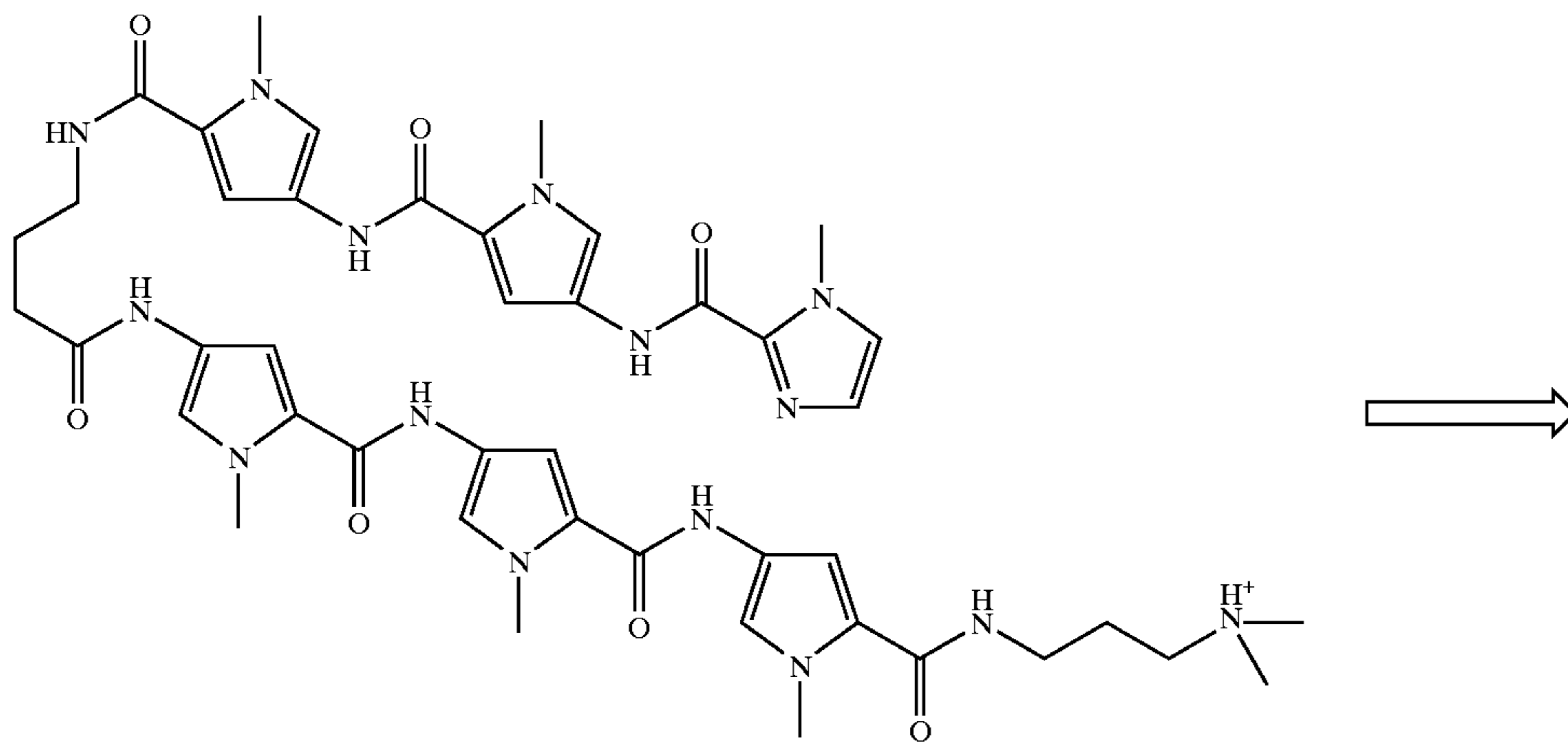
ImPyPy- \gamma -PyPyPy-Dp K_8 = 7 \times 10^7 \text{ M}^{-1} specificity: 24-fold
