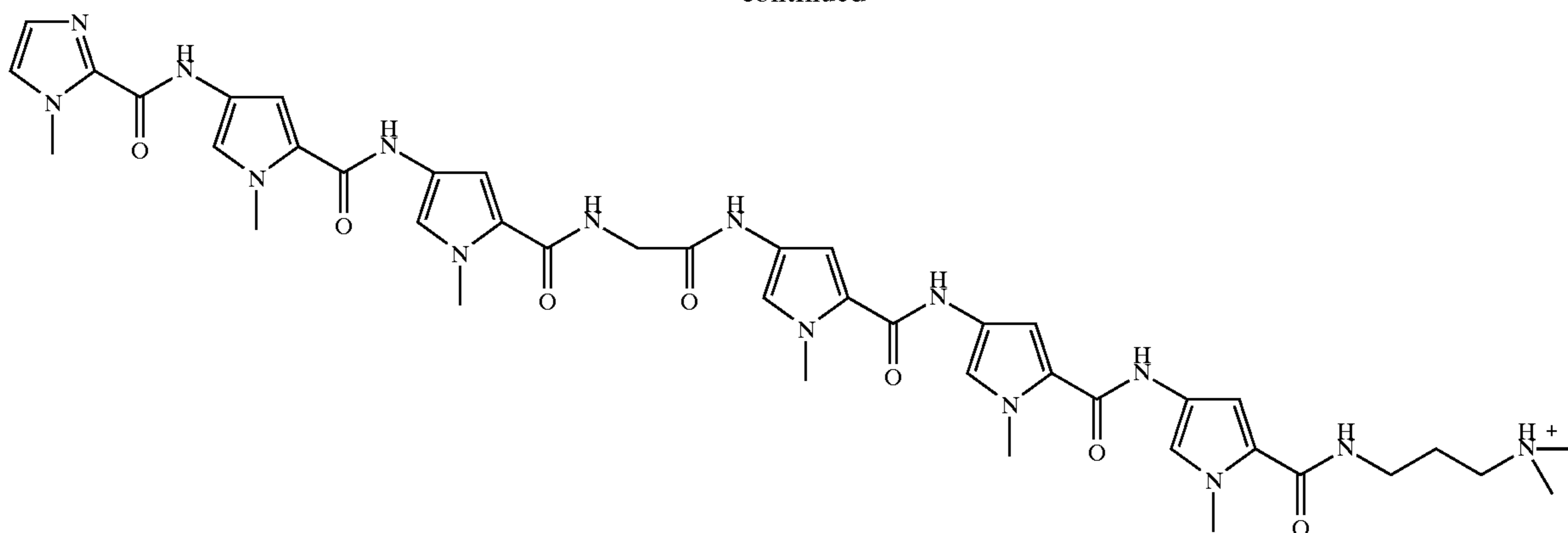
ImPyPy-G-PyPyPy-Dp
