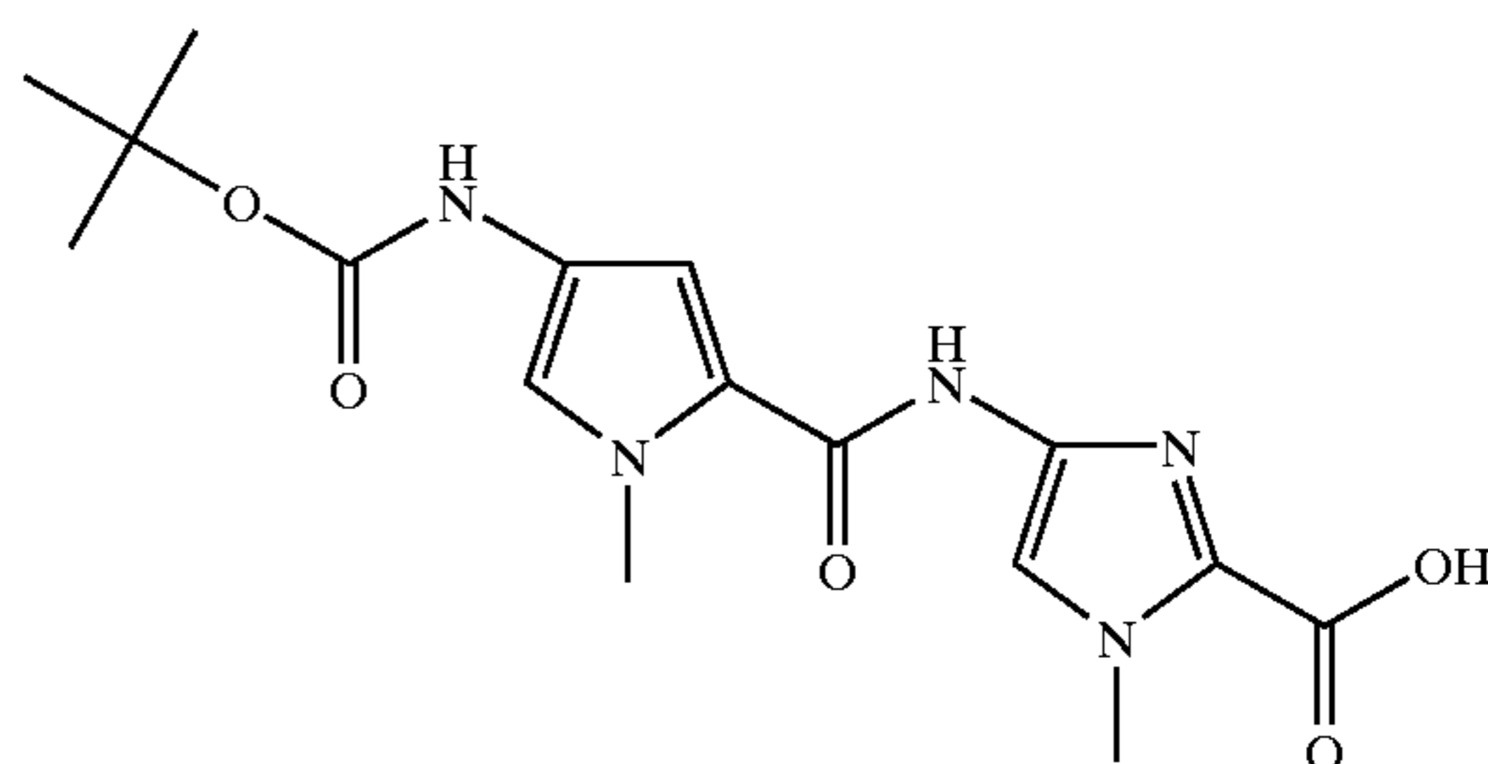
11. 4-[(tert-butoxycarbonyl)amino]-1-methylpyrrole-2-(4-carboxamido-1-methyl imidazole)-2-carboxylic acid
