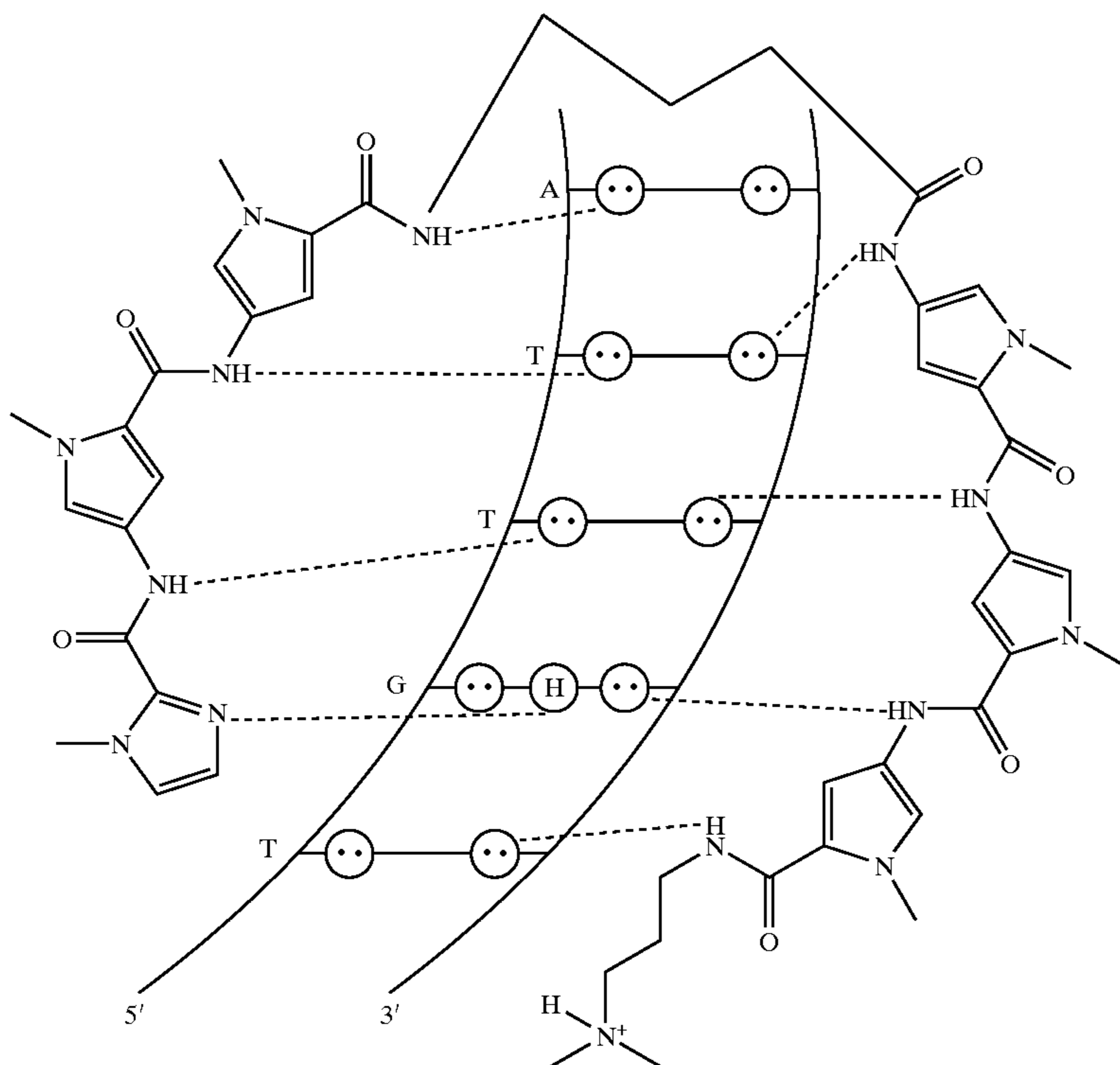
ImPyPy- \gamma -PyPyPy-Dp•5'-TGTTA-3' K_a = 7 \times 10^7 \text{ M}^{-1} specificity: 30-fold
