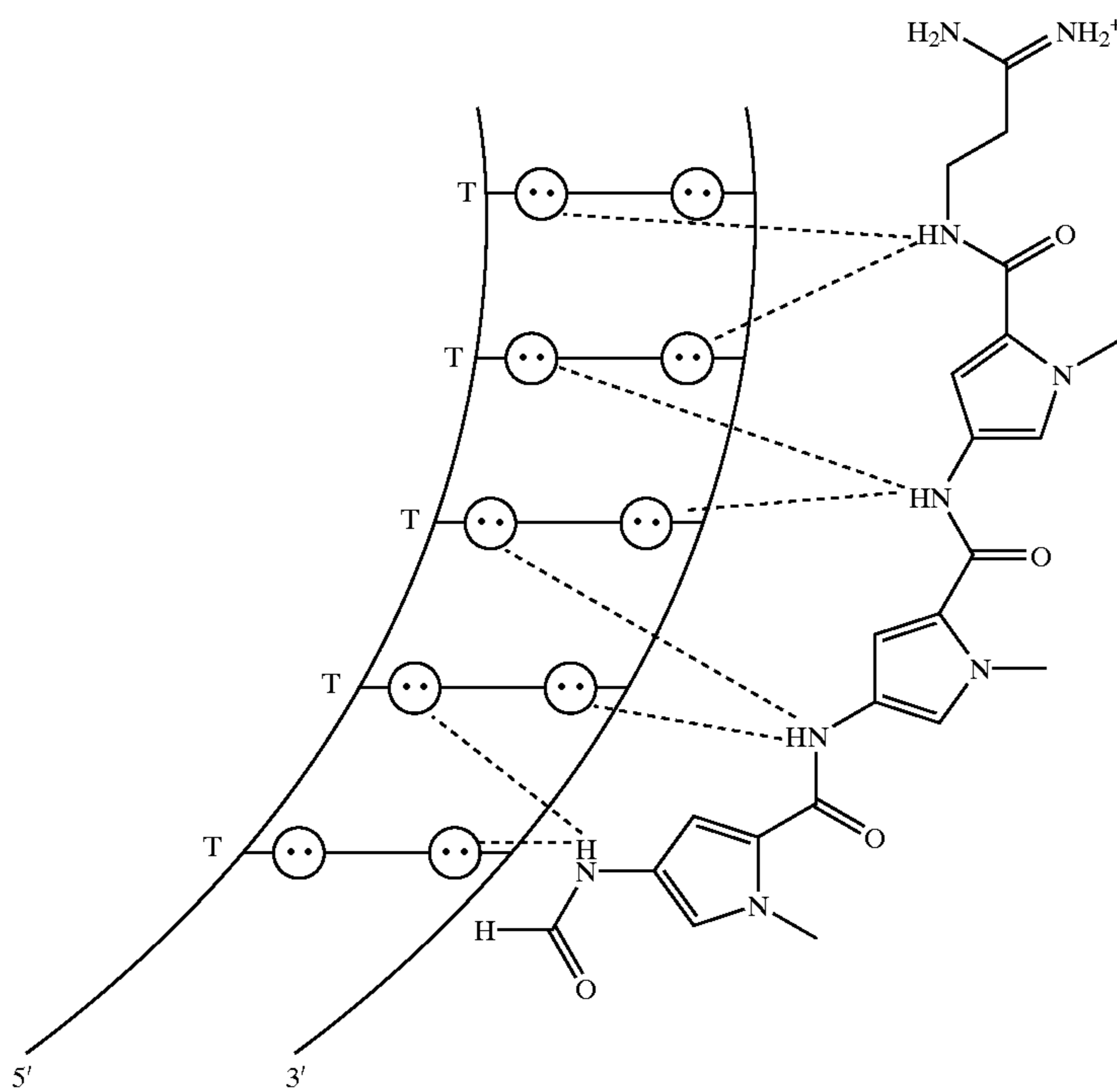
1:1 Distamycin•DNA Complex
