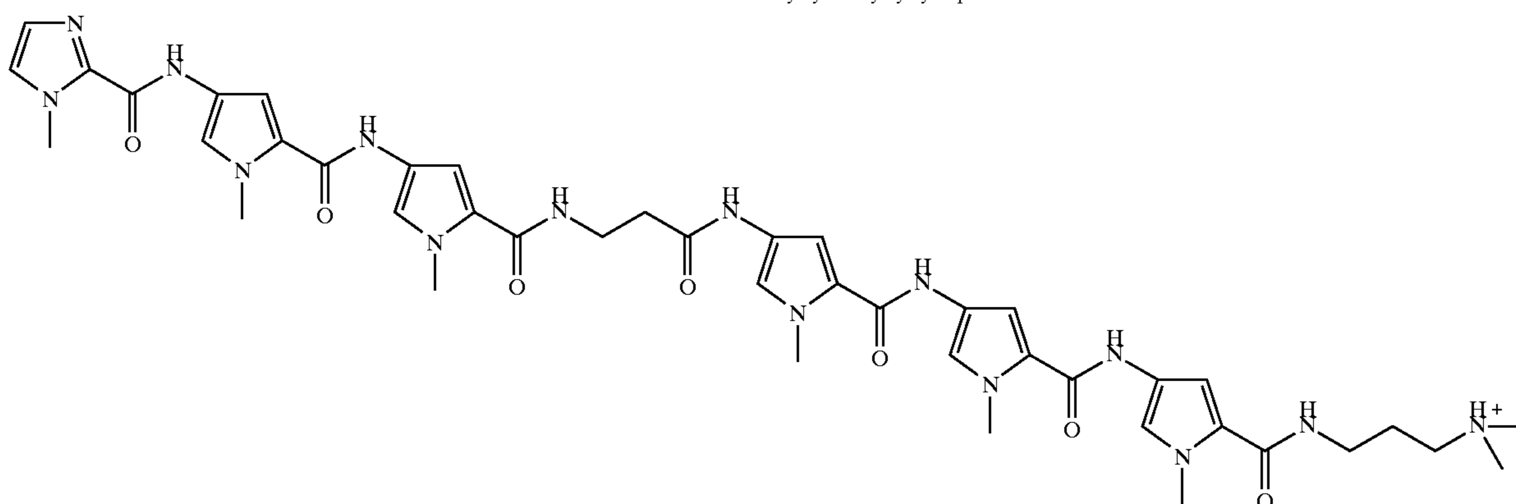
ImPyPy- \beta -PyPyPy-Dp
