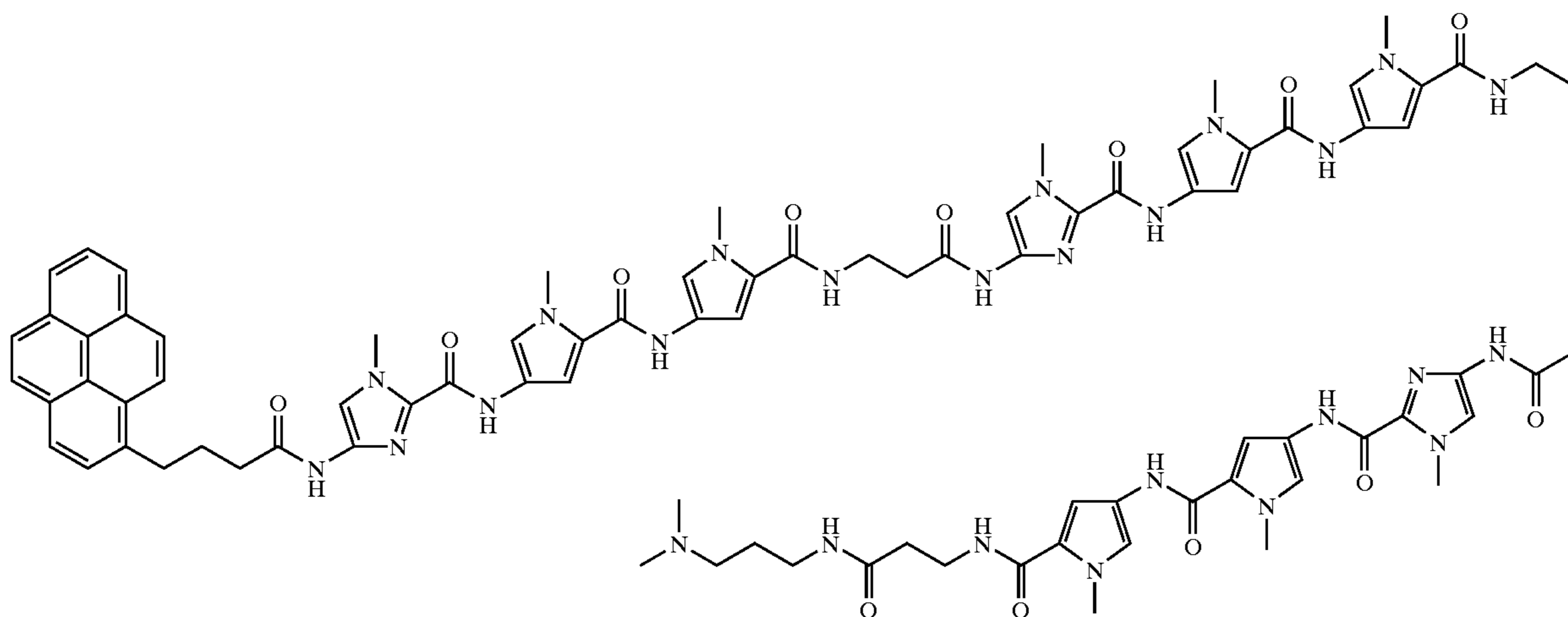
Pyrene-PyPyPy- \beta -ImPyPy- \gamma -ImPyPy- \beta -Dp
