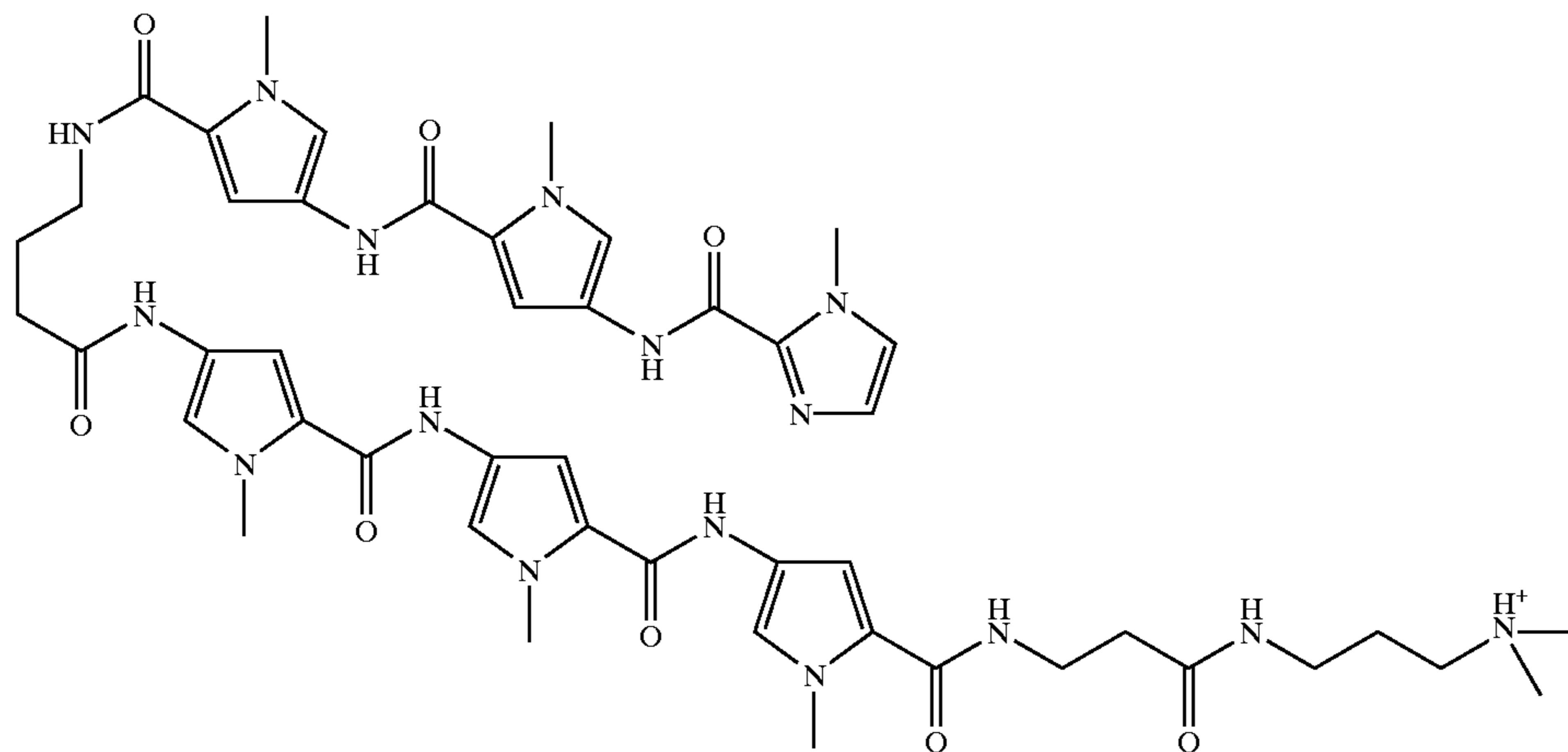
ImPyPy- \gamma -PyPyPy- \beta -Dp K_8 = 1 \times 10^8 \text{ M}^{-1} specificity: 60-fold
