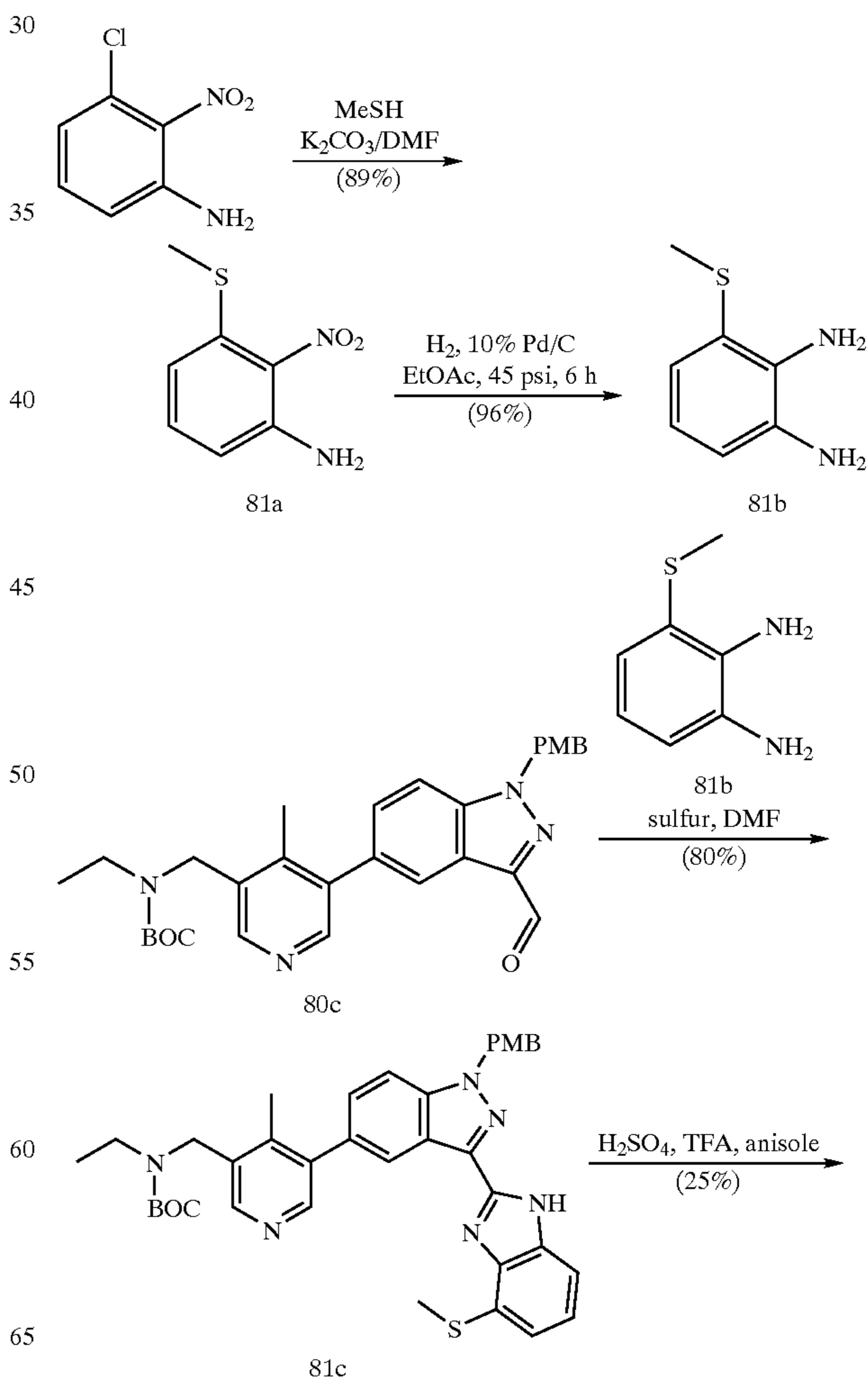
Ethyl-4-{methyl-5-[3-(4-methylsulfanyl-1H-benzimidazol-2-yl)-1H-indazol-5-yl]-pyridin-3-ylmethyl}-amine
