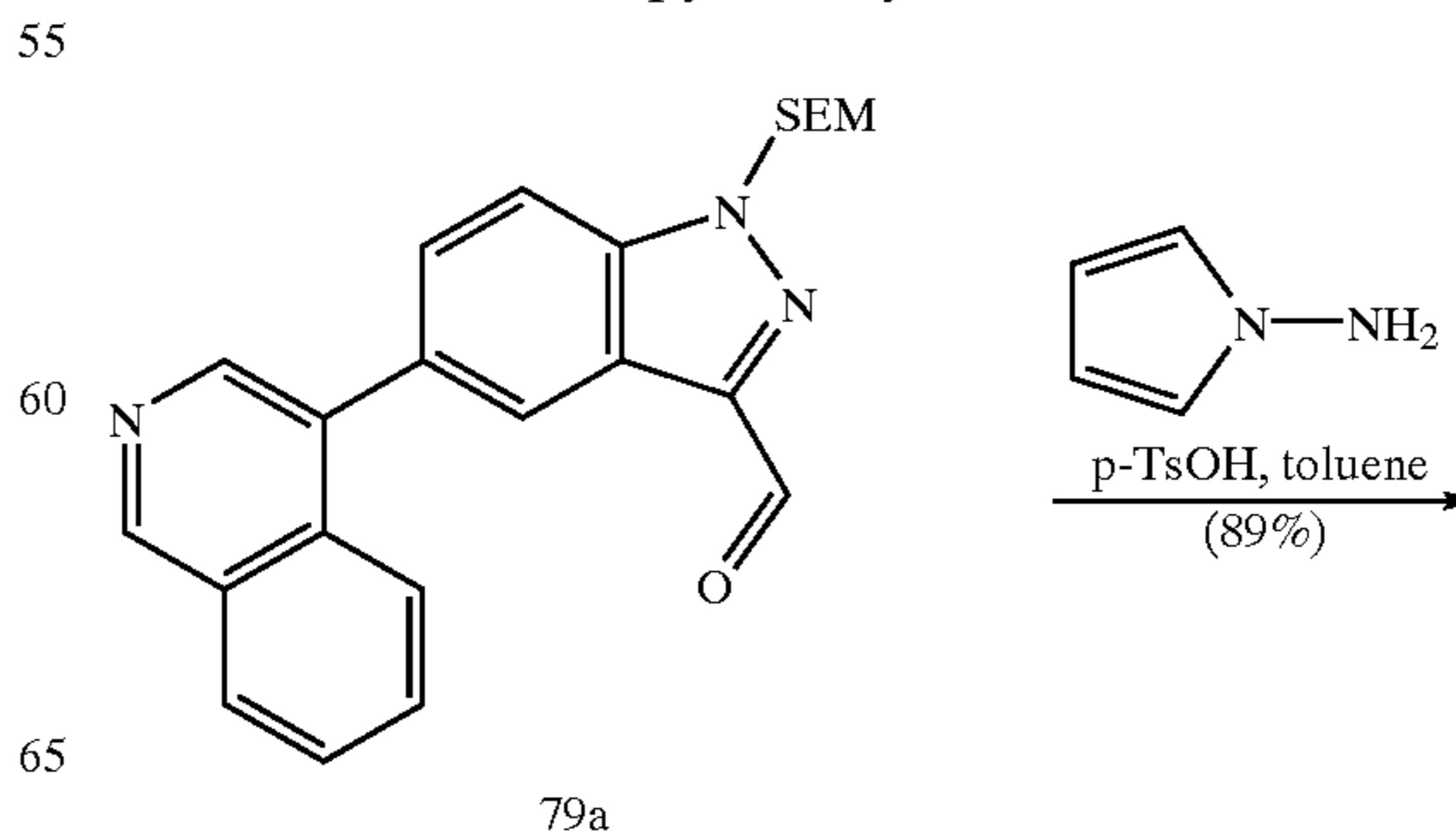
(5-Isoquinolin-4-yl-1H-indazol-3-ylmethylene)-pyrrol-1-yl-amine
