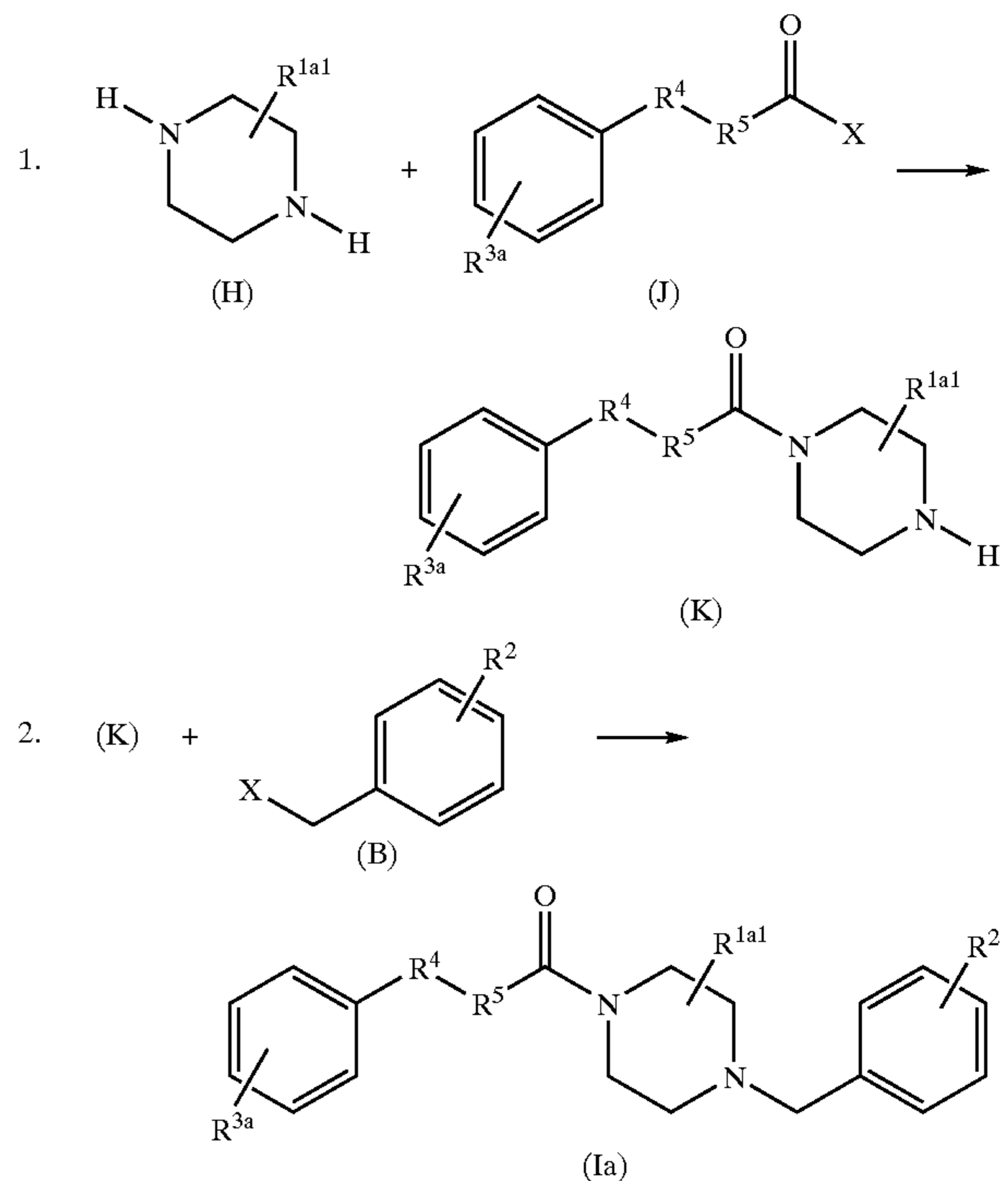
Reaction Scheme 3
