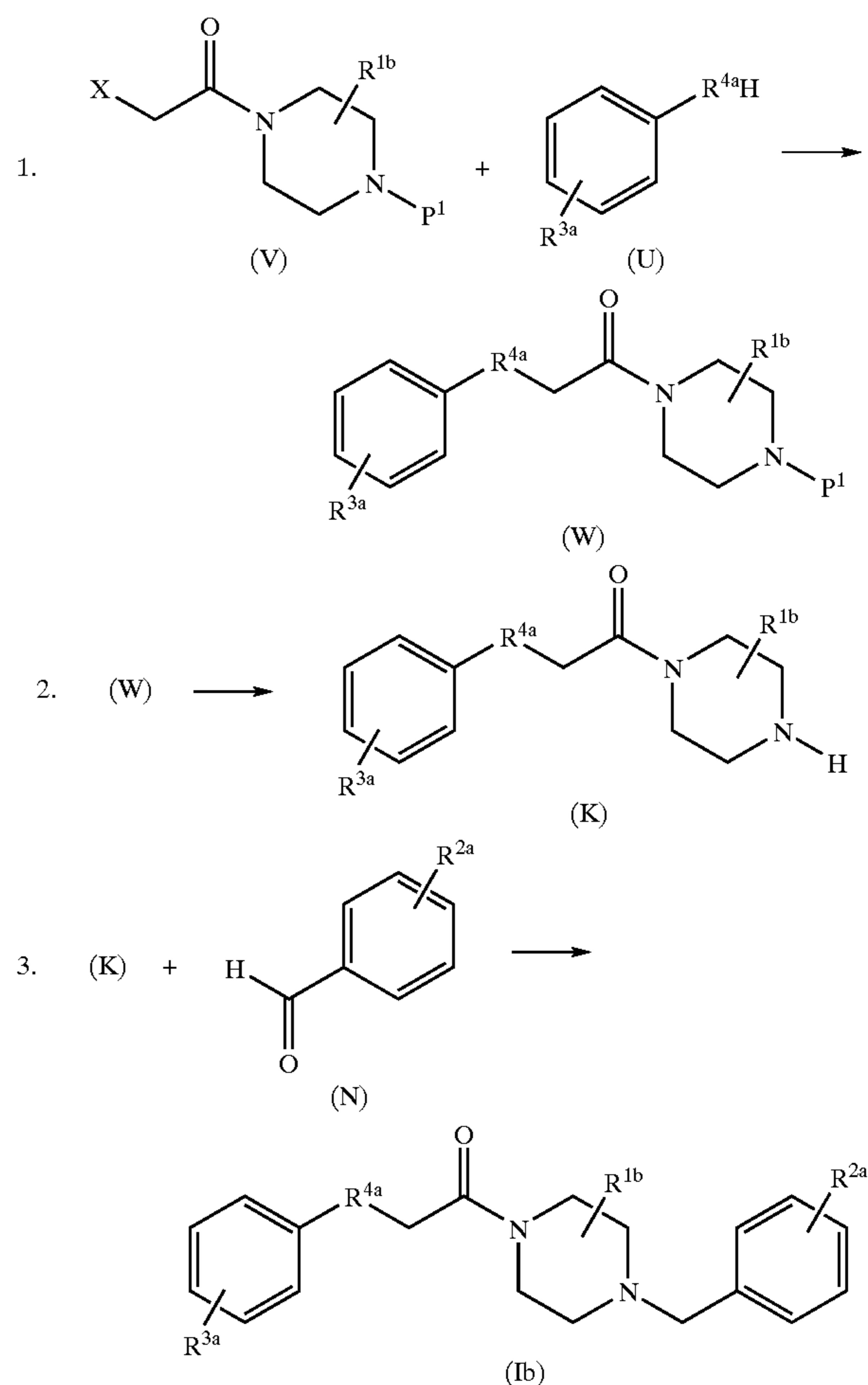
Reaction Scheme 6
