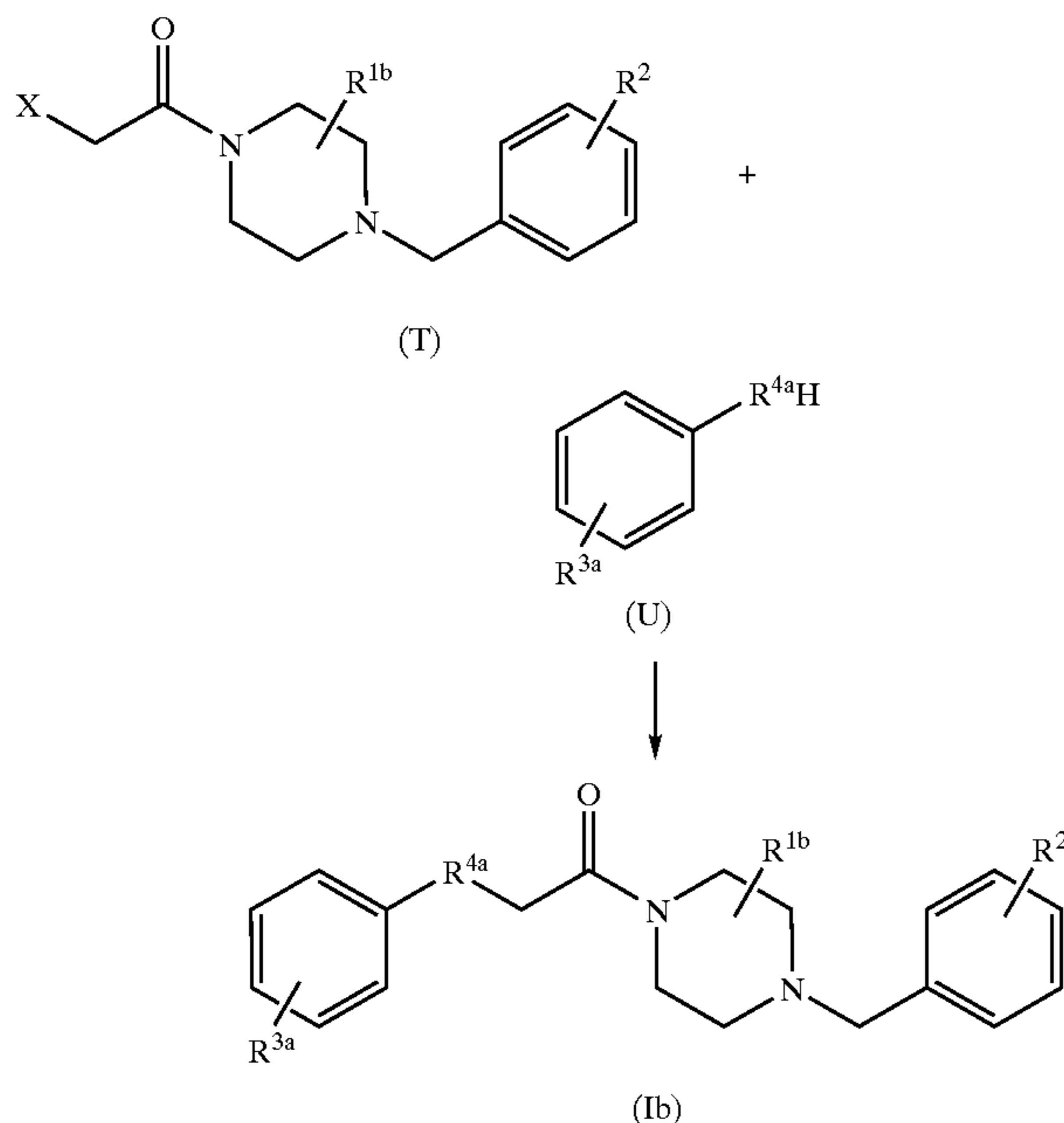
Reaction Scheme 5
