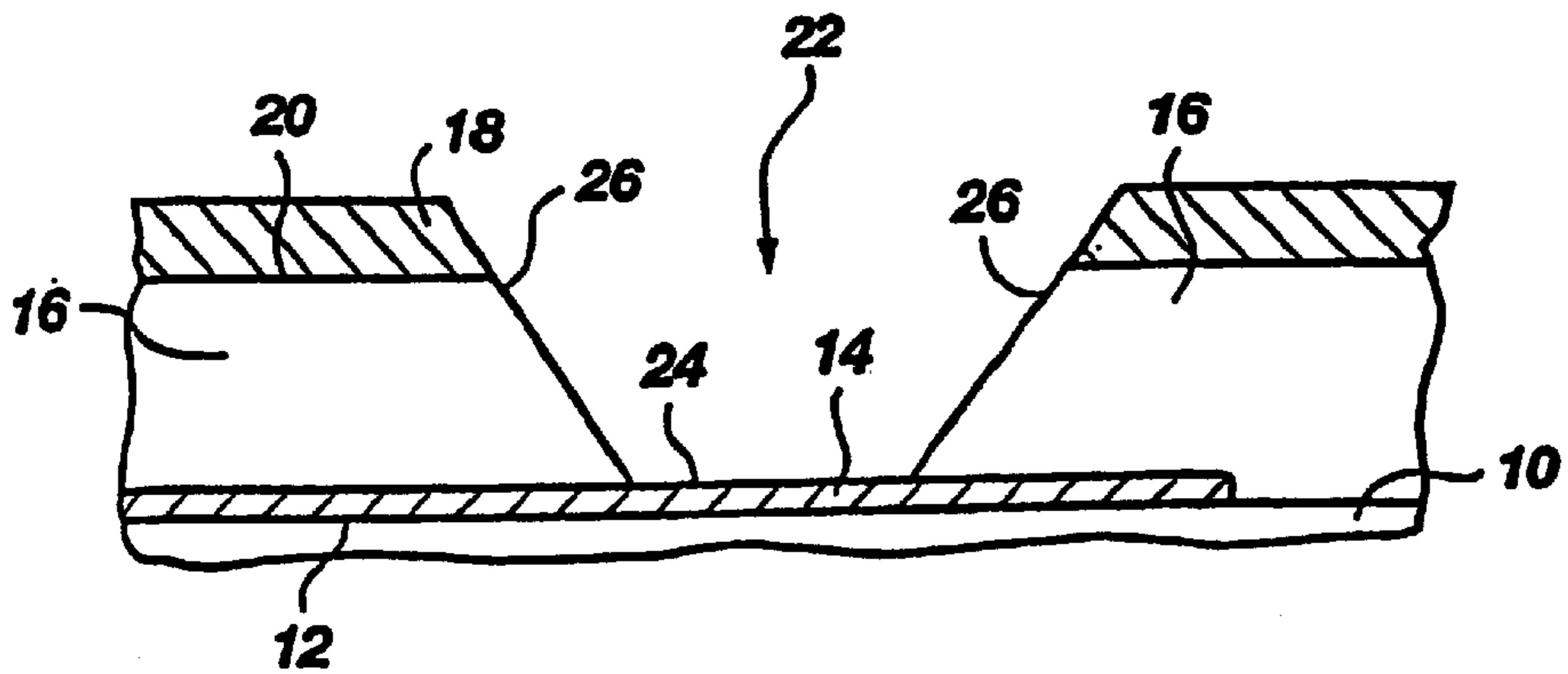
Fig. 1c (PRIOR ART)
