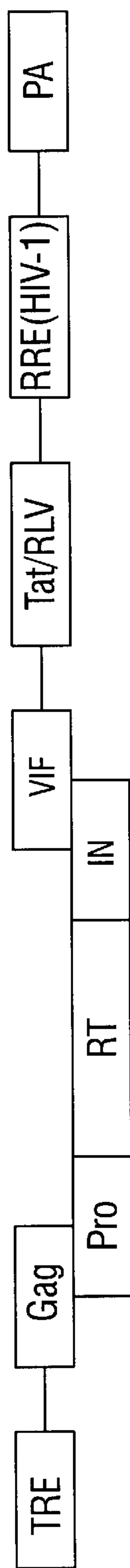
FIG. 23A pTRE, Gag-Pro-RT-IN
