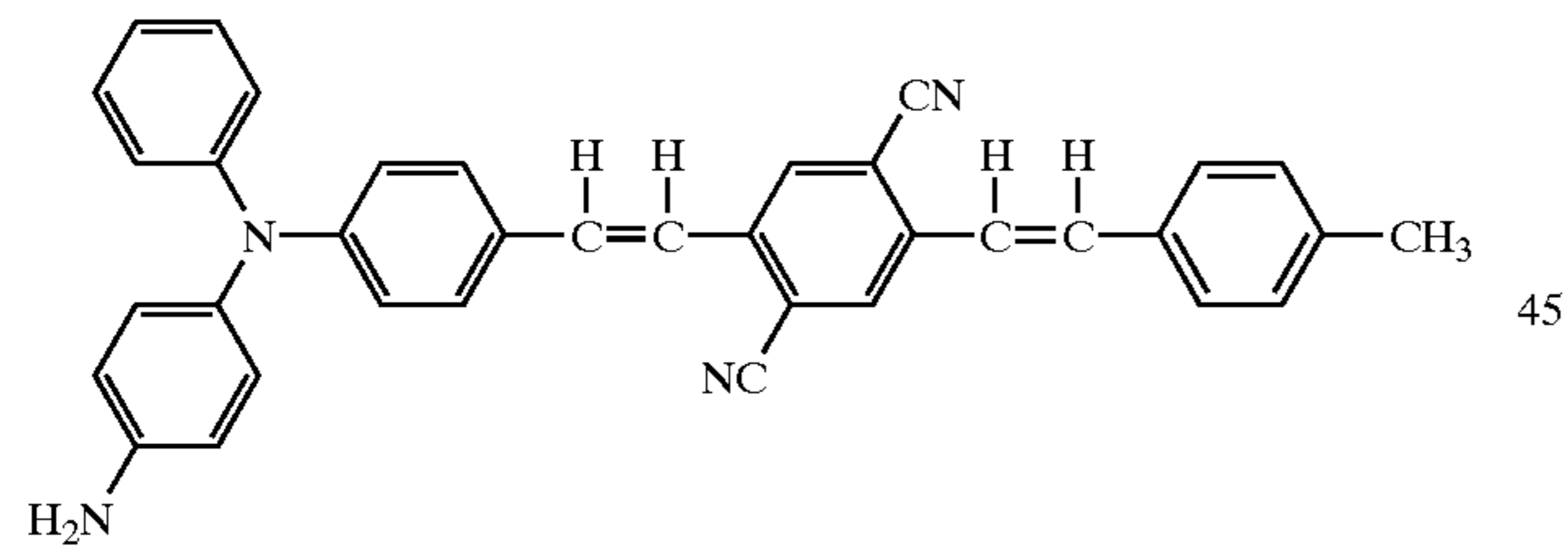
Structural Formula (10)-11
