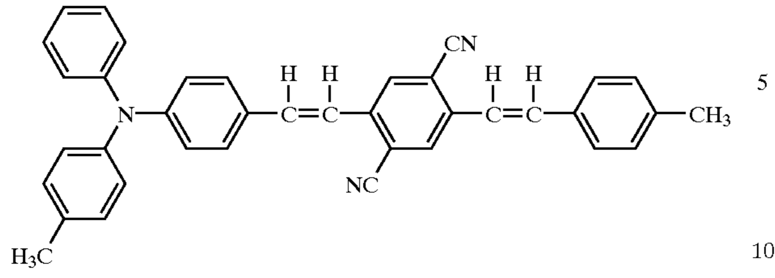
Structural Formula (10)-3
