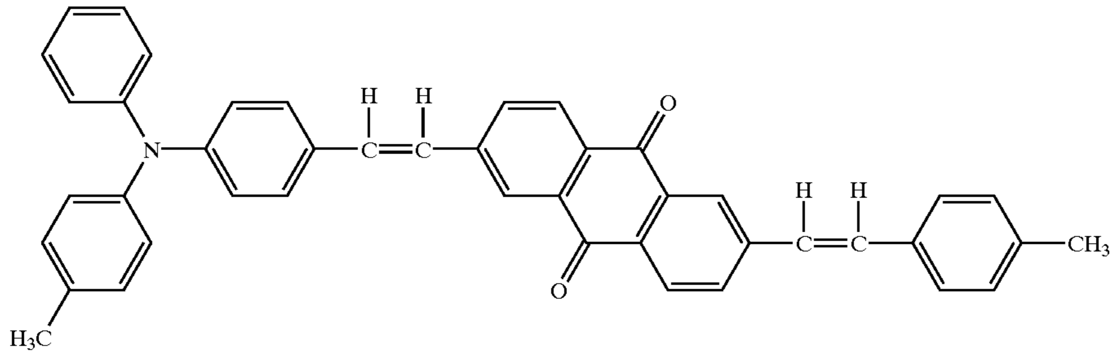
Structural Formula (10)-9
