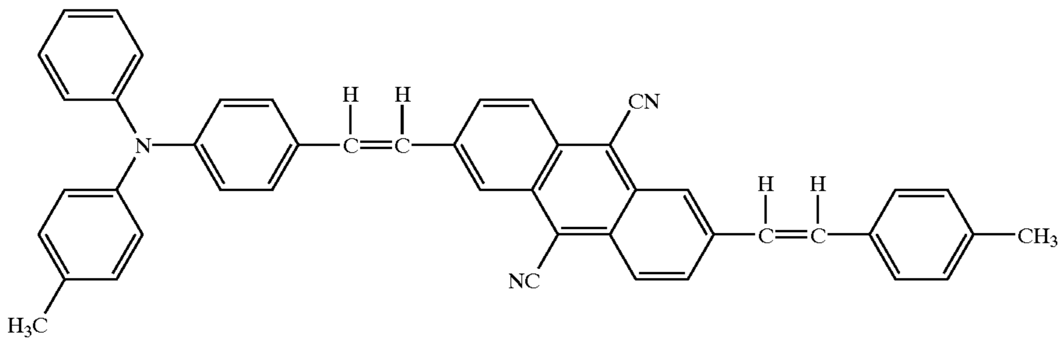
Structural Formula (10)-4
