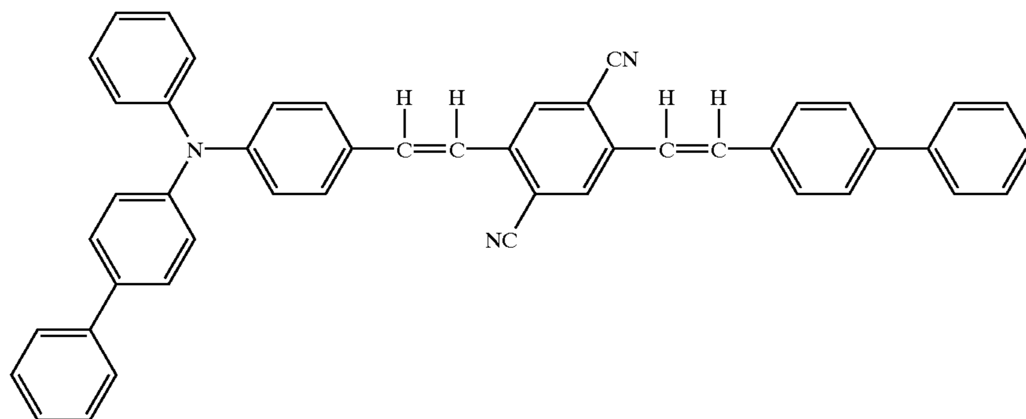
Structural Formula (10)-16
