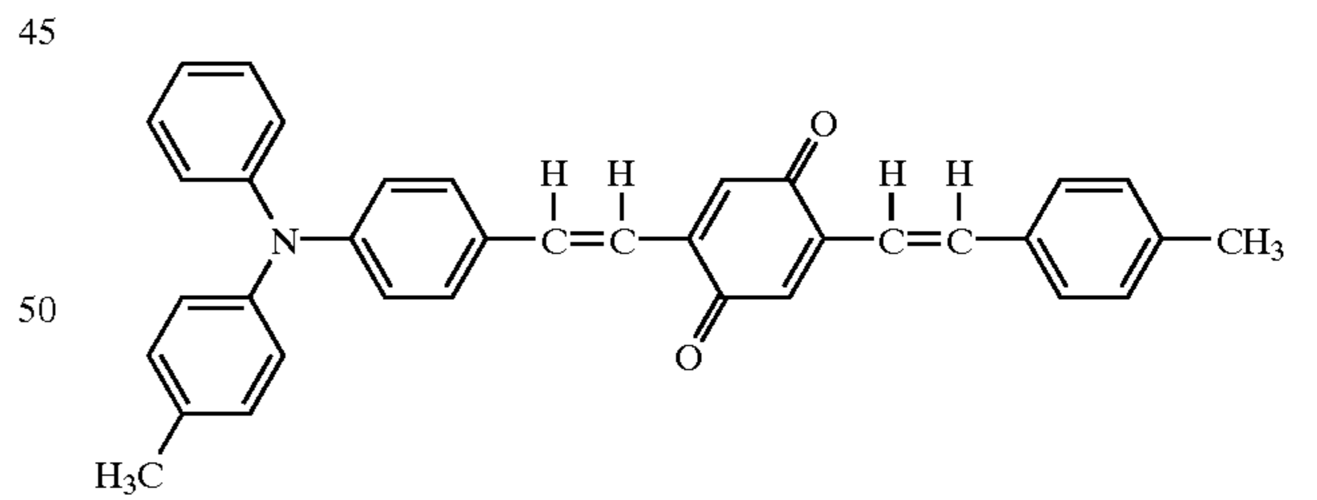
Structural Formula (10)-7
