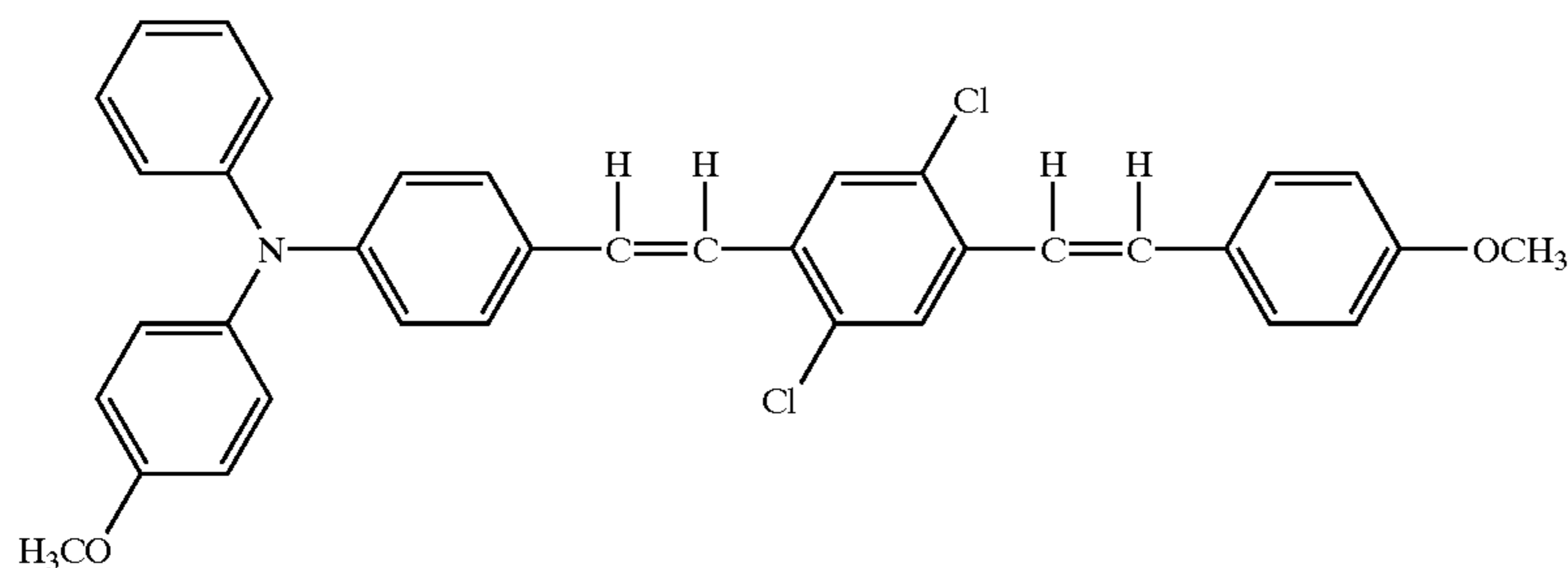
Structural Formula (10)-18
