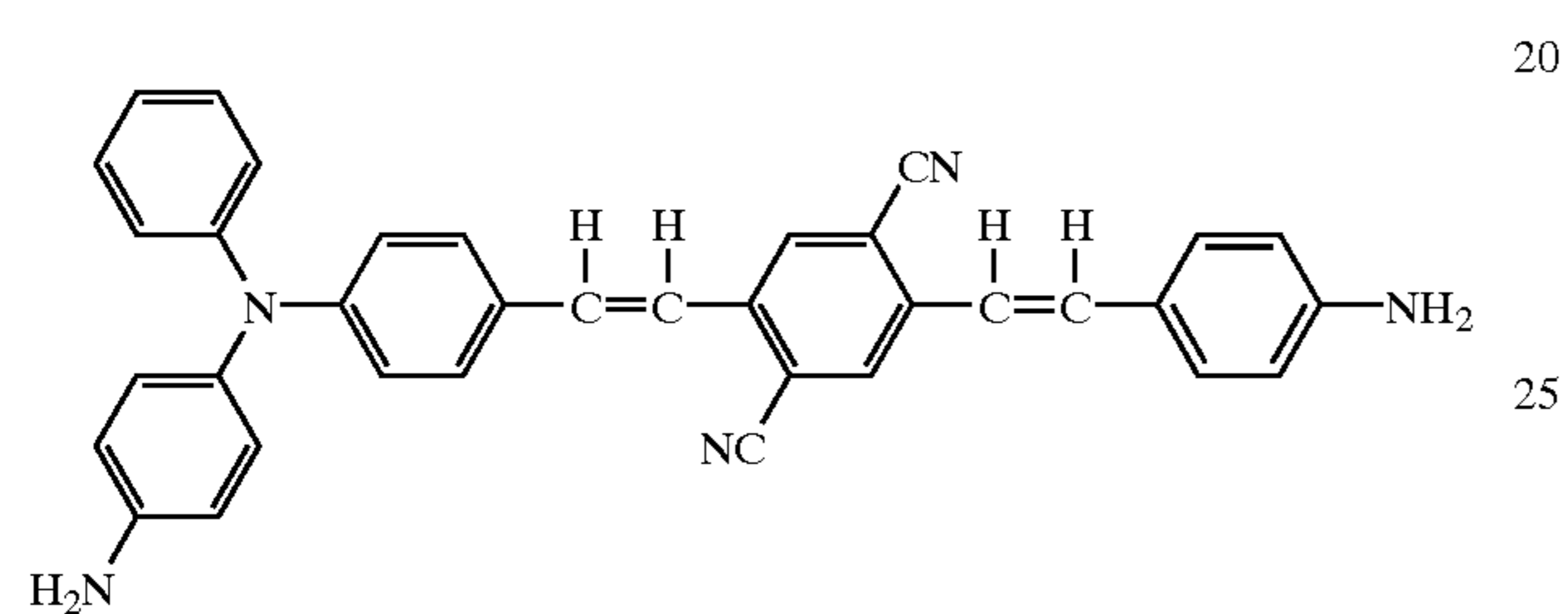
Structural Formula (10)-15
