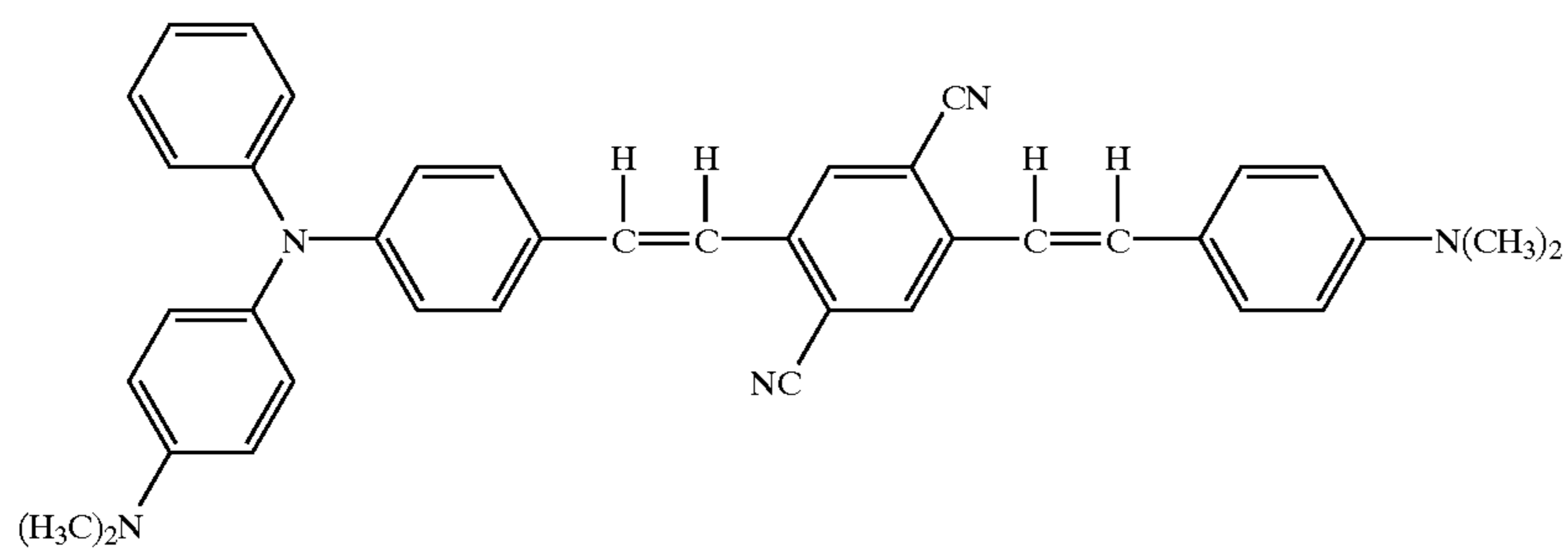
Structural Formula (10)-14
