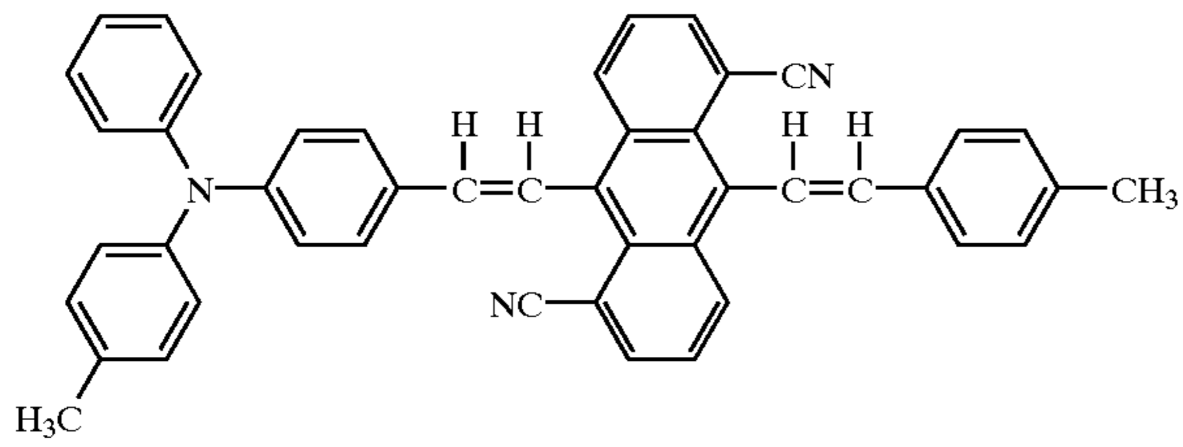
Structural Formula (10)-6
