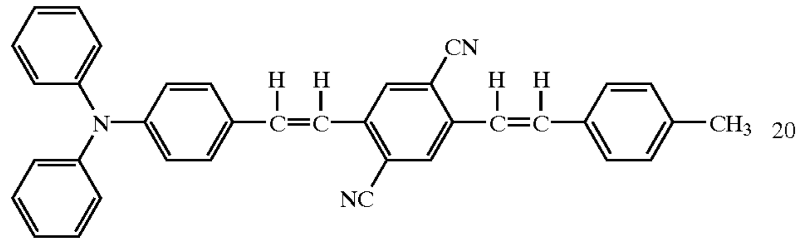
Structural Formula (10)-9
