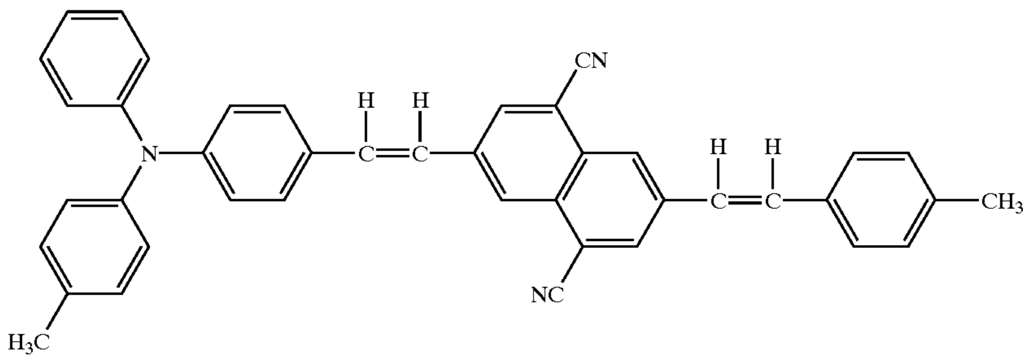
Structural Formula (10)-3
