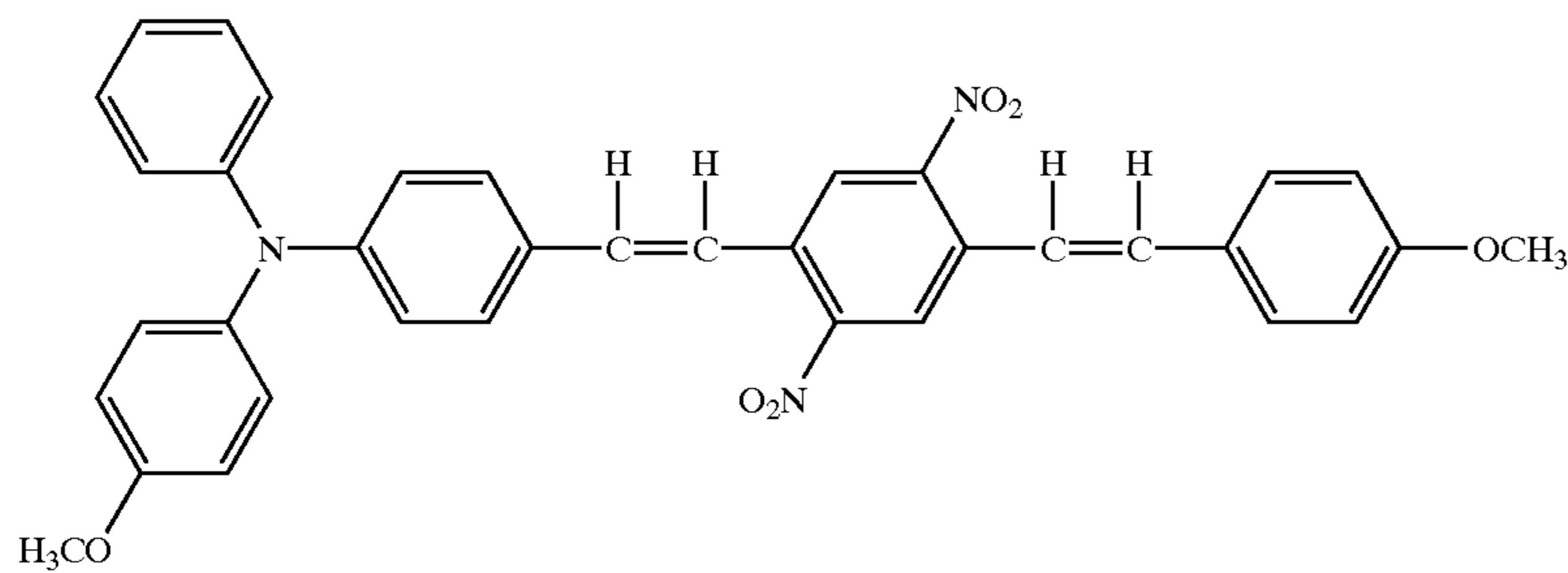
Structural Formula (10)-17
