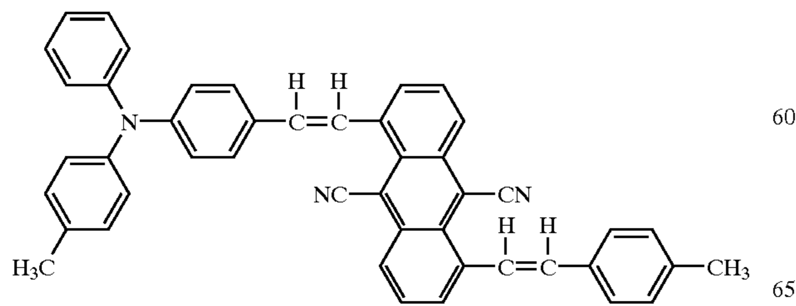
Structural Formula (10)-6
