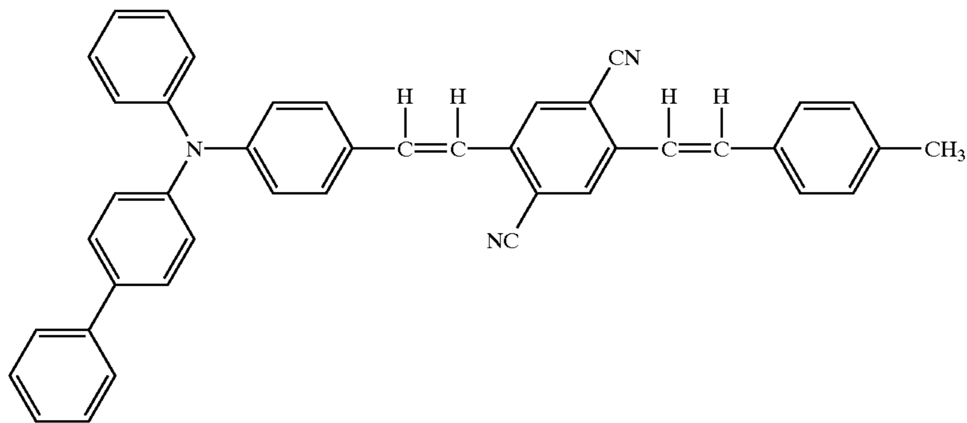
Structural Formula (10)-12
