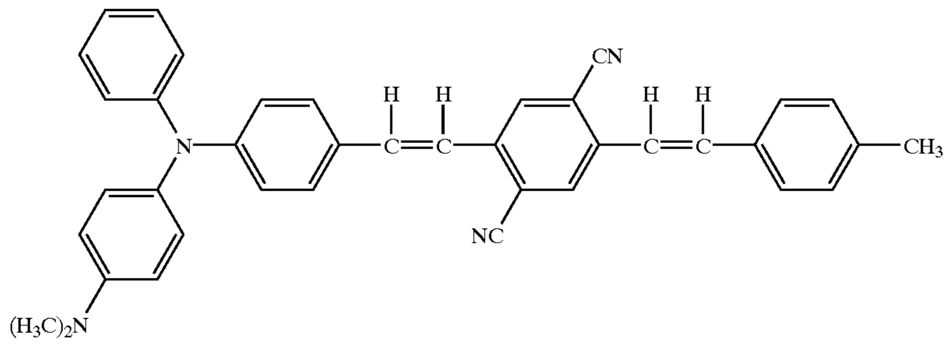
Structural Formula (10)-11
