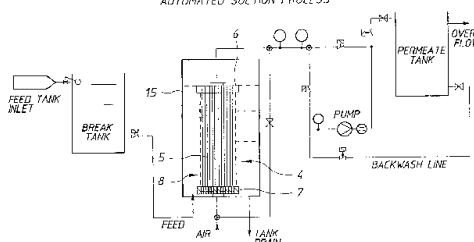
AUTOMATED SUCTION PROCESS
