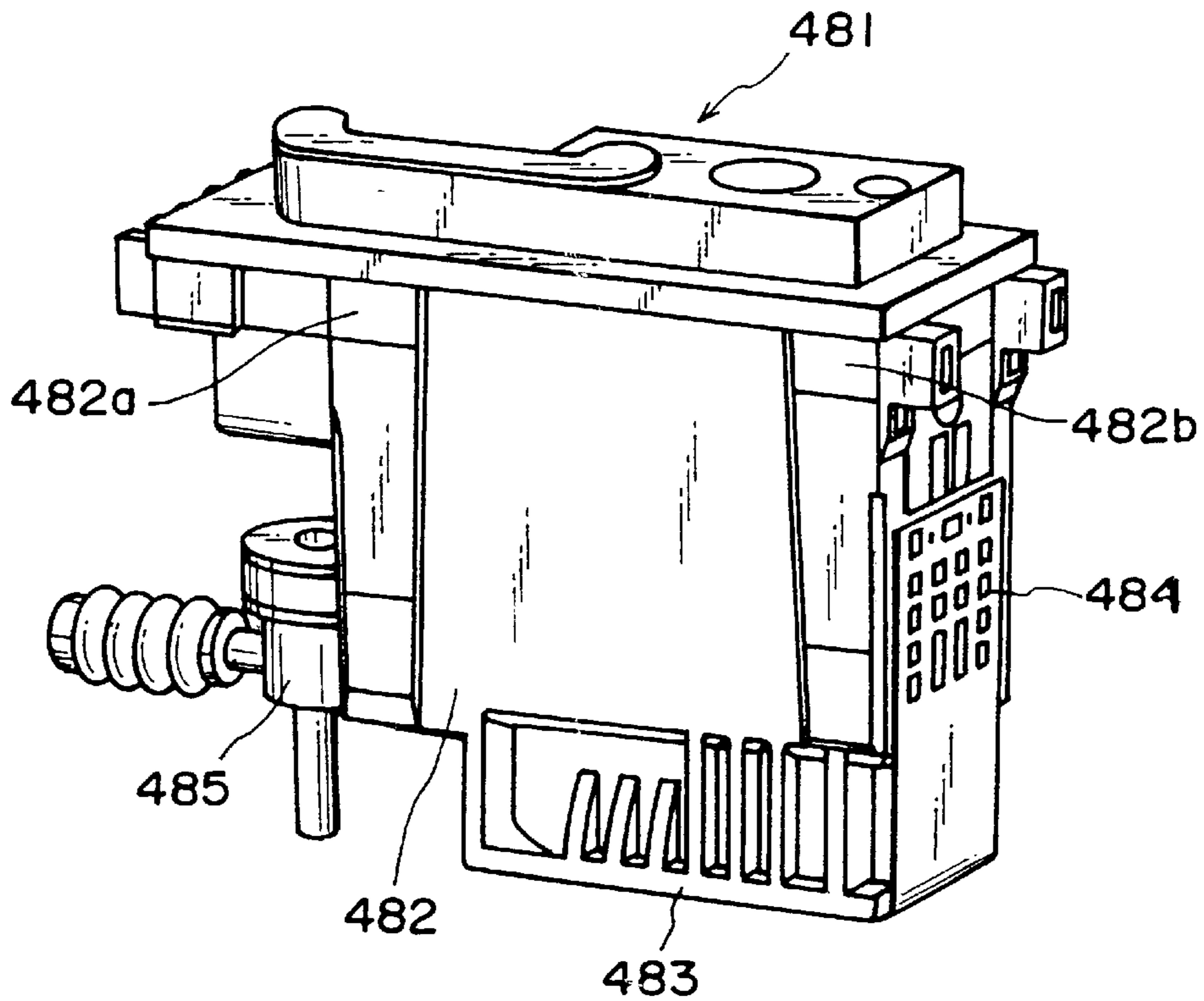
FIG. 76 PRIOR ART
