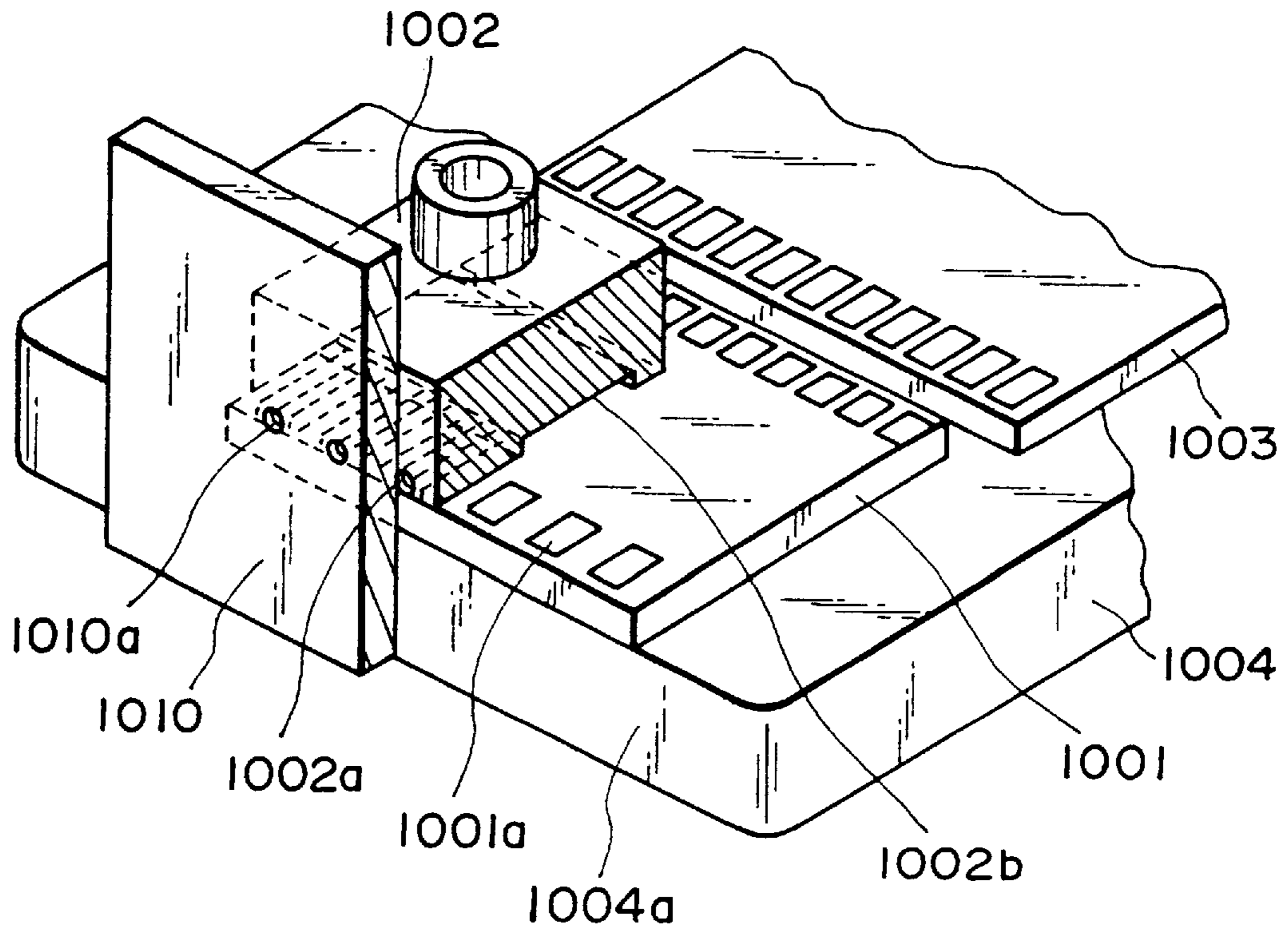
FIG. 73 PRIOR ART
