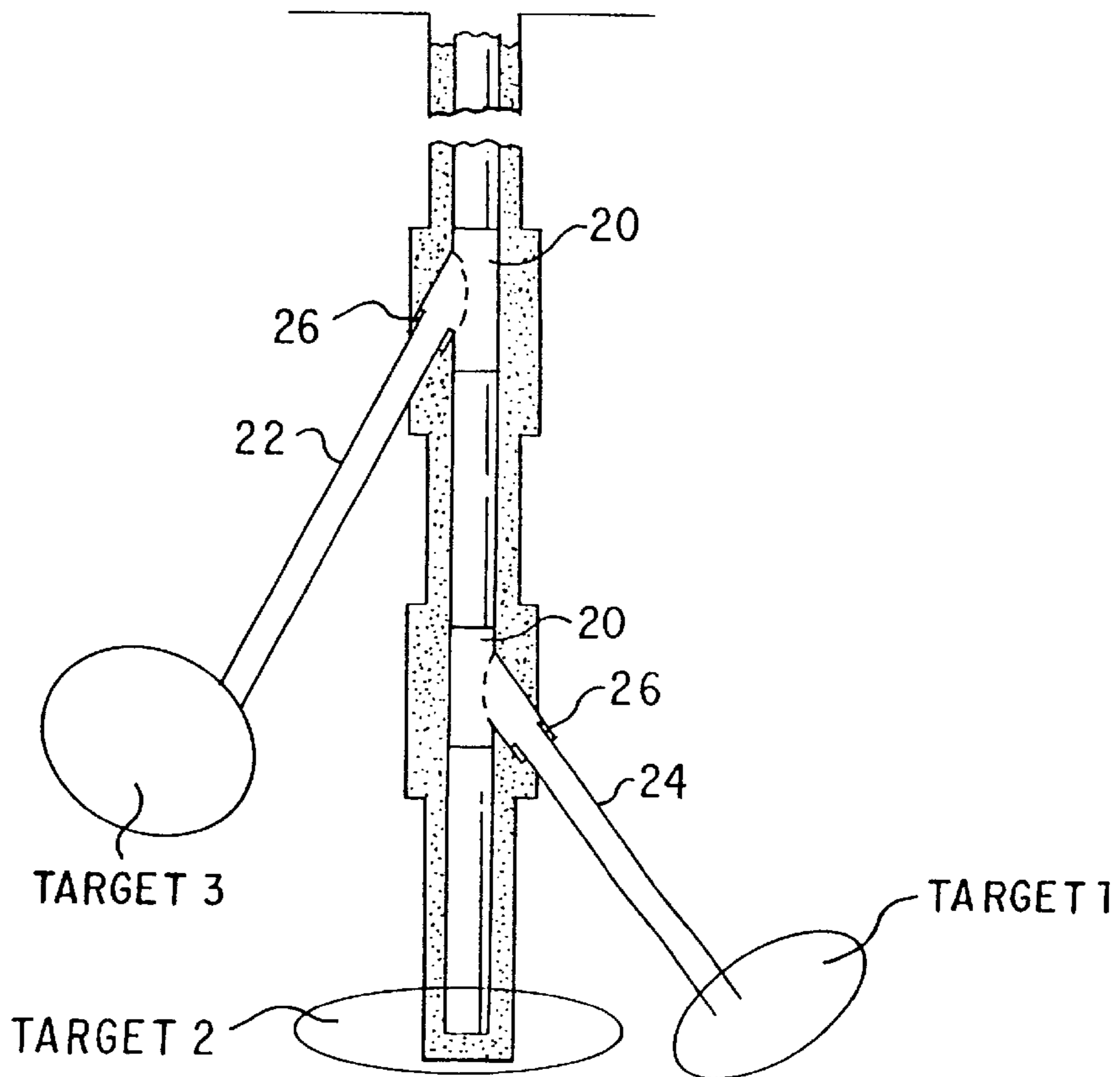
FIG. 2 PRIOR ART
