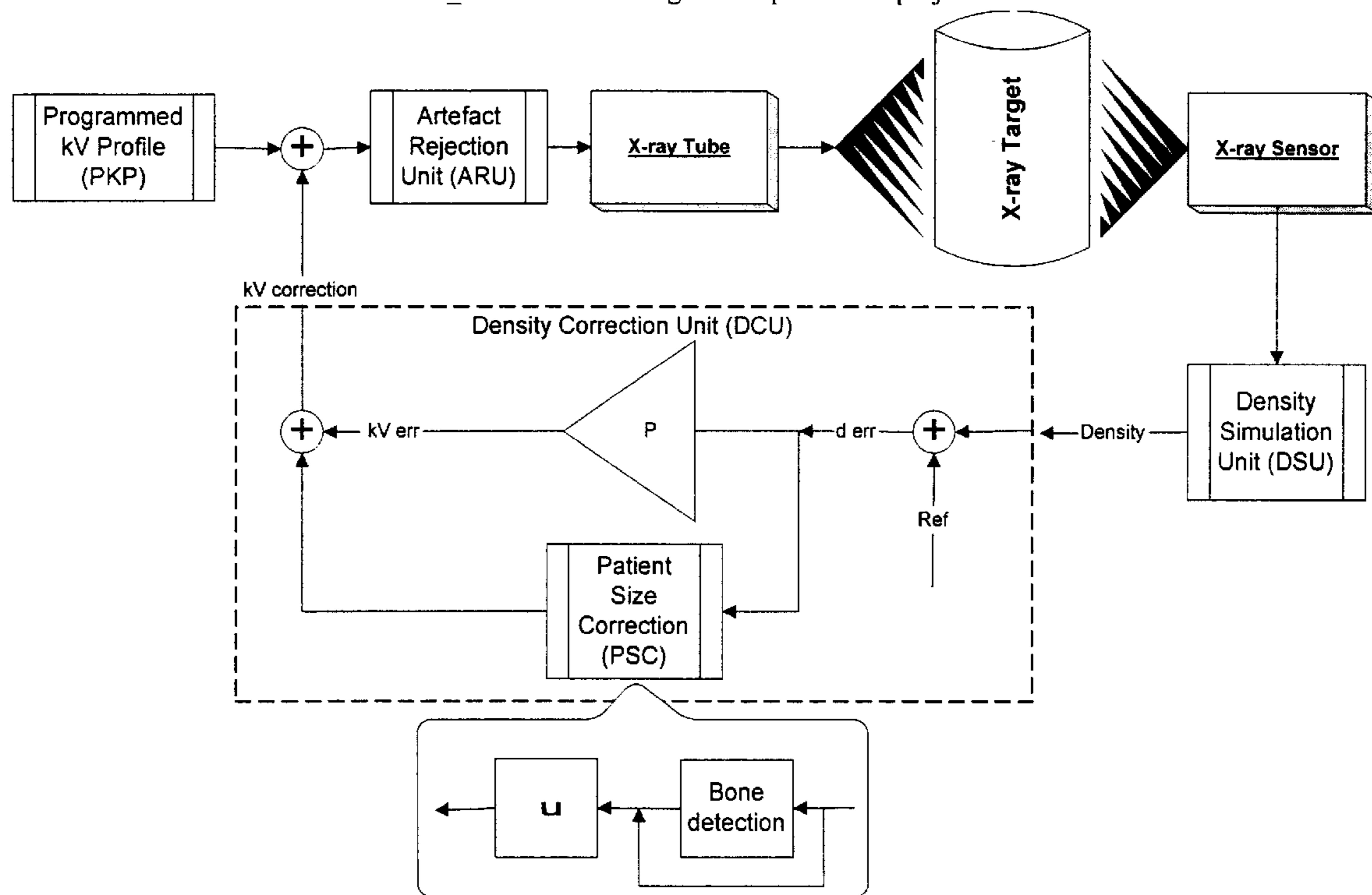
FIG_2a: AEC block diagram for panoramic projections
