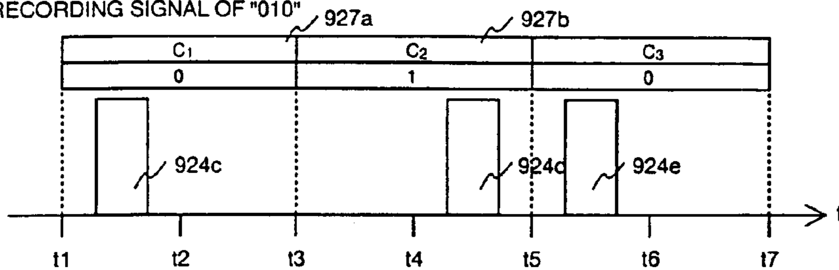
(4) RECORDING SIGNAL OF "010"
