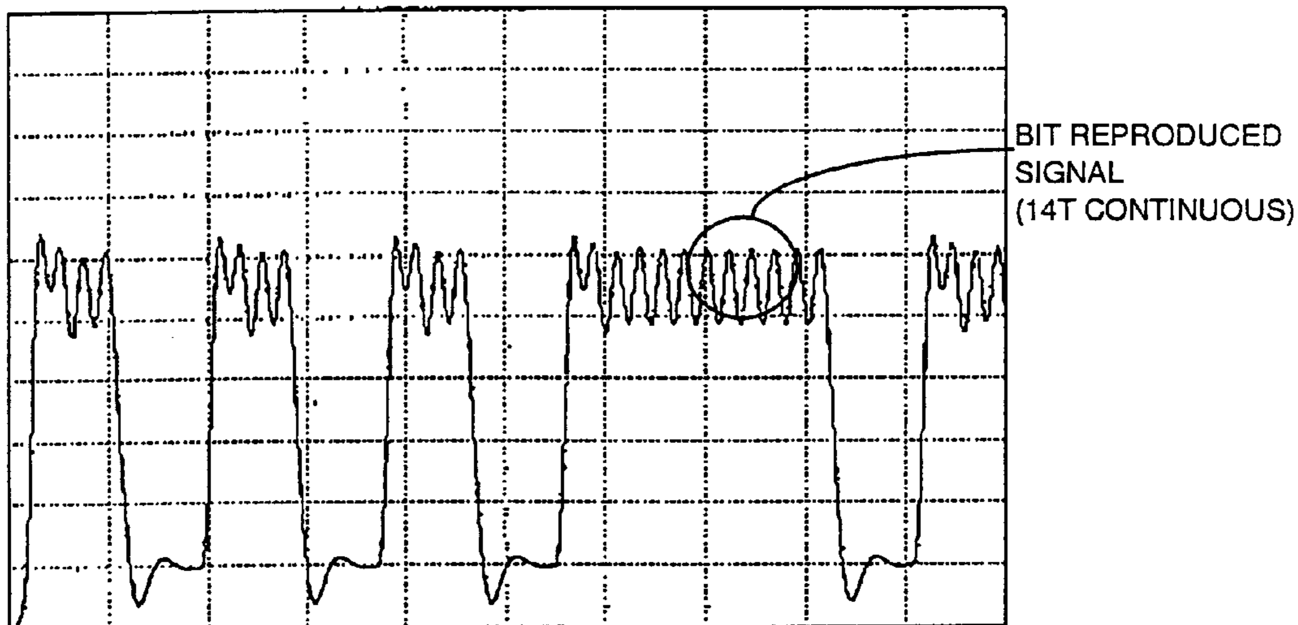
(b) SIMULATOR WAVEFORM AFTER LPF : I 14L = I S = 0.1
