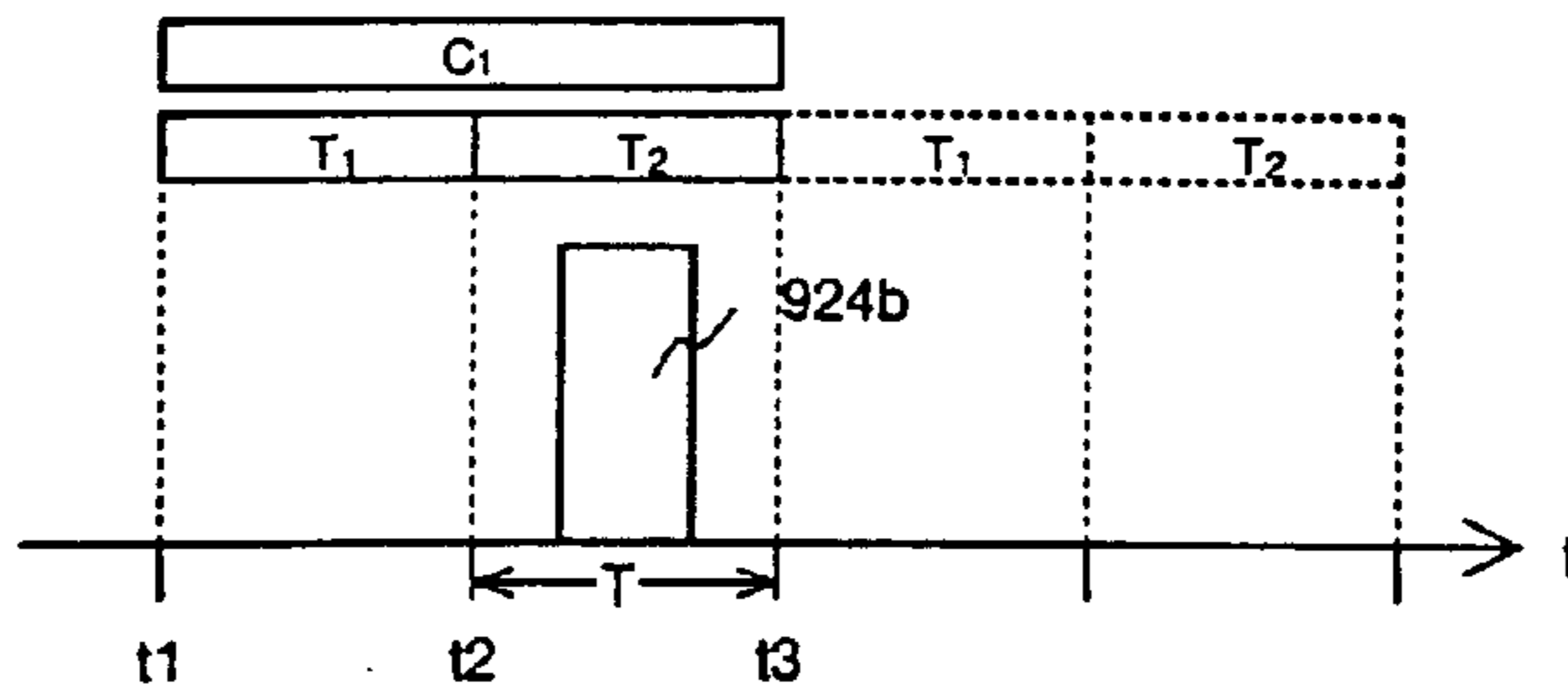
(4) TRIMMING PATTERN OF "1"
