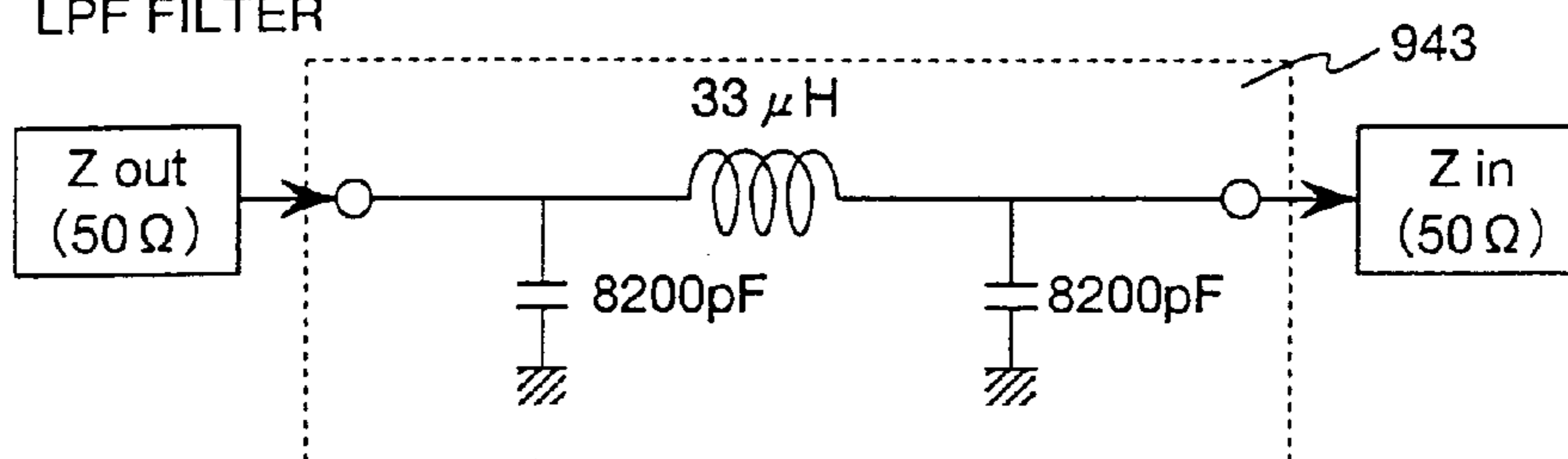
(a) LPF FILTER
