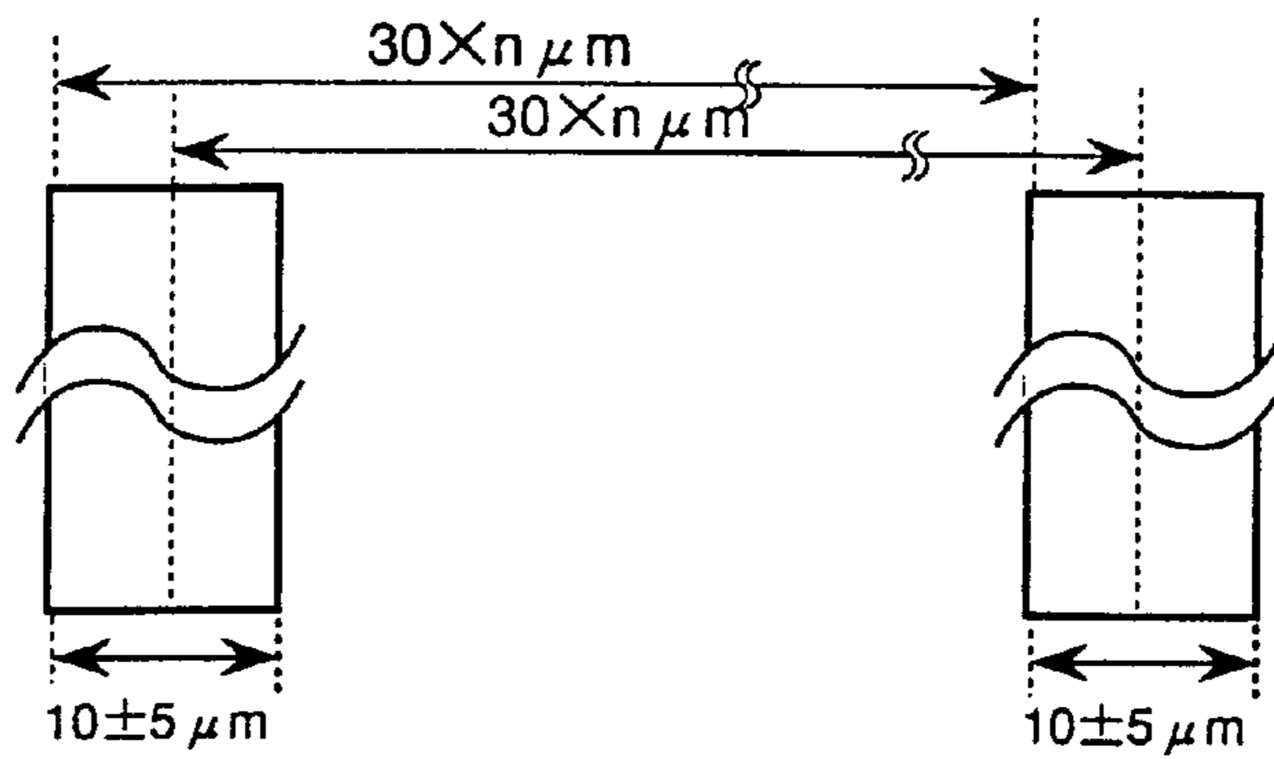
(b) DIMENSIONAL ACCURACY OF SLIT ( at r=22.2mm )
