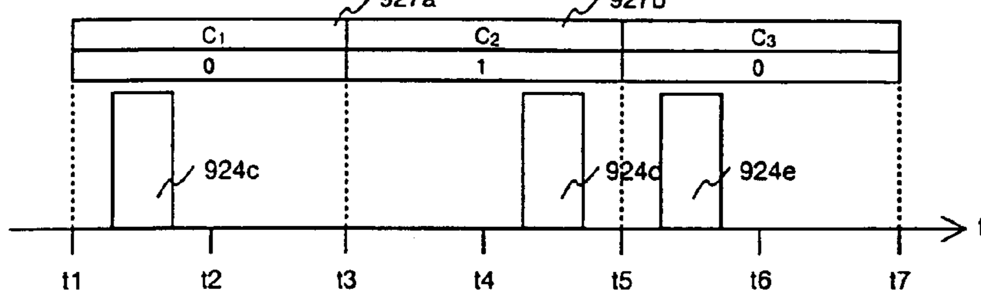
(4) RECORDING SIGNAL OF "010"
