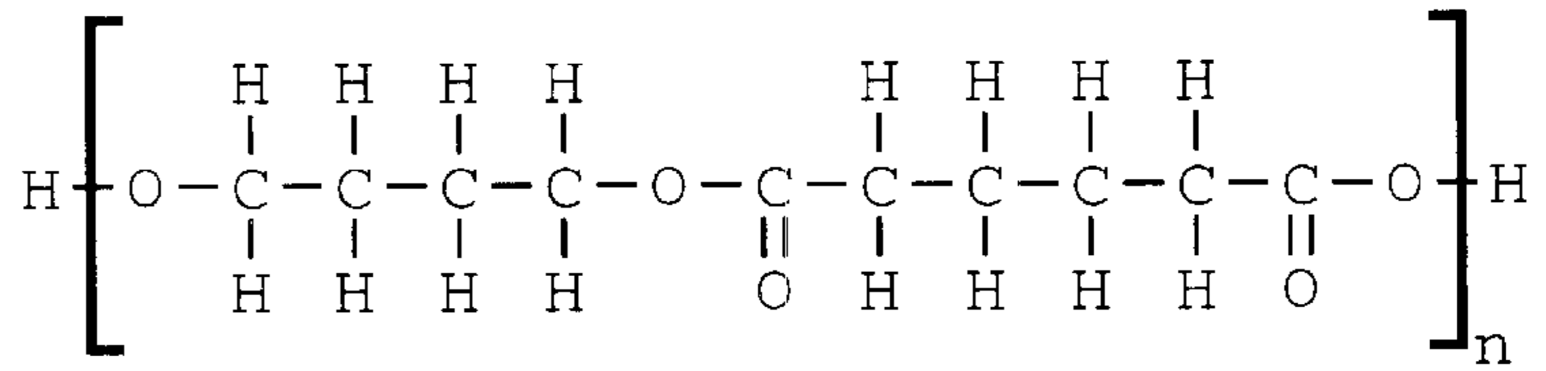
poly(buthyleneglycol adipinat)
