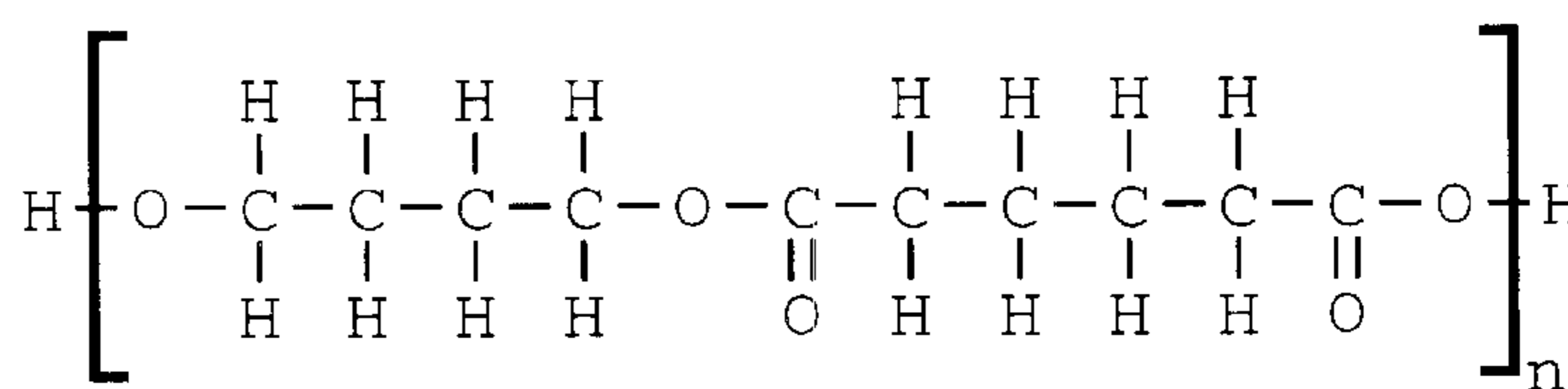
poly(buthyleneglycol adipinat)
