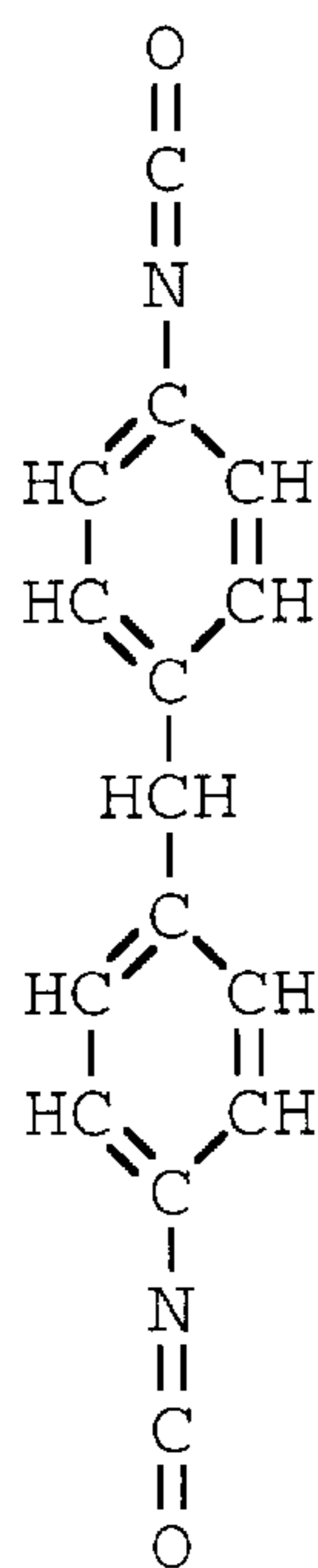
4,4'-methylene- biphenyl isocyanate
