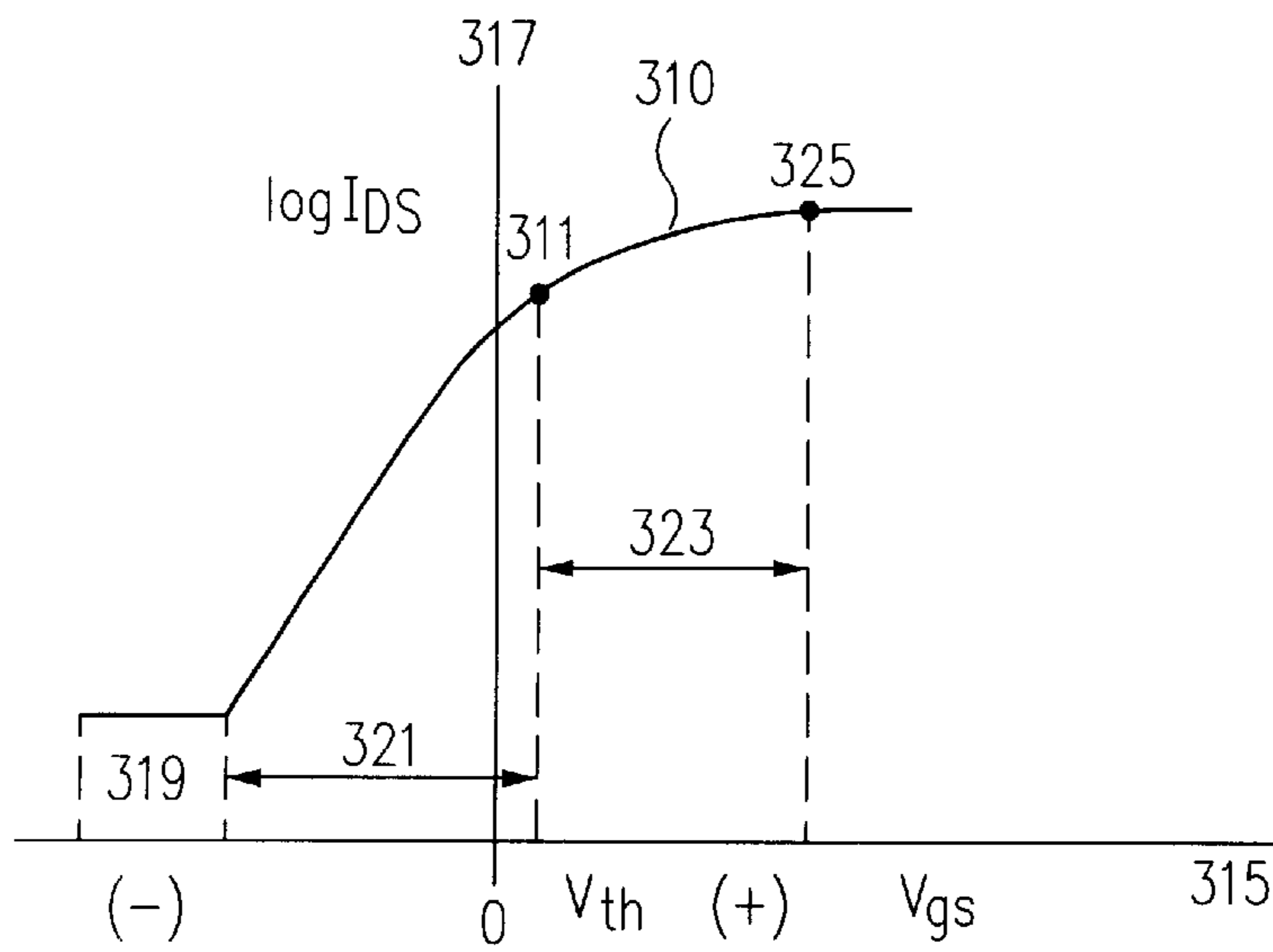
FIG. 3 (PRIOR ART)
