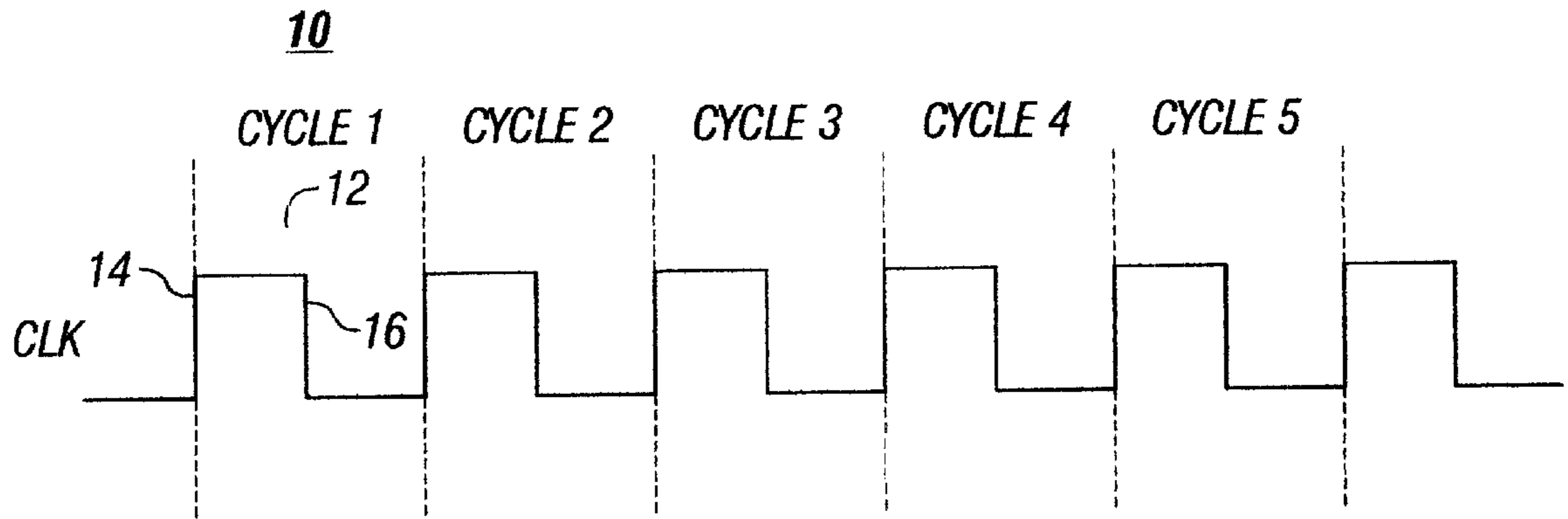
FIG. 1 (Prior Art)
