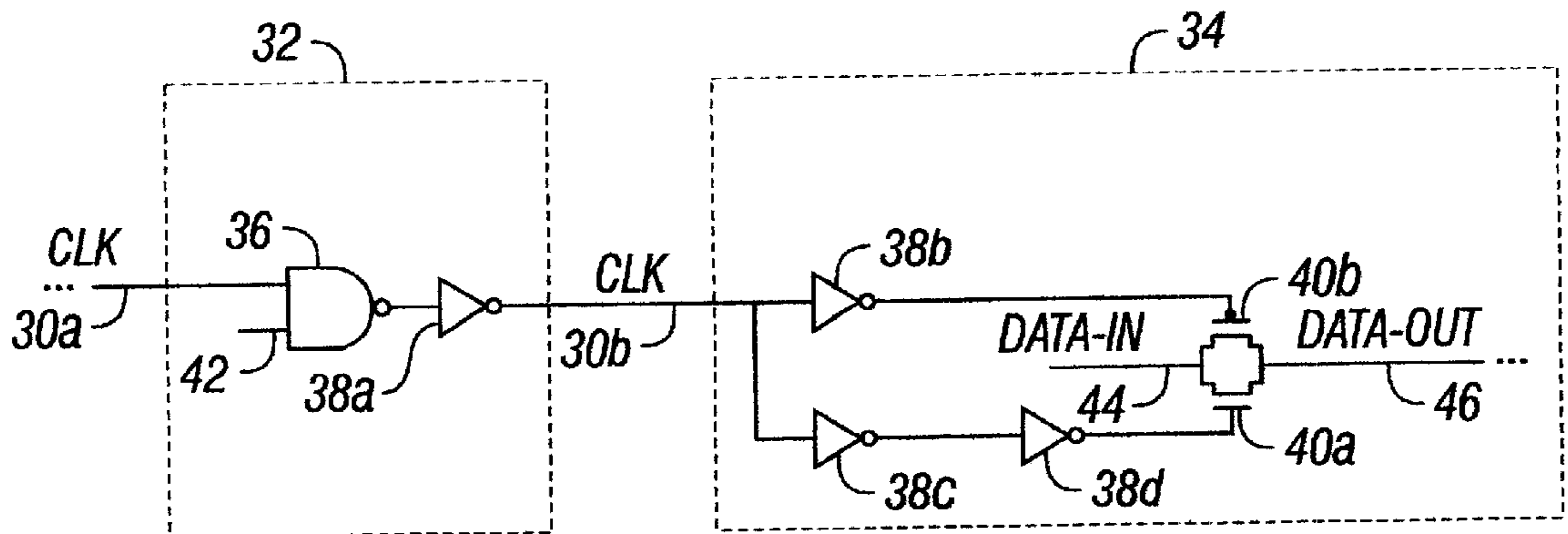
FIG. 3 (Prior Art)
